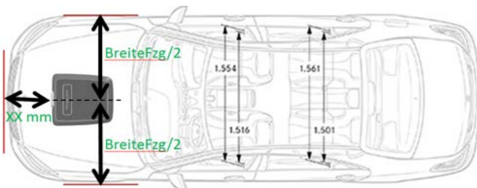
Figure 13 Example for positioning the GPM with desired forward parking
