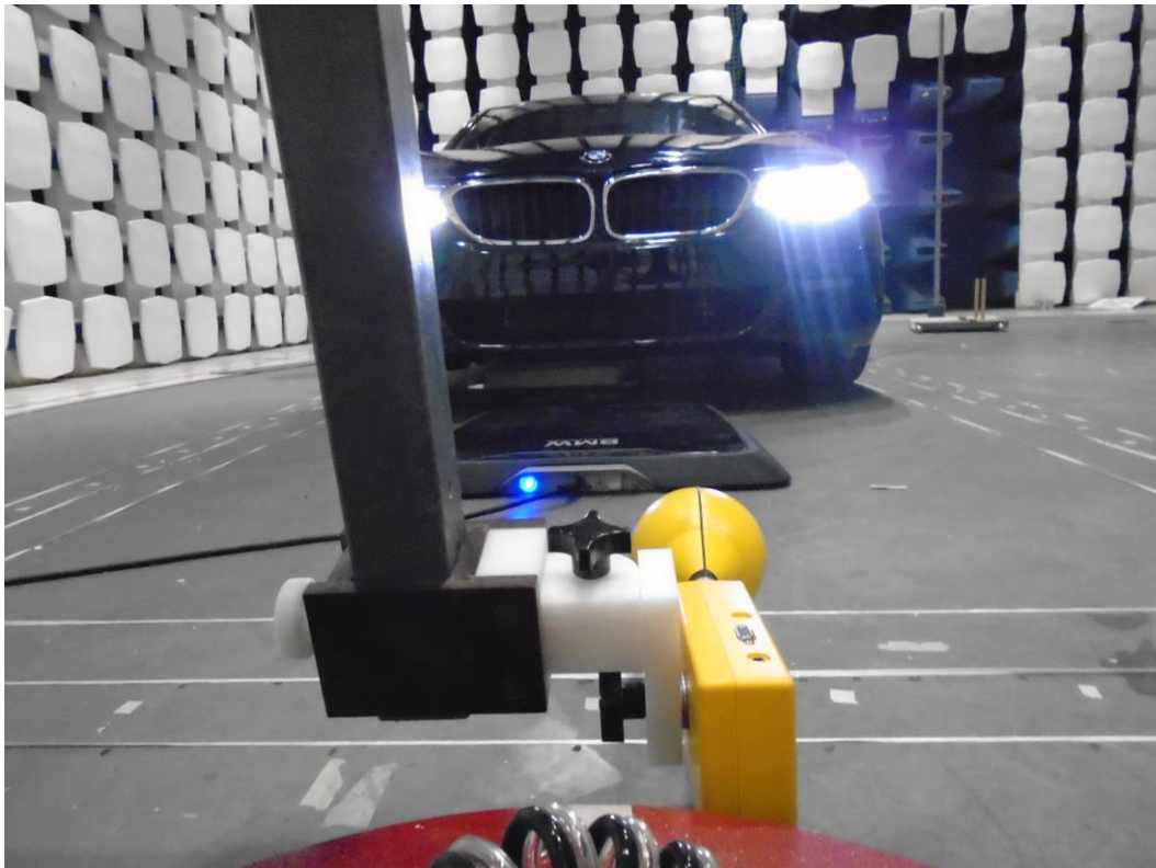
Figure 12 – General Setup of EUT
