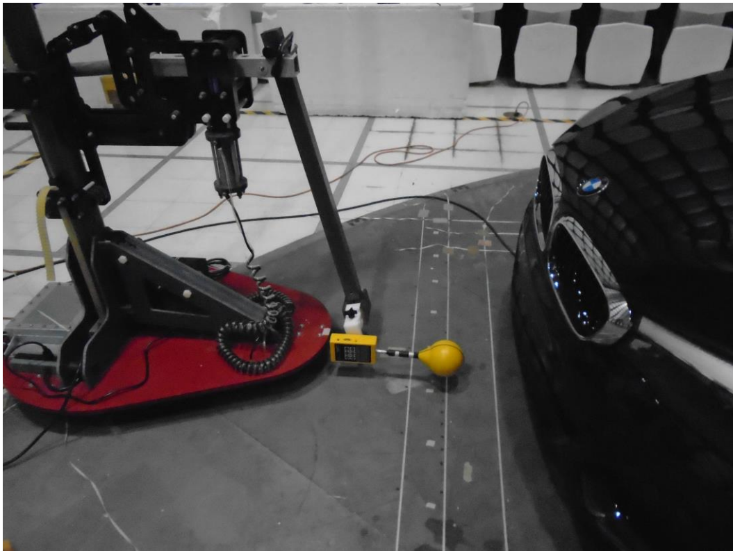
Figure 13 – Position 2 Setup
