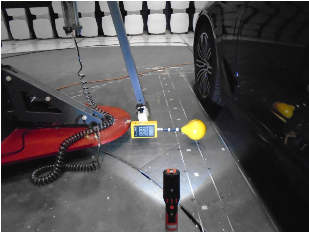
Figure 14 – Position 3 Setup
