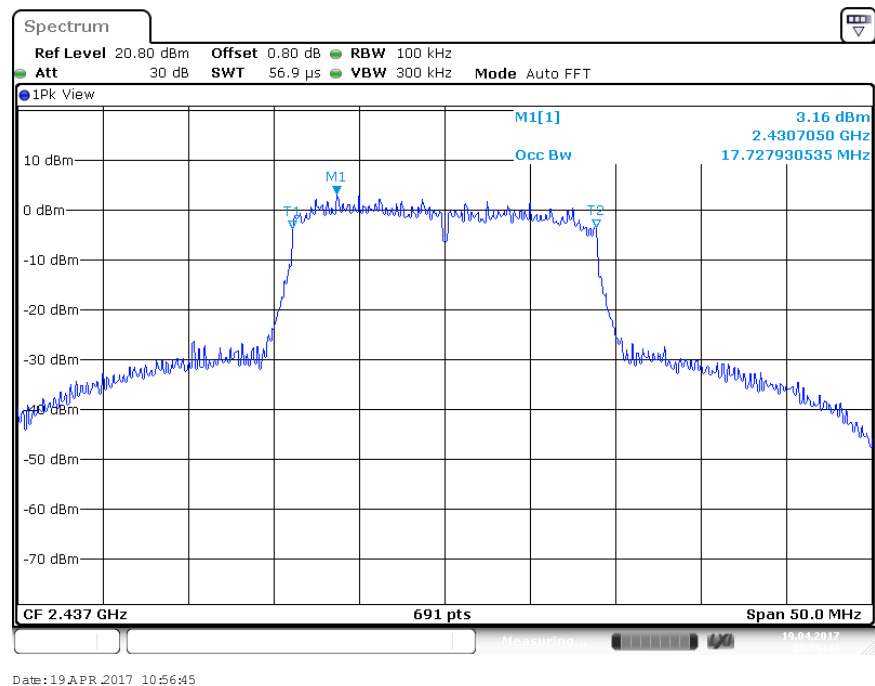
Figure 9: 99% Occupied Bandwidth, 2437 MHz at HT20 MCS7
