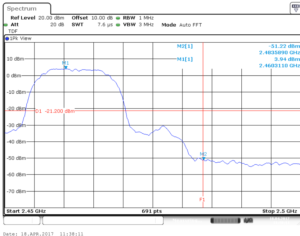
Figure 39: Radiated Emission at 2483.5 MHz Edge for 2462 MHz-802.11b- Vert. (Pk)
