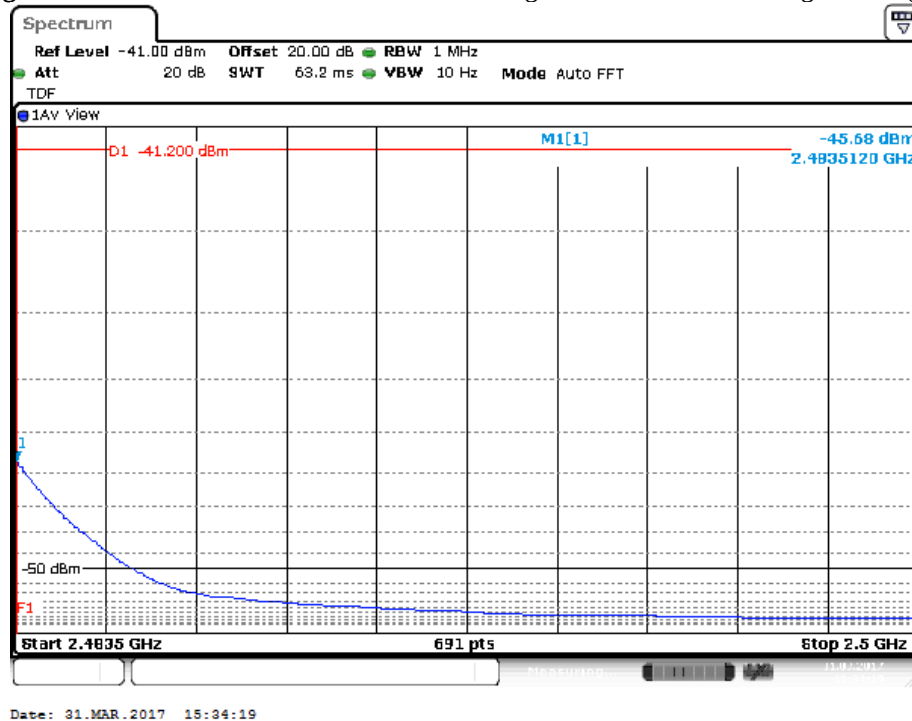
Figure 32: Radiated Emission at 2483.5 MHz Edge for 2462 MHz-802.11g – Vert. (Ave)
