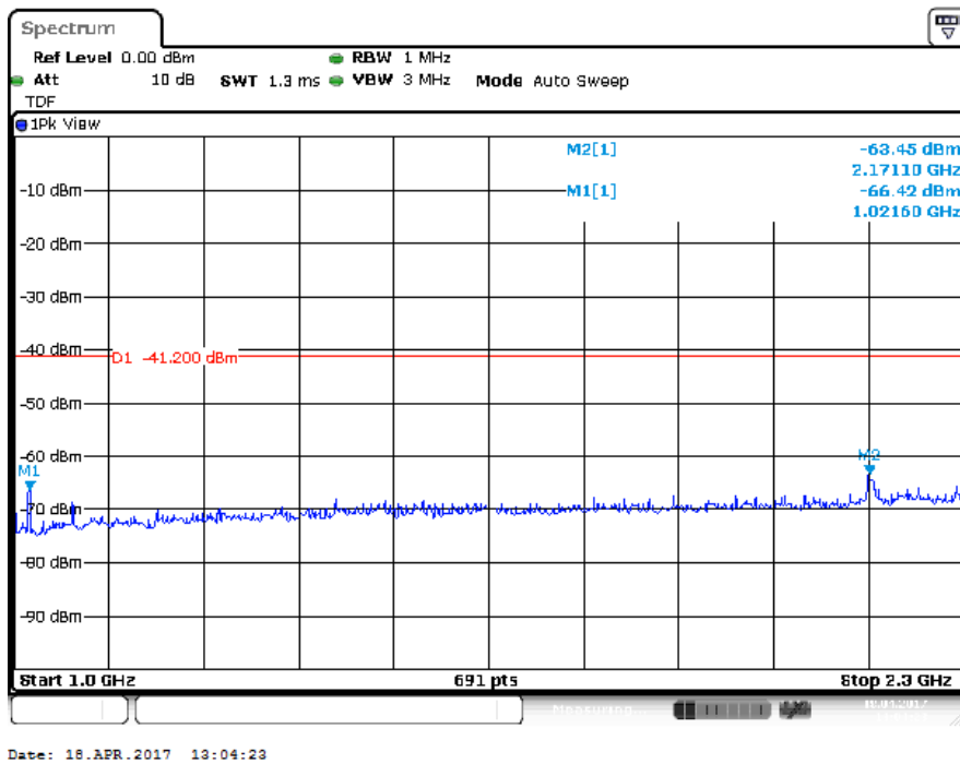
Plot of the emissions (peak values shown) in the range 1-2.3 GHz, 802.11b 1Mbps, EUT V Ant H
