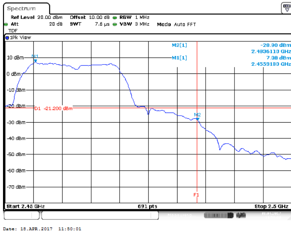
Figure 43: Radiated Emission at 2483.5 MHz Edge for 2462 MHz-802.11g- Vert (Pk)
