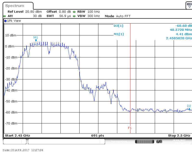
Figure 15: Measured Bandedge for 802.11b-1Mbps at 2462 MHz
