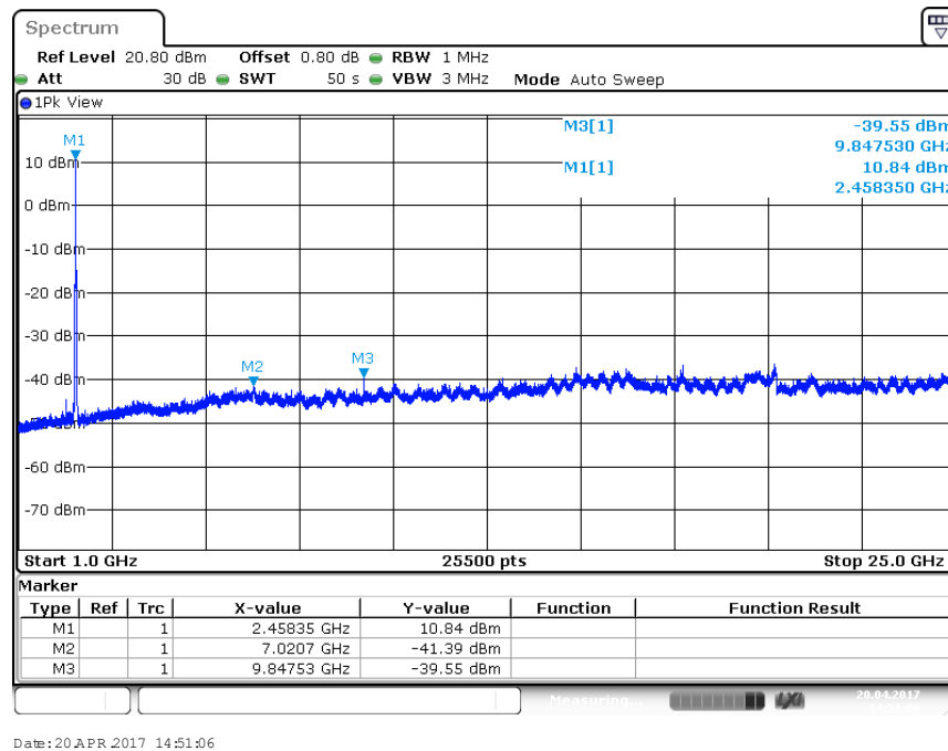
Figure 20: Out of Band Emissions for 802.11g-6Mbps at 2462 MHz
