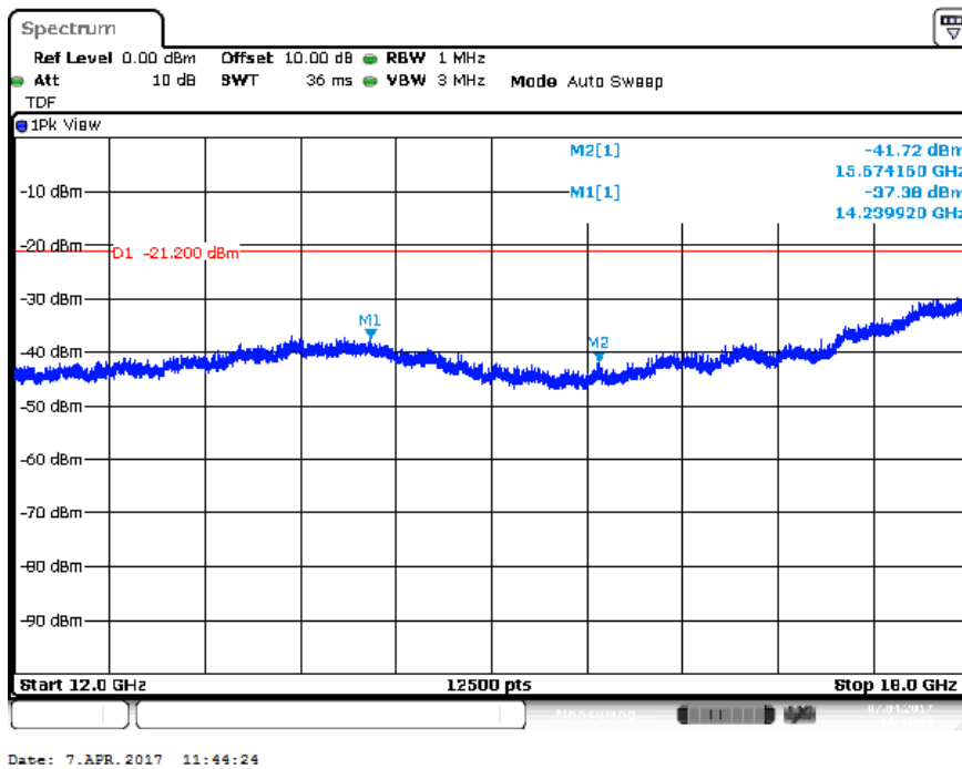
Plot of the emissions (peak values shown) in the range 12 -18 GHz, 802.11n mcs0 , EUT V Ant V
