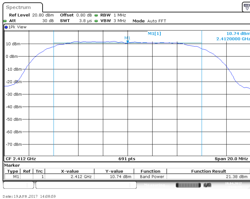
Figure 1: Maximum Transmitted Power, 2412 MHz at 11b 1Mbps
