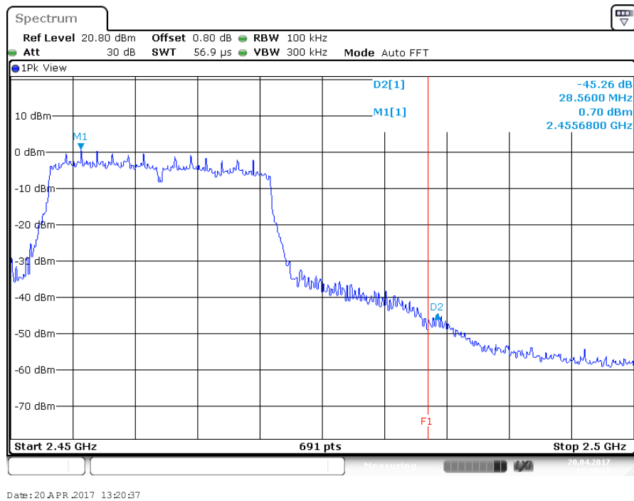
Figure 23: Measured Bandedge for HT20-MCS0 at 2462 MHz
