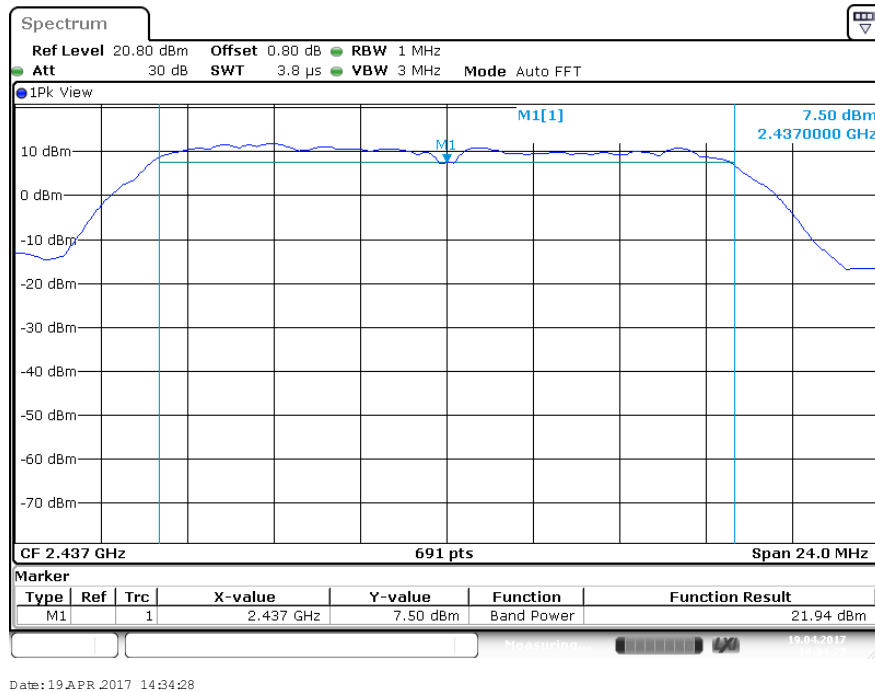
Figure 2: Maximum Transmitted Power, 2437 MHz at 11g 54Mbps
