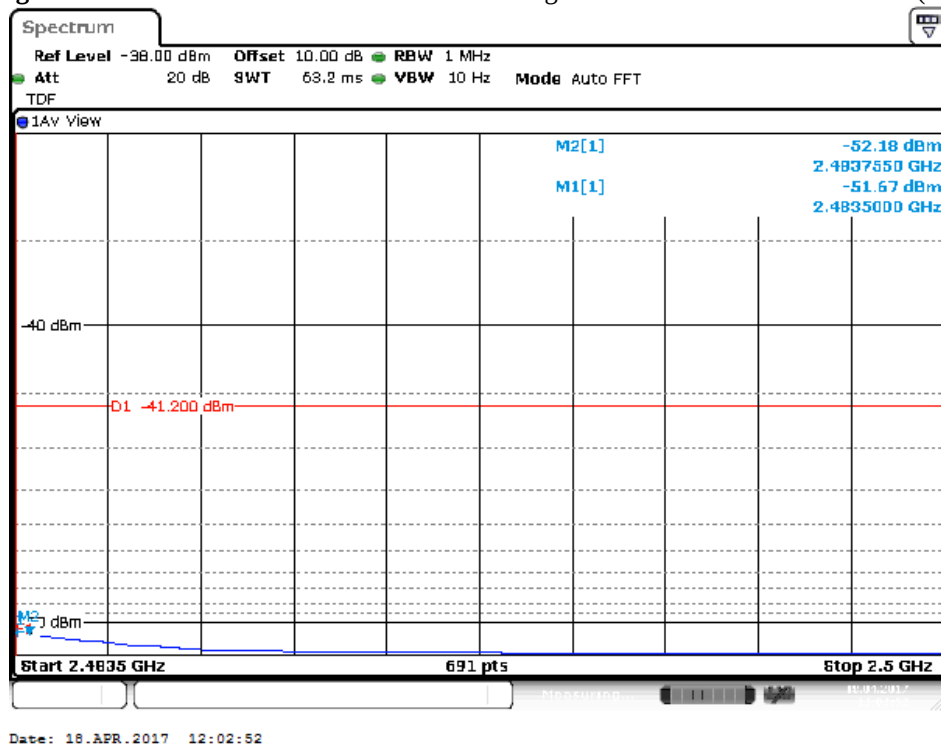
Figure 48: Radiated Emission at 2483.5 MHz Edge for 2462 MHz-802.11n-Vert (Ave)
