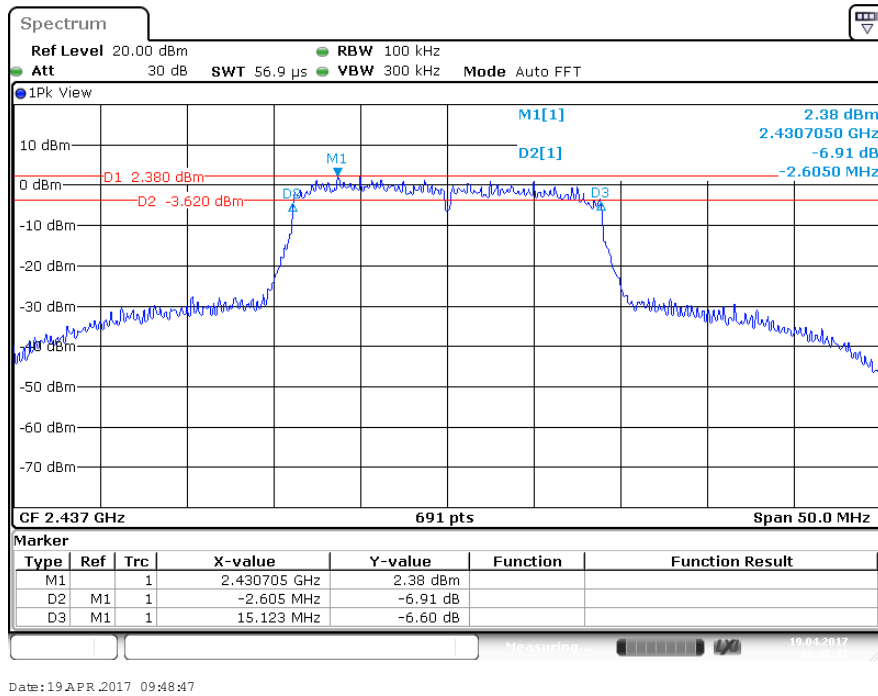
Figure 8: 6dB Bandwidth, 2437 MHz at HT20 MCS7
