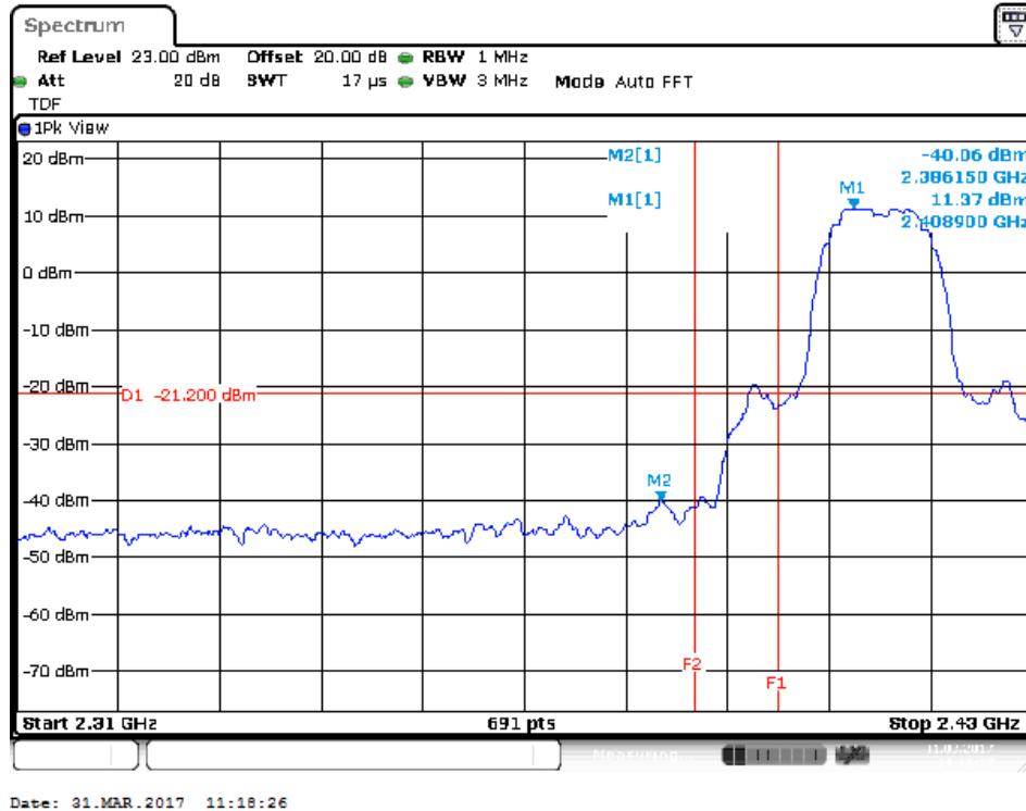
Figure 25: Radiated Emission at 2390 MHz Edge for 2412 MHz-802.11b – Vert. (Pk)
