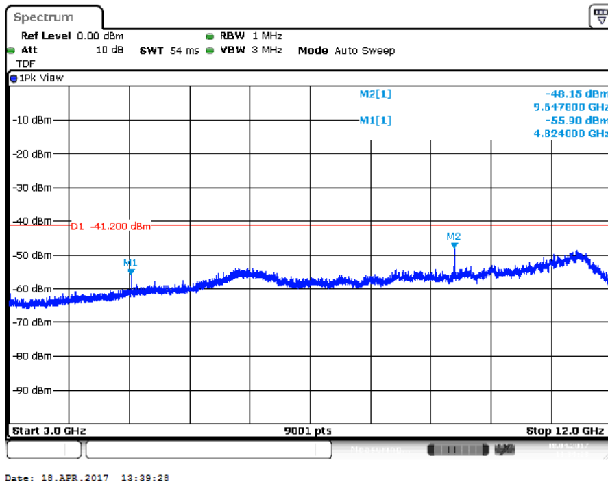
Plot of the emissions (peak values shown) in the range 3 -12 GHz, 802.11b 1Mbps, EUT H Ant V
