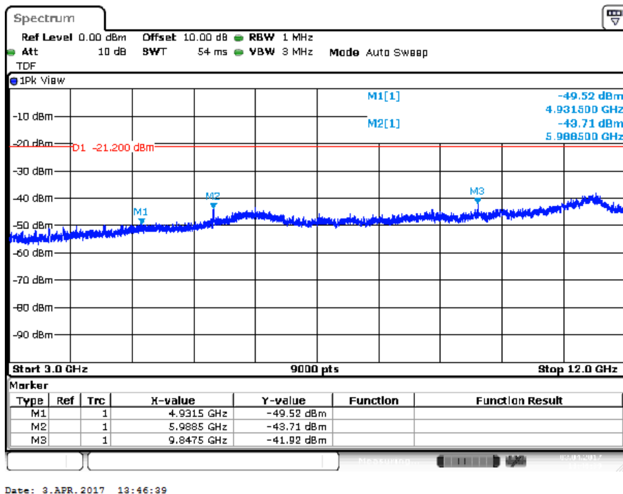
Plot of the emissions (peak values shown) in the range 3 -12 GHz, 802.11g 54Mbps, EUT Z Ant V
