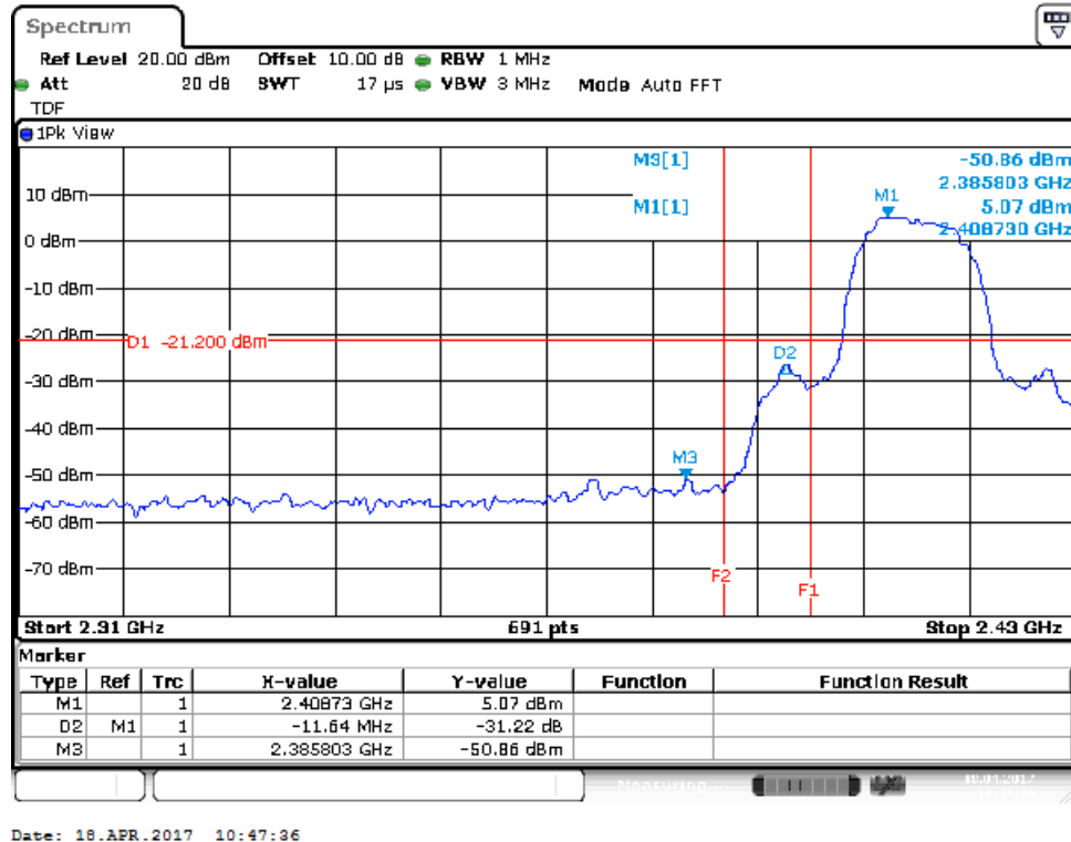
Figure 37: Radiated Emission at 2390 MHz Edge for 2412 MHz-802.11b- Vert. (Pk)
