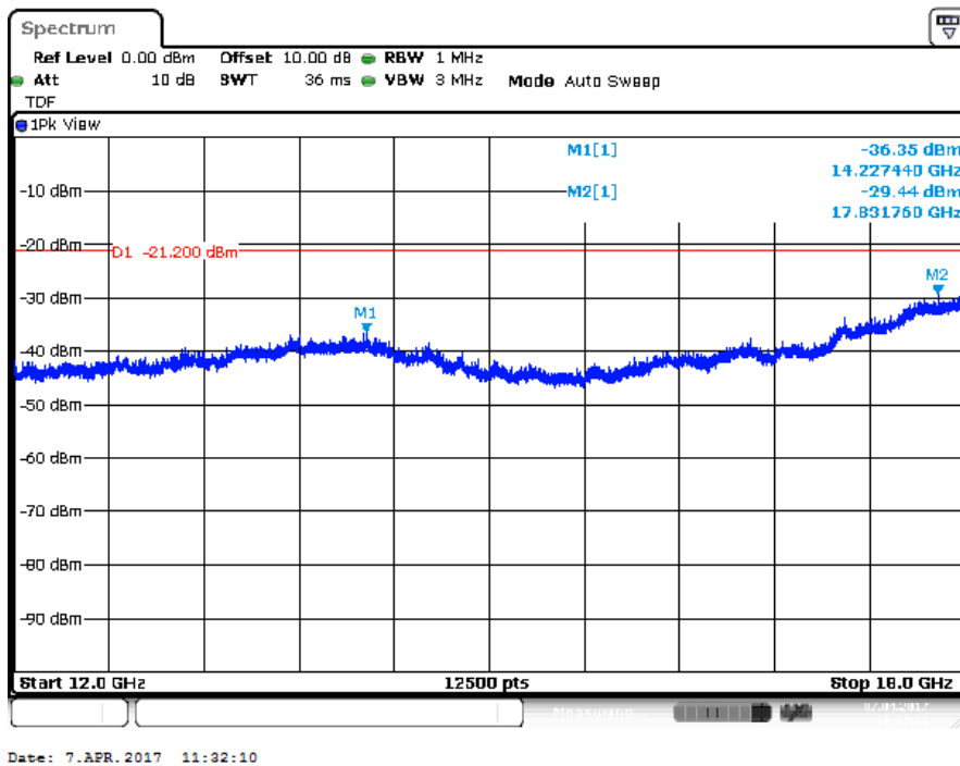
Plot of the emissions (peak values shown) in the range 12 -18 GHz, 802.11n mcs0 , EUT V Ant V
