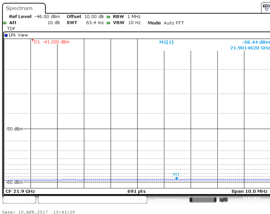
Plot of the emissions (average value shown) in the range 18-25 GHz, 802.11b 1Mbps, EUT Z Ant V
