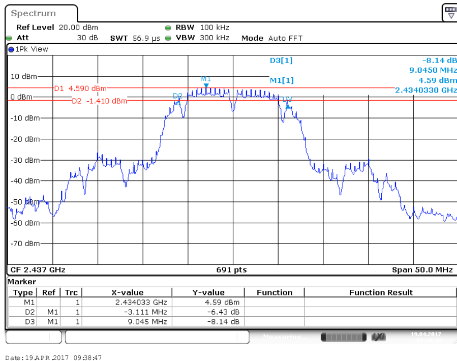
Figure 4: 6dB Bandwidth, 2437 MHz at 802.11b 1Mbps
