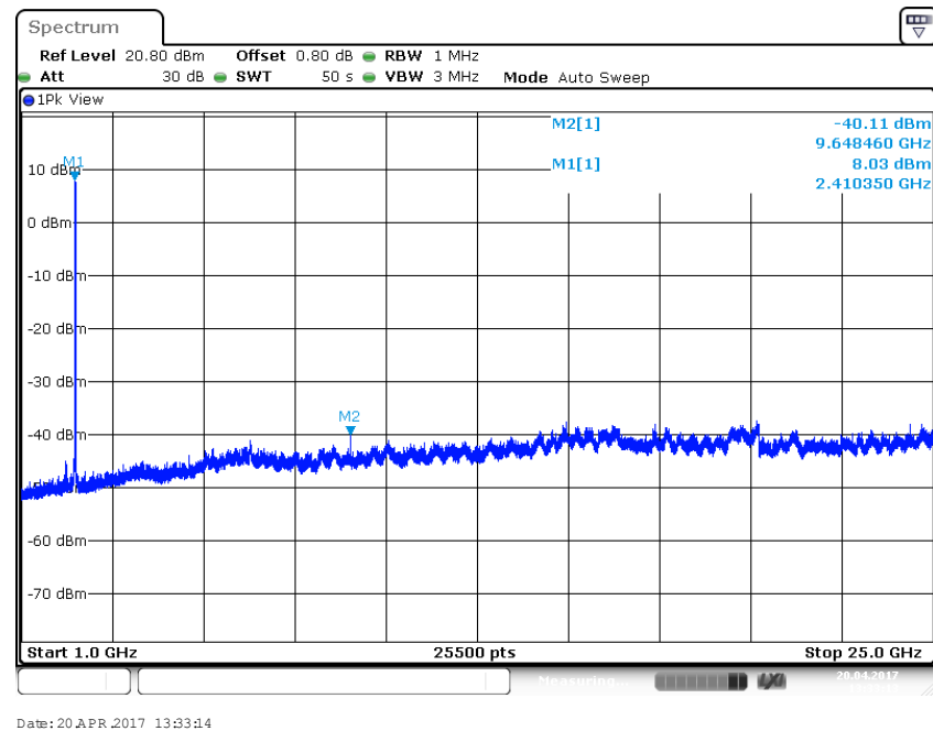
Figure 14: Out of Band Emissions for 802.11b-1Mbps at 2412 MHz
