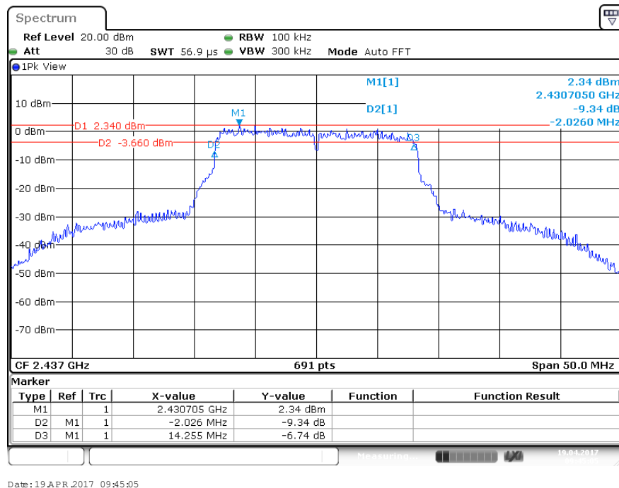
Figure 6: 6dB Bandwidth, 2437 MHz at 802.11g 54Mbps
