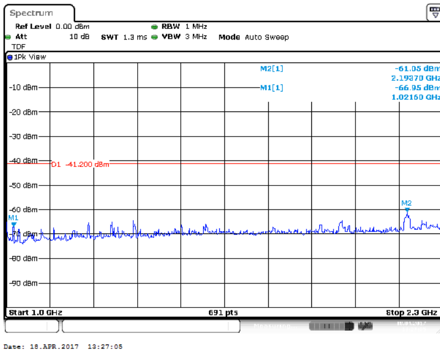
Plot of the emissions (peak values shown) in the range 1-2.3 GHz, 802.11n mcs0 , EUT V Ant H
