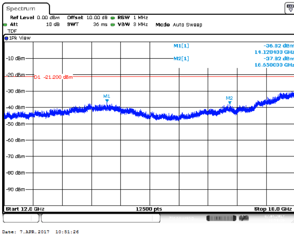
Plot of the emissions (peak values shown) in the range 12 -18 GHz, 802.11g 6Mbps, EUT V Ant V
