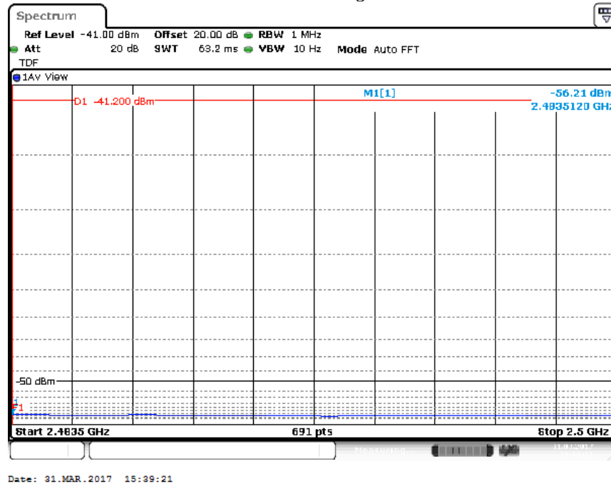
Figure 28: Radiated Emission at 2483.5 MHz Edge for 2462 MHz-802.11b – Vert. (Ave)
