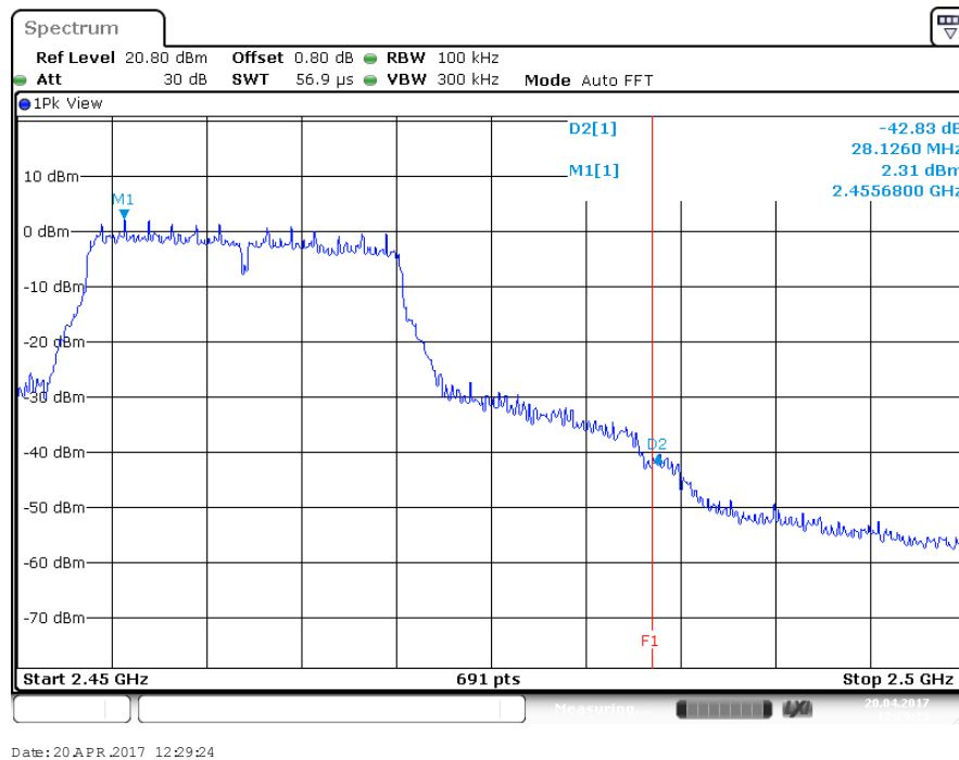
Figure 19: Measured Bandedge for 802.11g-6Mbps at 2462 MHz
