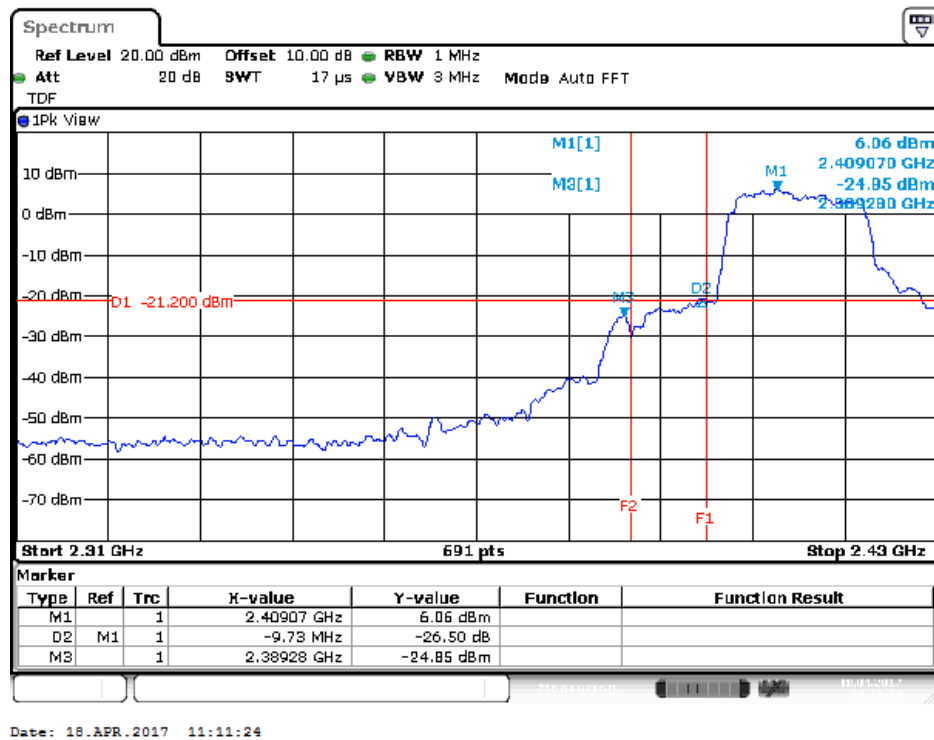
Figure 45: Radiated Emission at 2390 MHz Edge for 2412 MHz-802.11n- Vert. (Pk)
