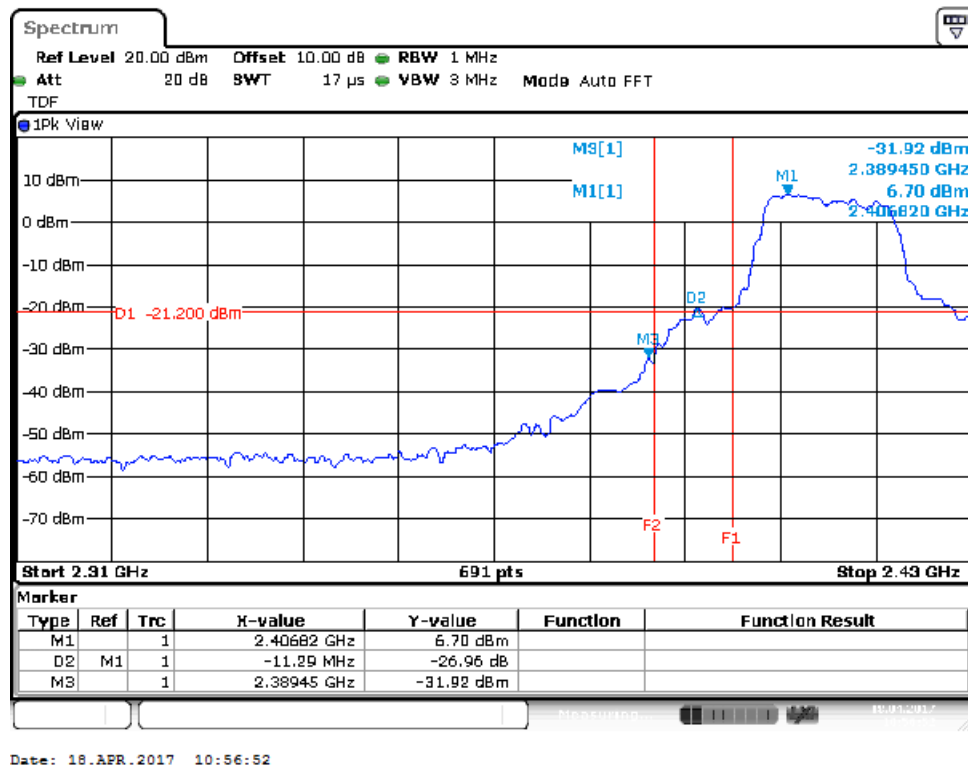
Figure 41: Radiated Emission at 2390 MHz Edge for 2412 MHz-802.11g- Vert. (Pk)
