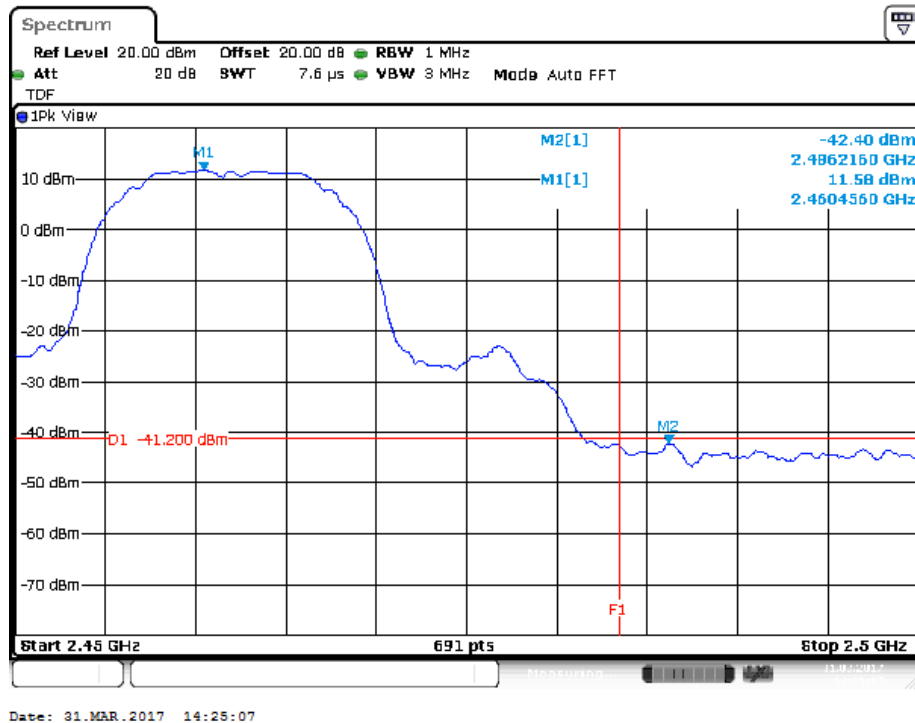
Figure 27: Radiated Emission at 2483.5 MHz Edge for 2462 MHz-802.11b – Vert. (Pk)
