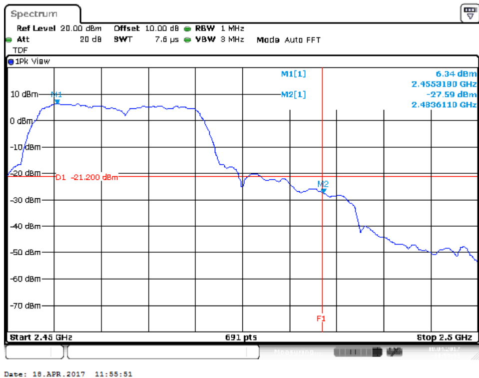
Figure 47: Radiated Emission at 2483.5 MHz Edge for 2462 MHz-802.11n-Horz. (Pk)
