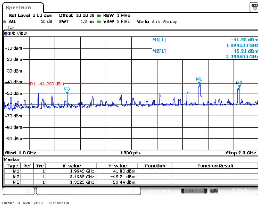
Plot of the emissions (peak values shown) in the range 1-2.3 GHz, 802.11g 54Mbps, EUT Z Ant V
