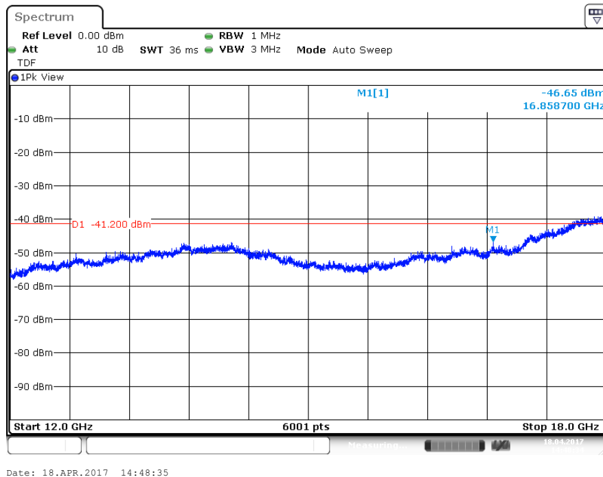
Plot of the emissions (peak values shown) in the range 12-18 GHz, 802.11b 1Mbps, EUT V Ant V
