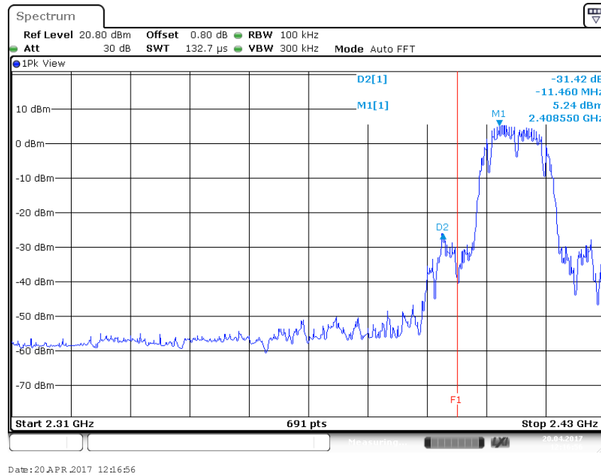
Figure 13: Measured Bandedge for 802.11b-1Mbps at 2412 MHz
