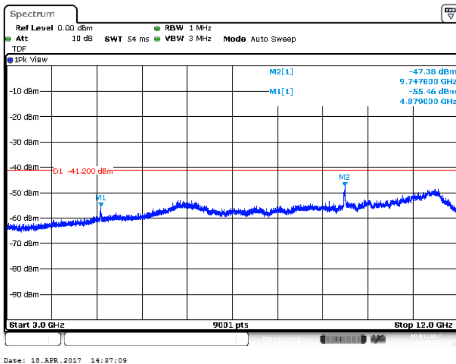
Plot of the emissions (peak values shown) in the range 3 -12 GHz, 802.11n mcs7 , EUT H Ant V
