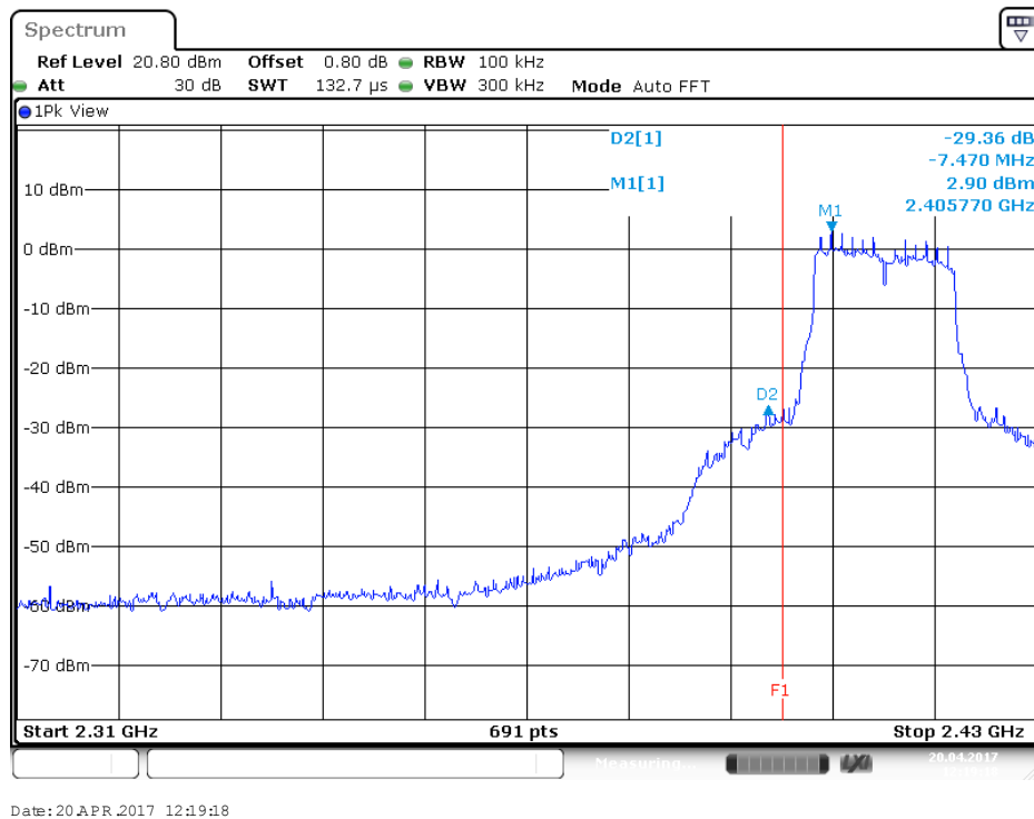
Figure 17: Measured Bandedge for 802.11g-6Mbps at 2412 MHz
