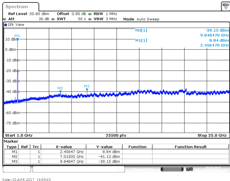
Figure 24: Out of Band Emissions for HT20-MCS0 at 2462 MHz
