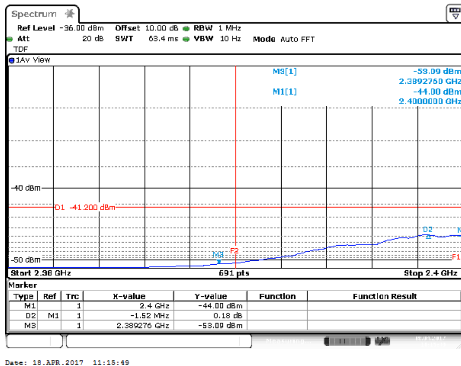
Figure 46: Radiated Emission at 2390 MHz Edge for 2412 MHz-802.11n- Vert. (Ave)
