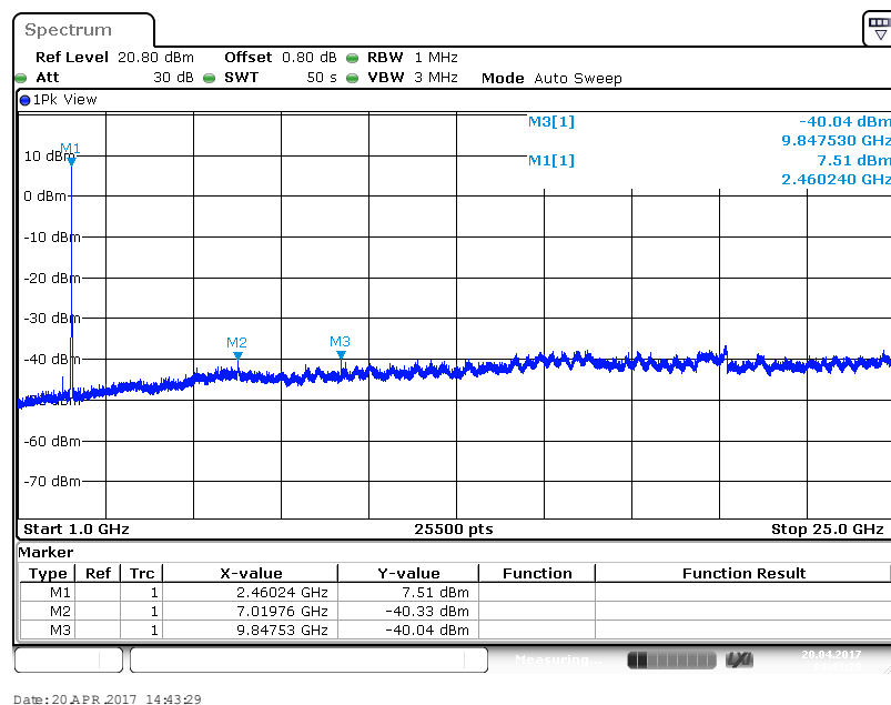
Figure 16: Out of Band Emissions for 802.11b-1Mbps at 2462 MHz
