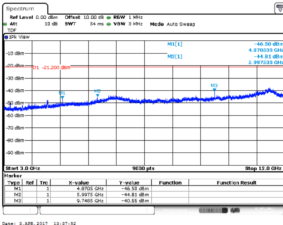
Plot of the emissions (peak values shown) in the range 3 -12 GHz, 802.11g 6Mbps, EUT Z Ant V
