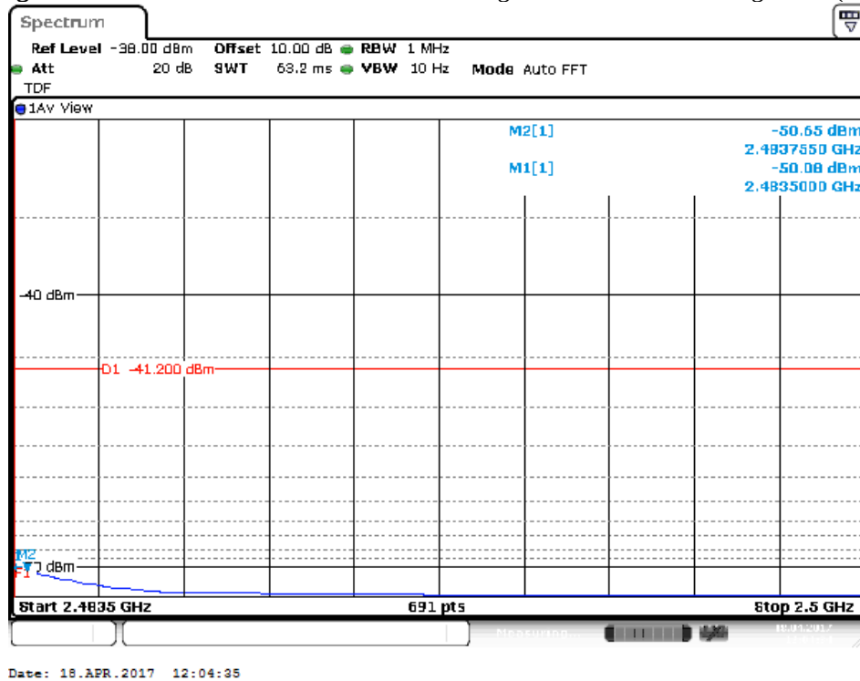
Figure 44: Radiated Emission at 2483.5 MHz Edge for 2462 MHz-802.11g- Vert. (Ave)
