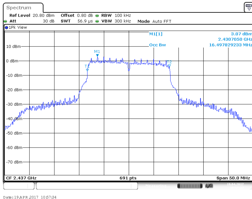
Figure 7: 99% Occupied Bandwidth, 2437 MHz at 802.11g 6Mbps
