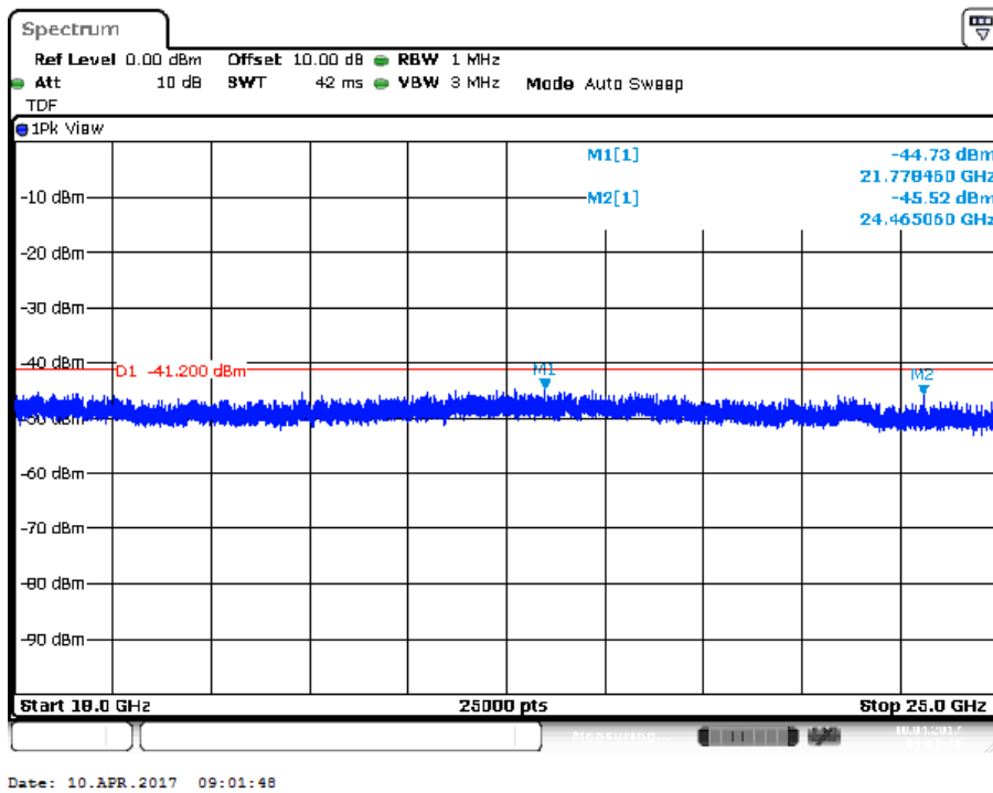
Plot of the emissions (peak values shown) in the range 18-25 GHz, 802.11b 1Mbps, EUT Z Ant V
