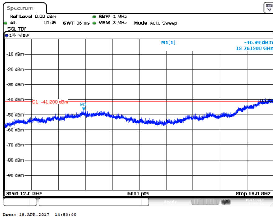
Plot of the emissions (peak value shown) in the range 12-18 GHz, 802.11b 1Mbps, EUT V Ant H
