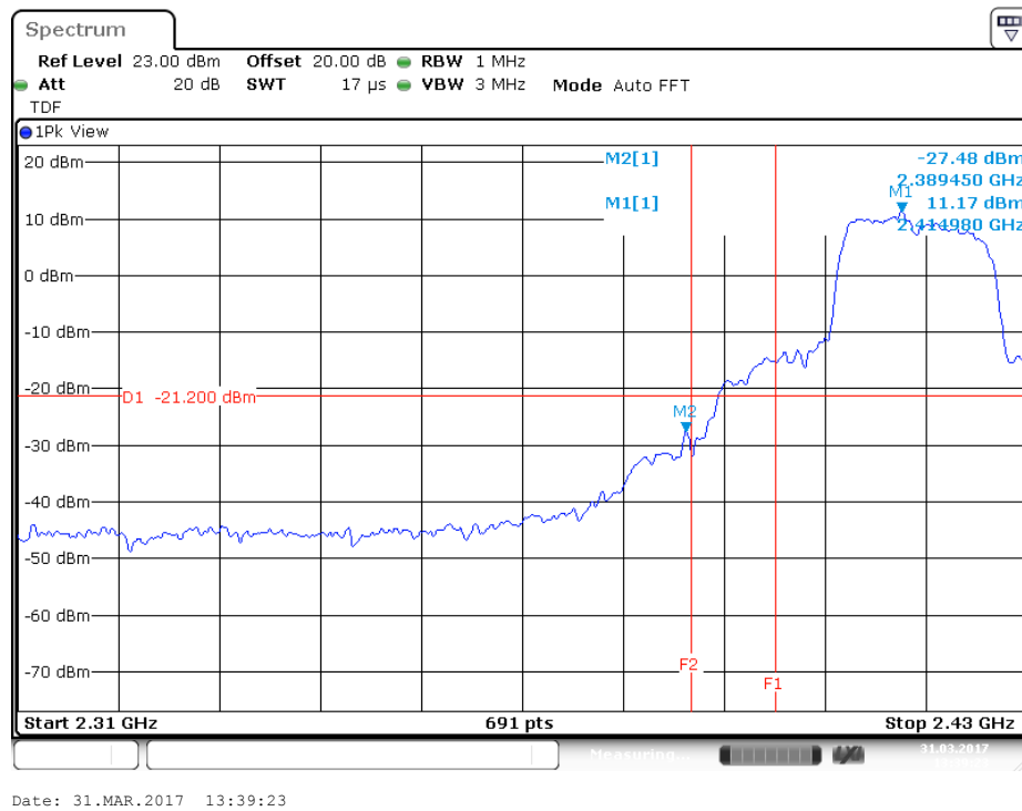
Figure 33: Radiated Emission at 2390 MHz Edge for 2412 MHz-802.11n – Vert. (Pk)
