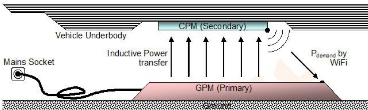
Figure 1: System description
