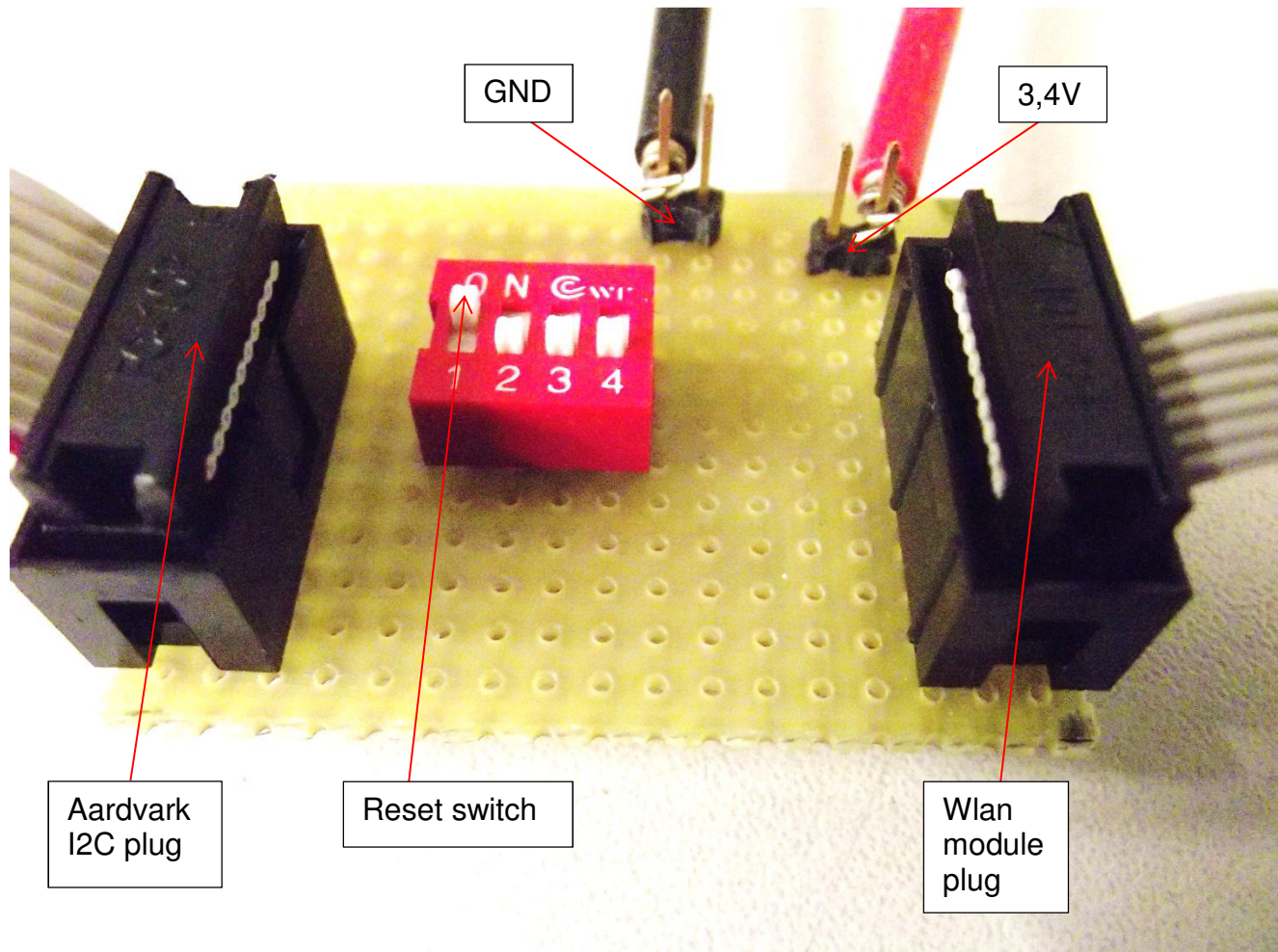
Figure 10: Adapter board
