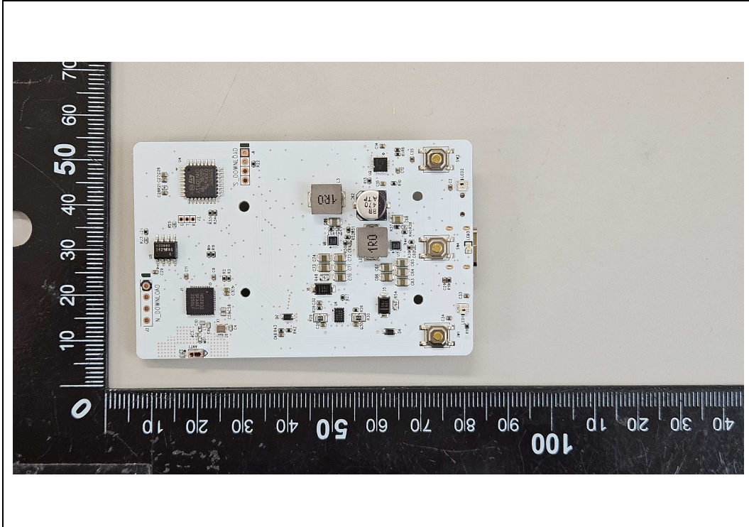
Main Board_Front
