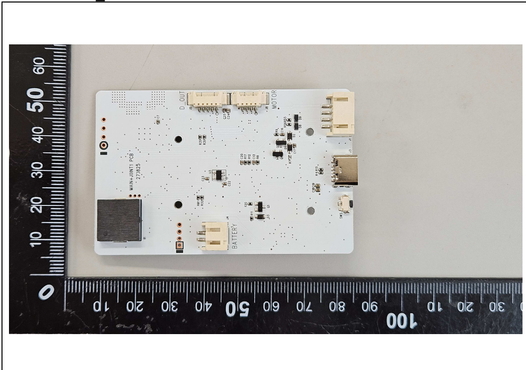
Main Board_Rear
