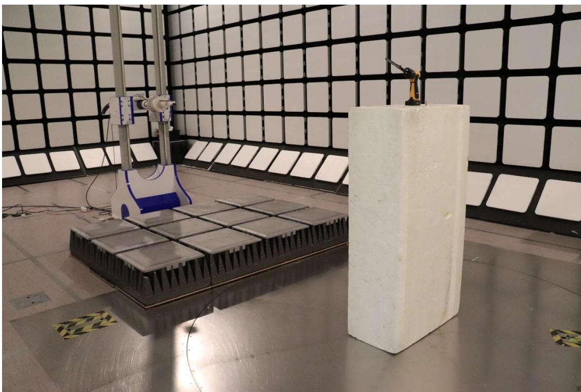
Photograph 4: Radiated emissions 18 – 25 GHz
