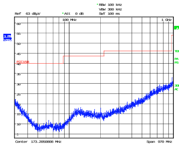
Figure 8.3-12: Radiated spurious emissions, high channel, 30 to 1000 MHz
