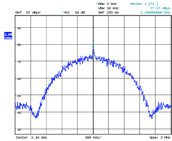
Figure 8.4-2: PSD sample plot on mid channel
