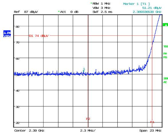
Figure 8.3-8: Radiated spurious emissions Lower band edge emission, low channel. F2 = 2.39 GHz (end of restricted band), F1 = 2.4 GHz
