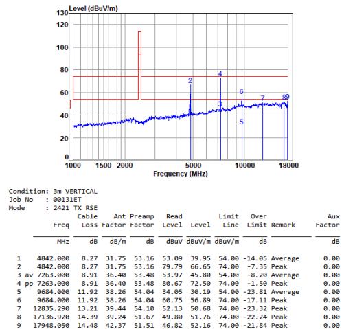
2.4G_SRD_MID_TX_Vertical
