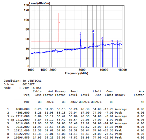
2.4G_SRD_LOW_TX_Vertical
