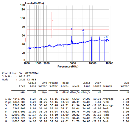
2.4G_SRD_MID_TX_Horizontal
