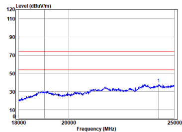
2.4G_SRD_LOW_TX_Vertical
