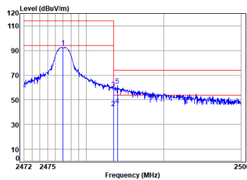
2.4G_SRD_HIGH_TX_Horizontal
