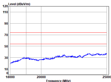
2.4G_SRD_LOW_TX_Vertical
