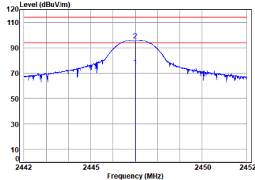
2.4G_SRD_MID_TX_Vertical
