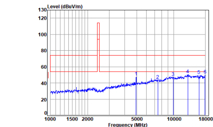
2.4G_SRD_HIGH_TX_Horizontal
