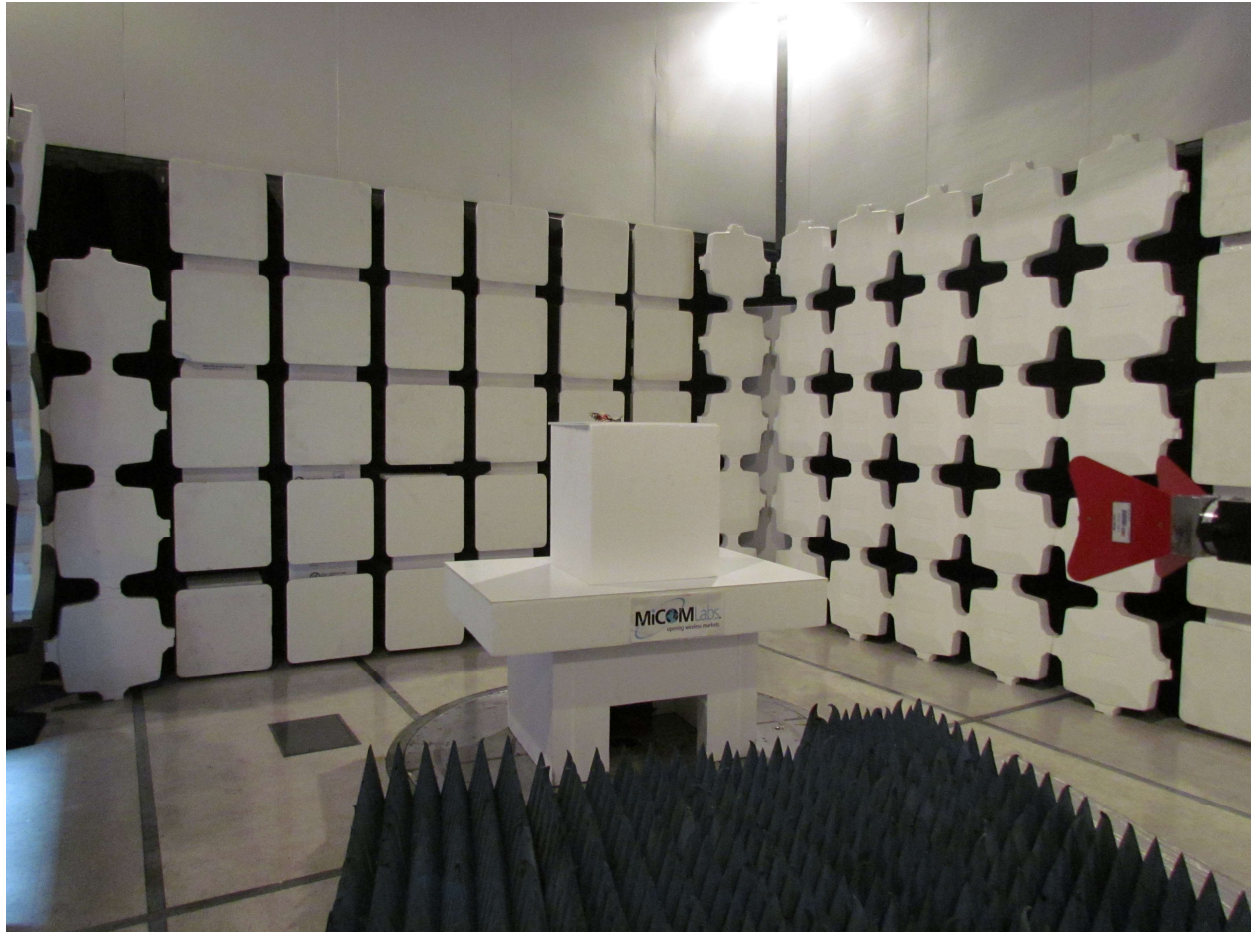
Spurious Emissions 1-18GHz
