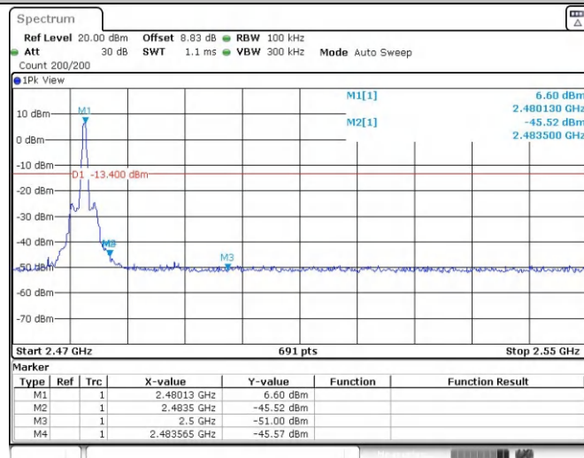
DH5_Ant1_High_2480
