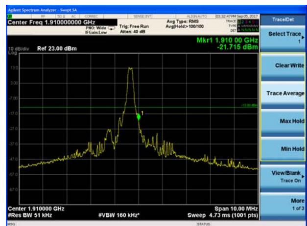
LTE Band 2 5MHz QPSK 6RB CH-High
