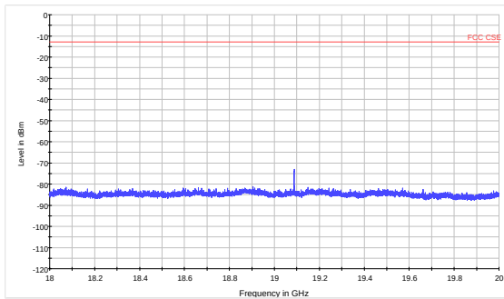
LTE Band 2 1.4MHz CH-High 18GHz~20GHz
