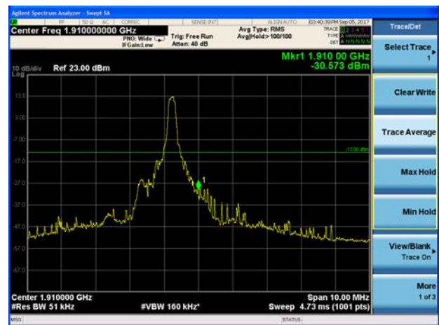
LTE Band 2 10MHz 16QAM 6RB CH-High
