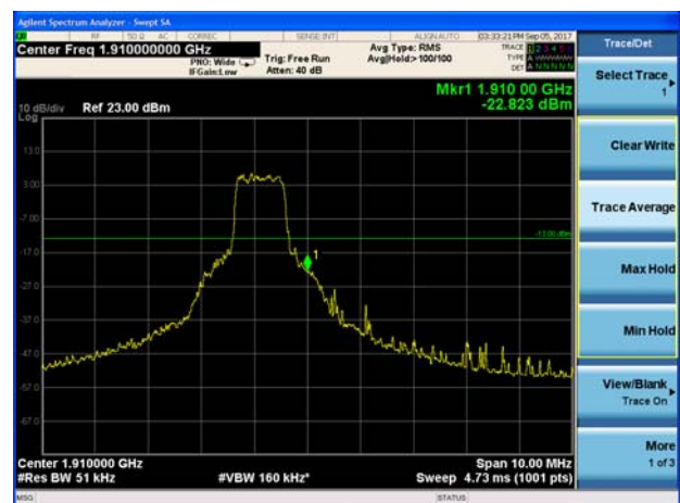
LTE Band 2 5MHz 16QAM 6RB CH-High
