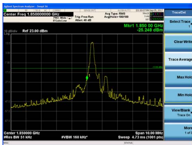
LTE Band 2 5MHz 16QAM 6RB CH-Low
