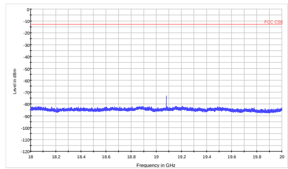
LTE Band 2 3MHz CH-High 18GHz~20GHz
