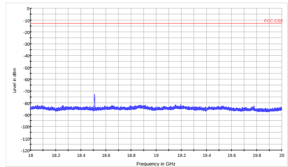
LTE Band 2 3MHz CH-Low 18GHz~20GHz
