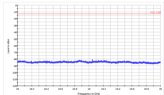
LTE Band 2 10MHz CH-High 18GHz~20GHz
