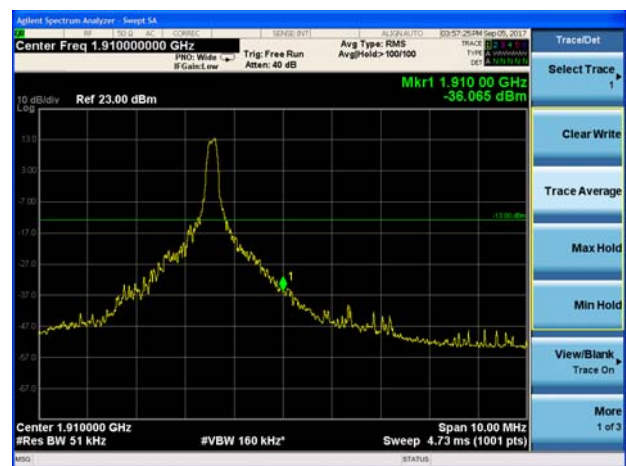
LTE Band 2 20MHz QPSK 6RB CH-High
