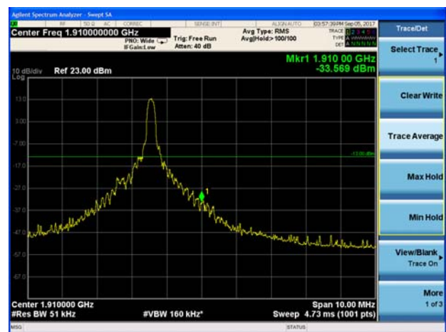
LTE Band 2 20MHz 16QAM 6RB CH-High
