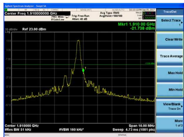
LTE Band 2 5MHz 16QAM 6RB CH-High
