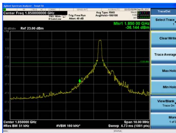
LTE Band 2 20MHz QPSK 6RB CH-Low
