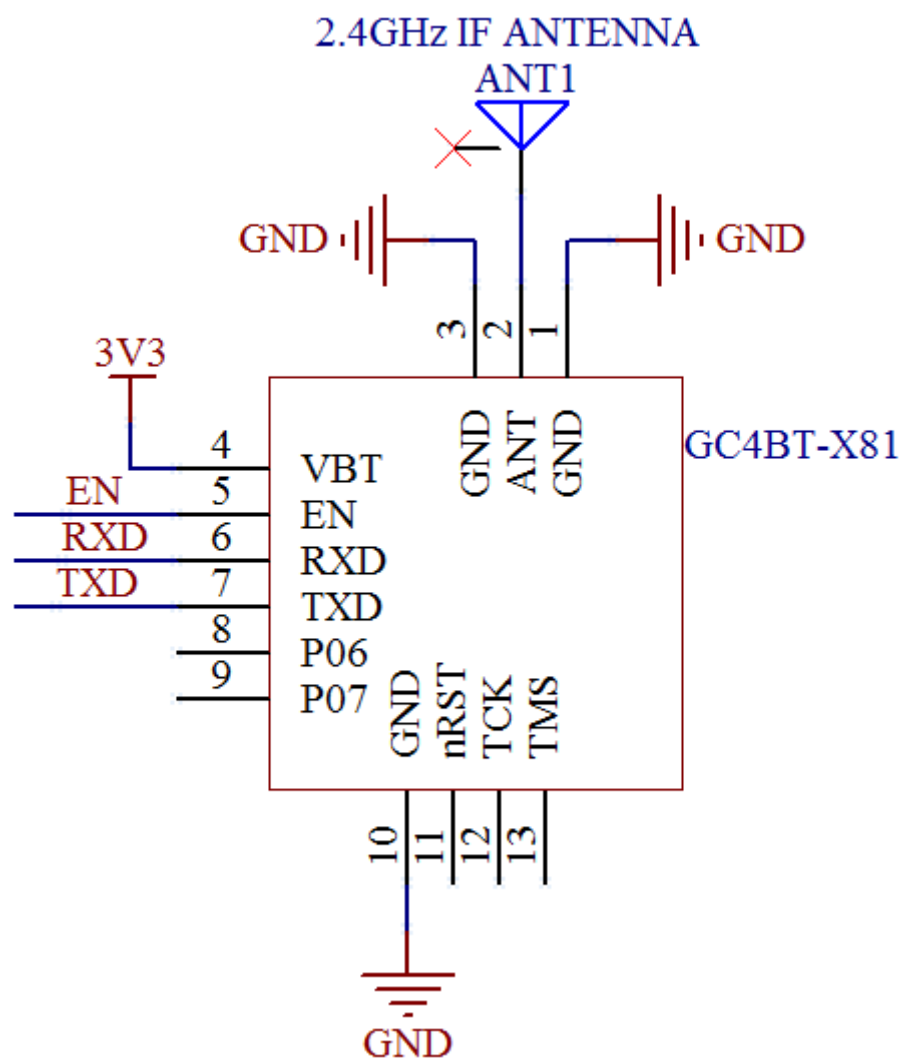
Fig 6-1 TransmissionTypical application Diagram
