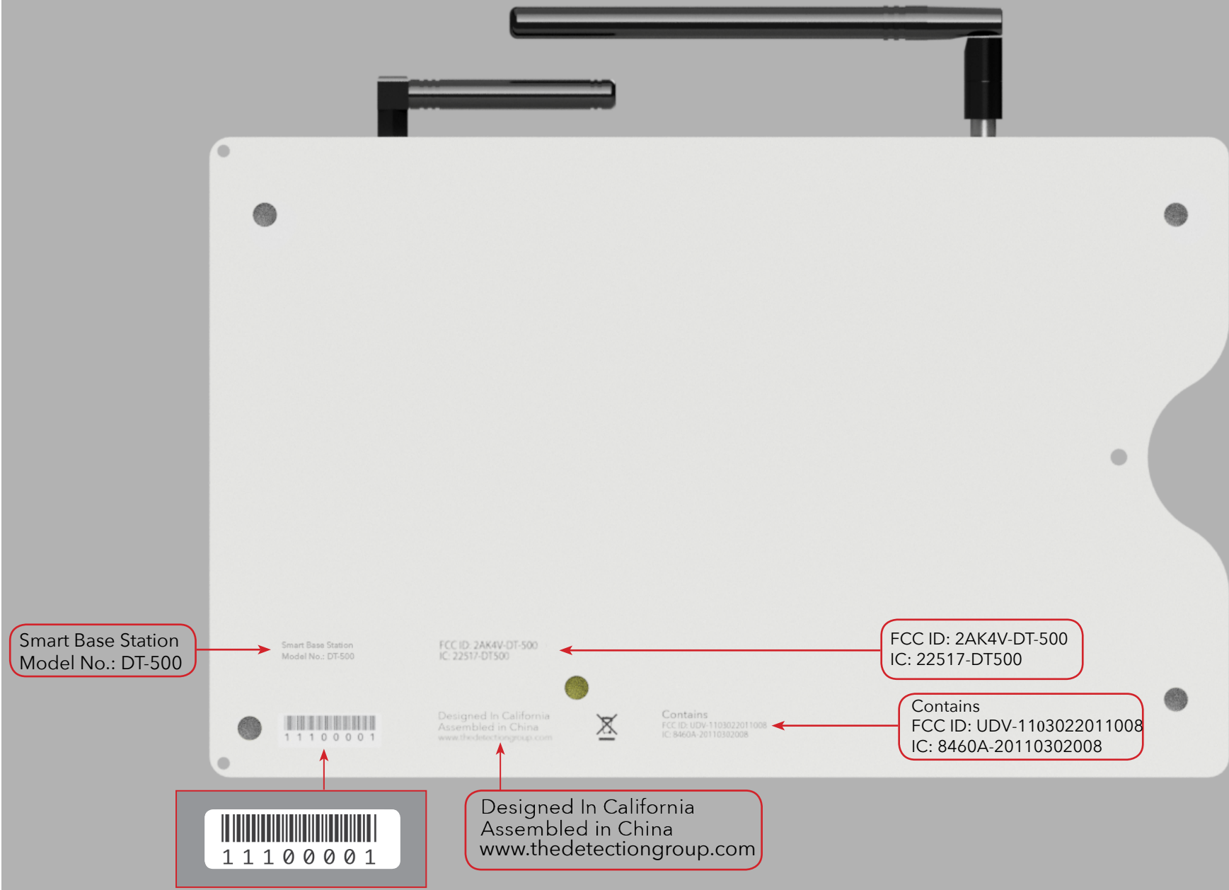
Adhesive Label
