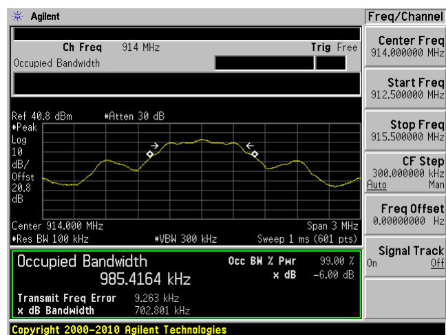
Middle Channel 914 MHz
