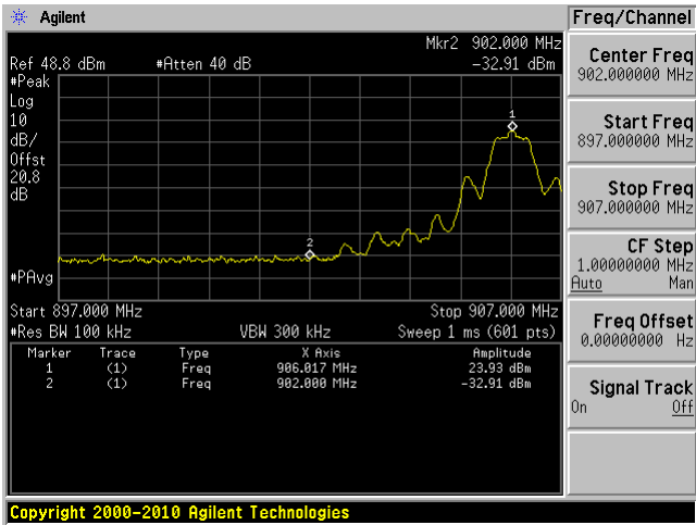
Low Channel 906 MHz
