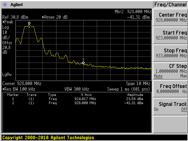
High Channel 924 MHz
