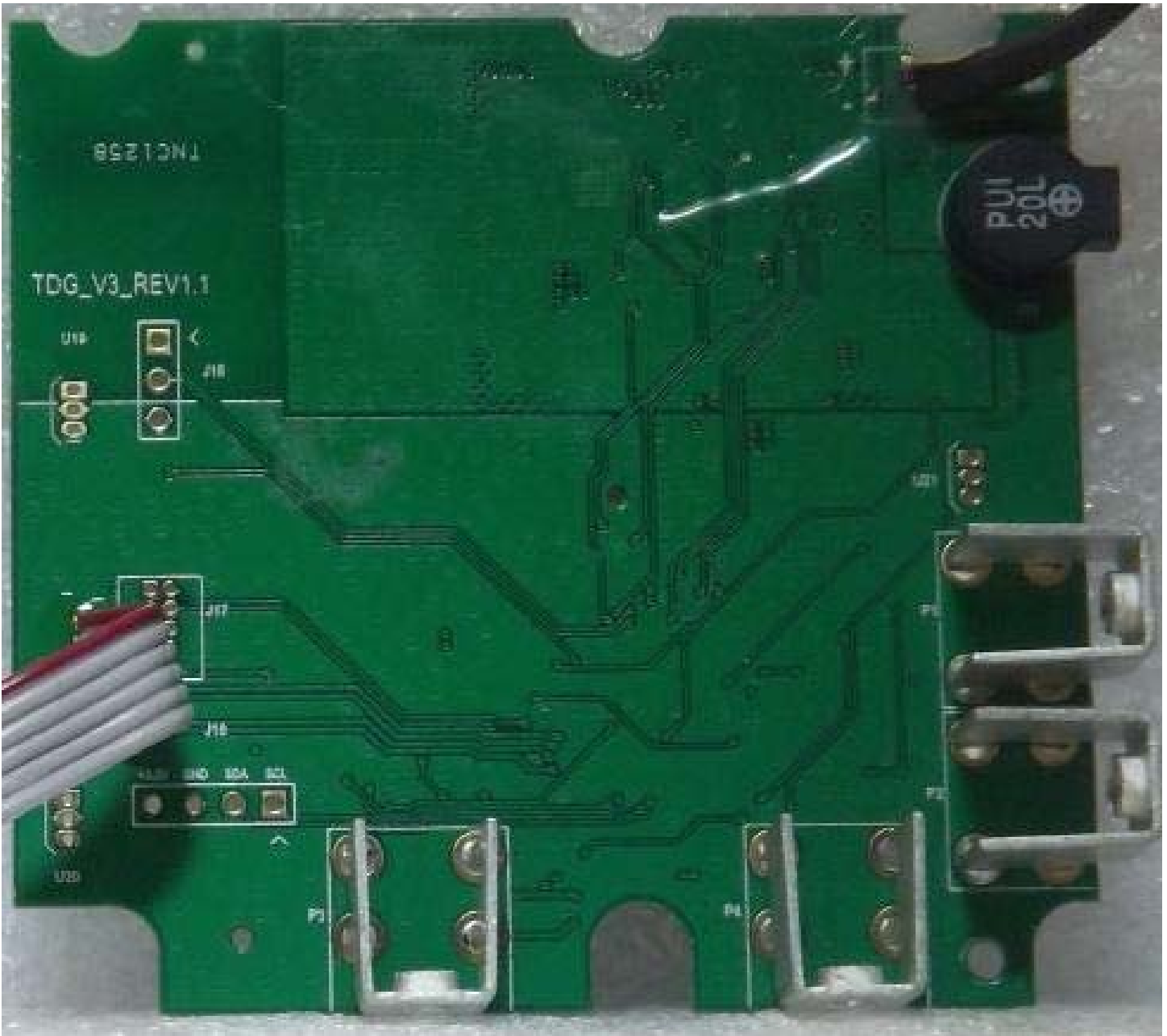
Figure E22.7 – Main PCB, Back Side
