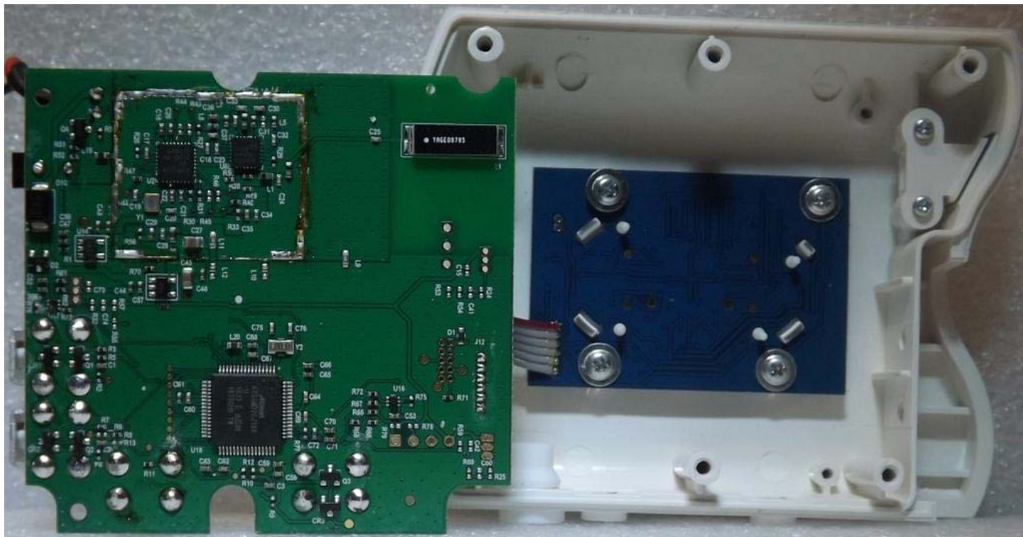
Figure E22.4 – Main PCB Removed
