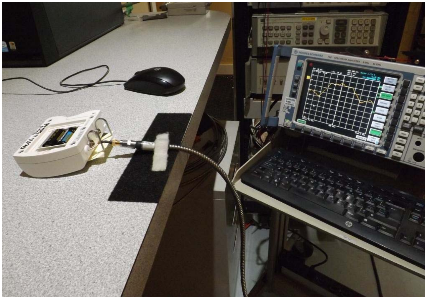
Figure E23.1 – Setup, Antenna Port Conducted Measurements
