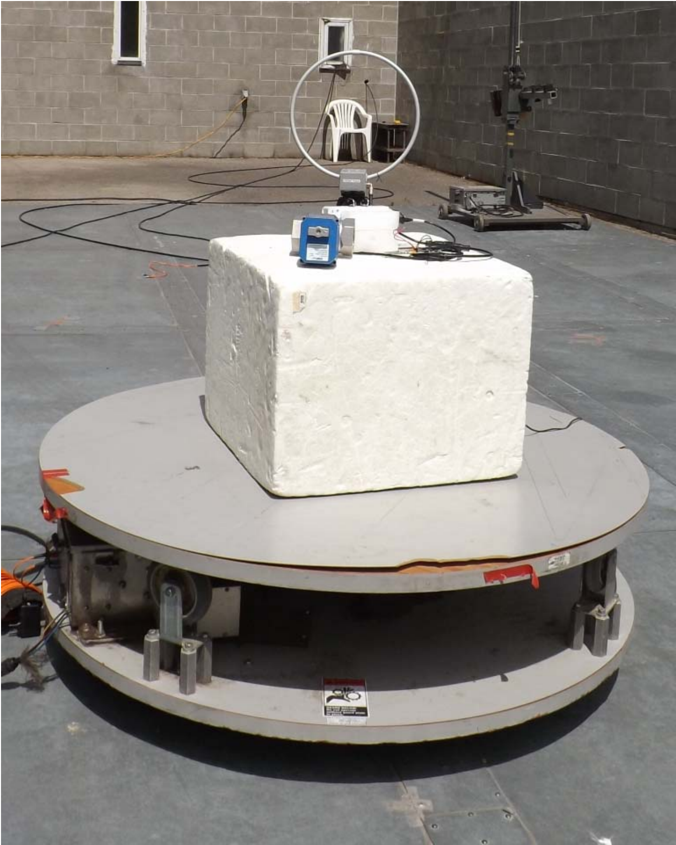
Figure E23.3 – Setup, Radiated Emissions Measurements Below 30MHz
