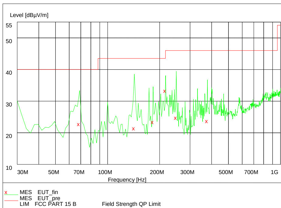
Pic4. Radiated emission (30MHz – 1GHz)
