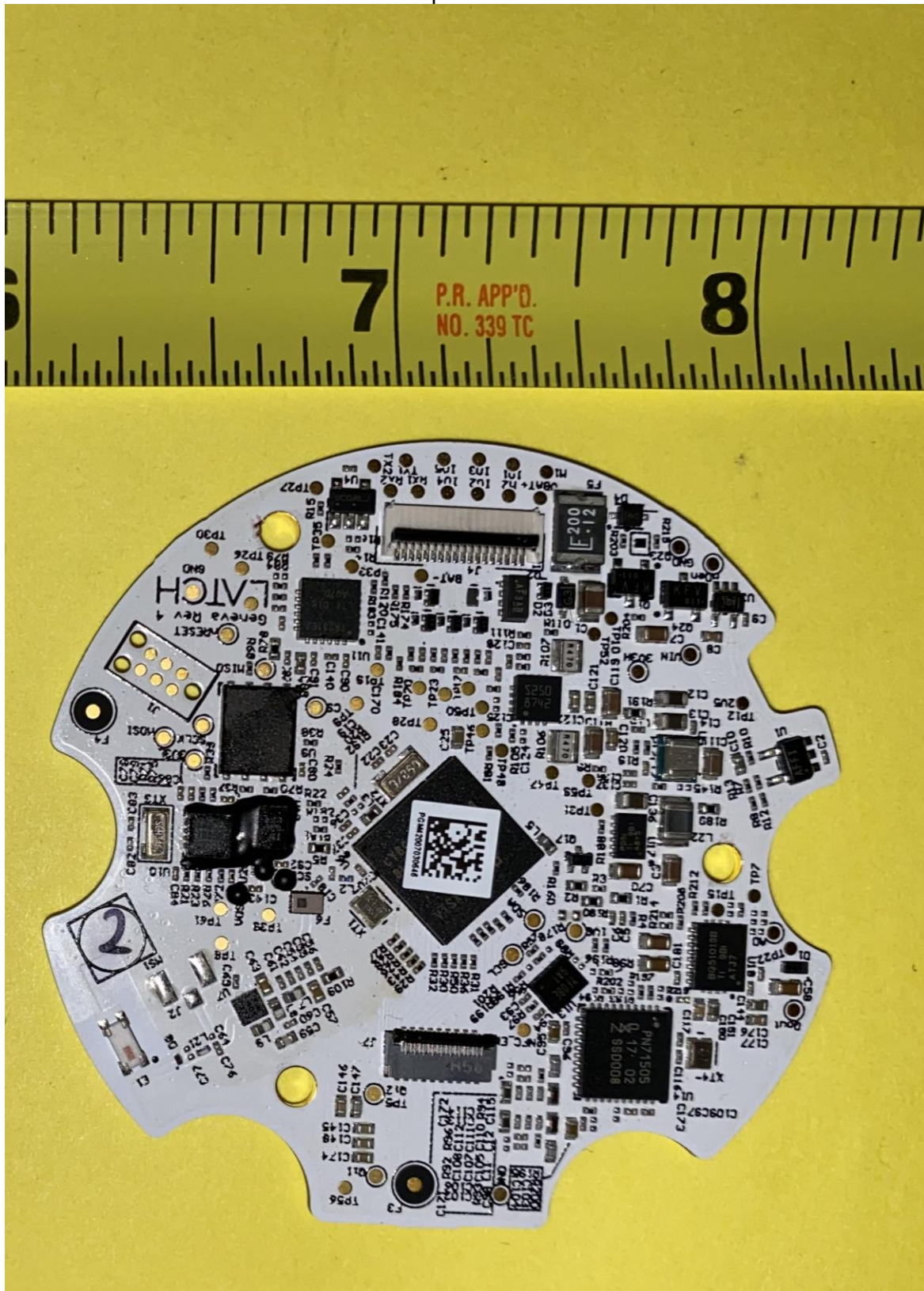
Component side
