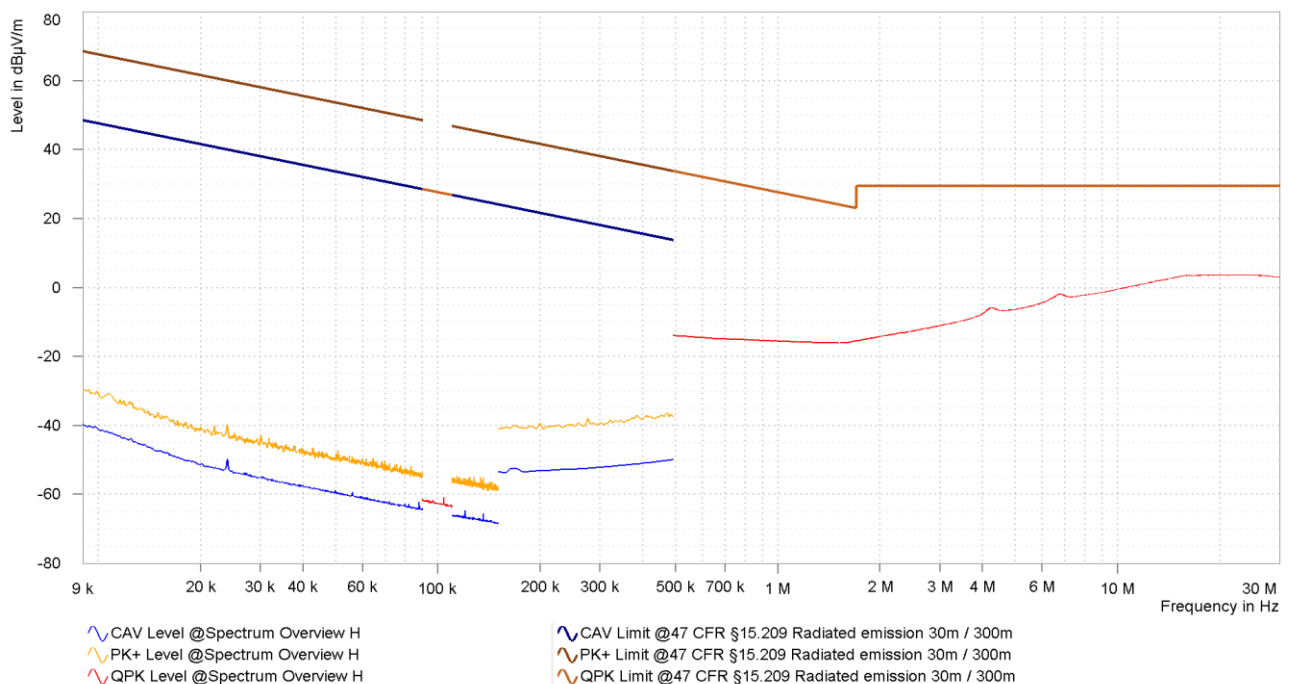
Figure 34: Chart of emissions test below 30 MHz on middle channel, EUT position Y, antenna parallel
