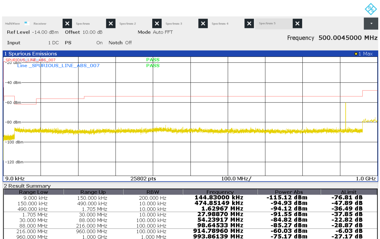
Figure 22: Chart of emissions test from 9 kHz to 1 GHz on lowest channel, PK
