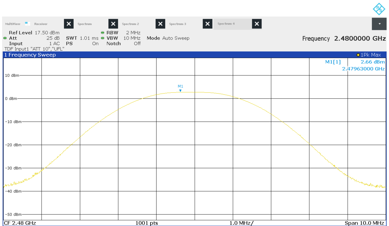
Figure 15: Chart of conducted output power on highest channel
