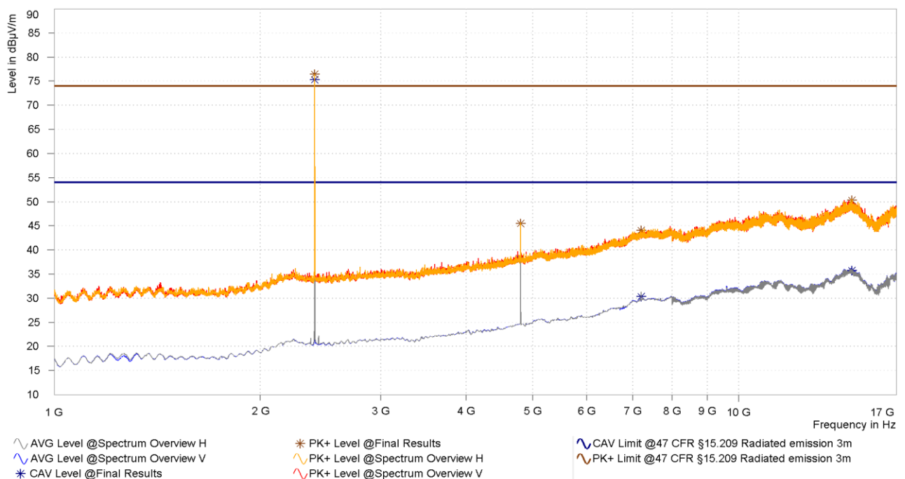
Figure 36: Chart of radiated emissions pre-measurement from 1 GHz to 17 GHz on lowest channel, EUT position Y, antenna polarization horizontal and vertical
