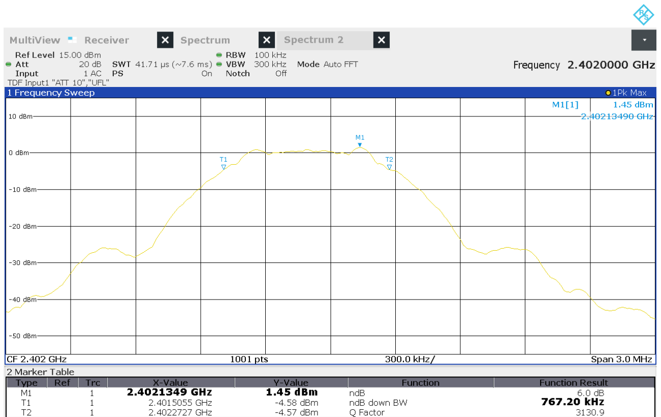
Figure 7: Chart of 6 dB bandwidth test on lowest channel
