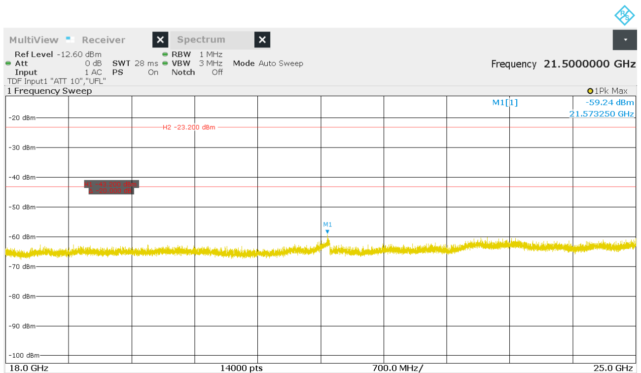
Figure 25: Chart of emissions test from 18 GHz to 25 GHz on lowest channel, Pk
