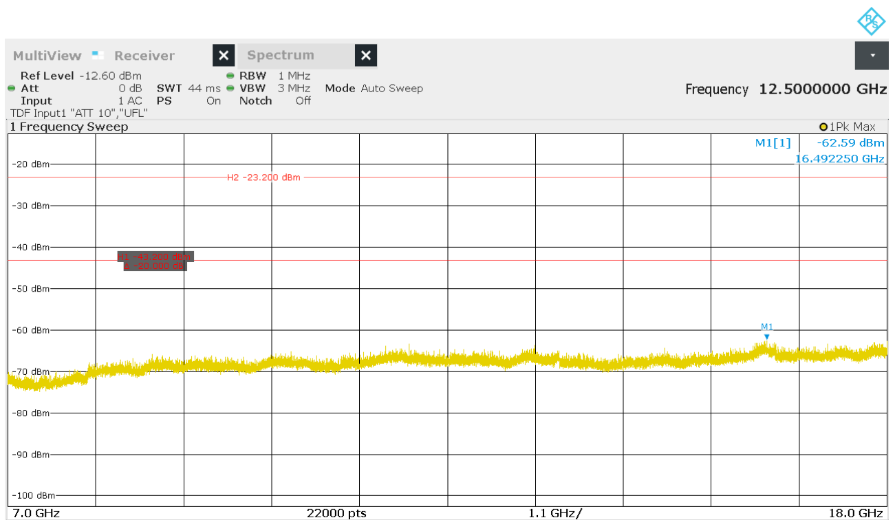
Figure 28: Chart of emissions test from 7 GHz to 18 GHz on middle channel, Pk
