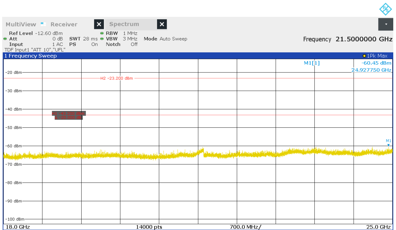
Figure 33: Chart of emissions test from 18 GHz to 25 GHz on highest channel, Pk
