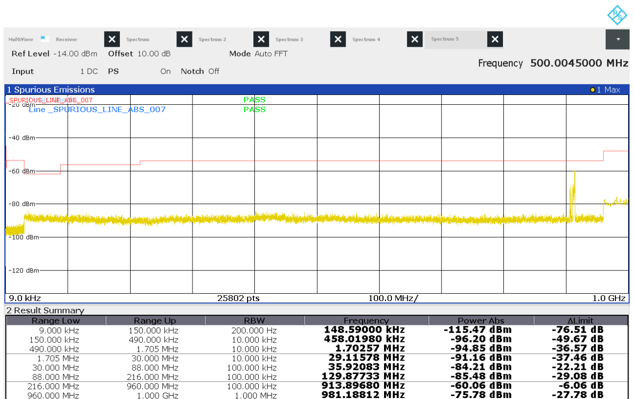
Figure 30: Chart of emissions test from 9 kHz to 1 GHz on highest channel, PK
