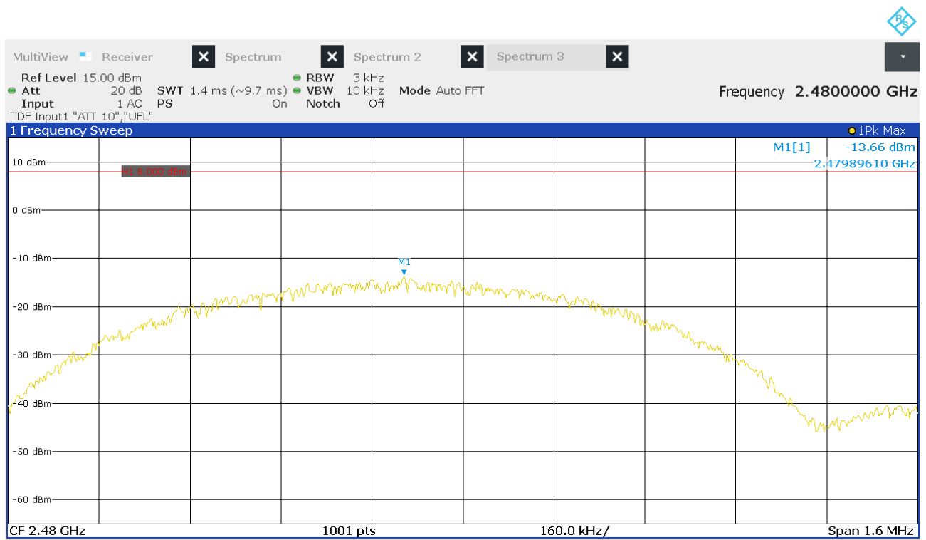
Figure 18: Chart of power spectral density on highest channel
