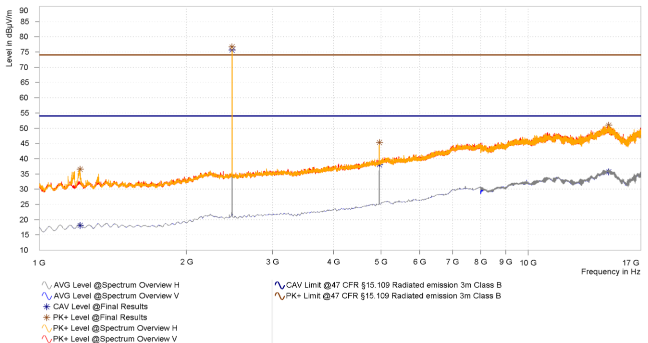
Figure 40: Chart of radiated emissions pre-measurement from 1 GHz to 17 GHz on highest channel, EUT position Y, antenna polarization horizontal and vertical
