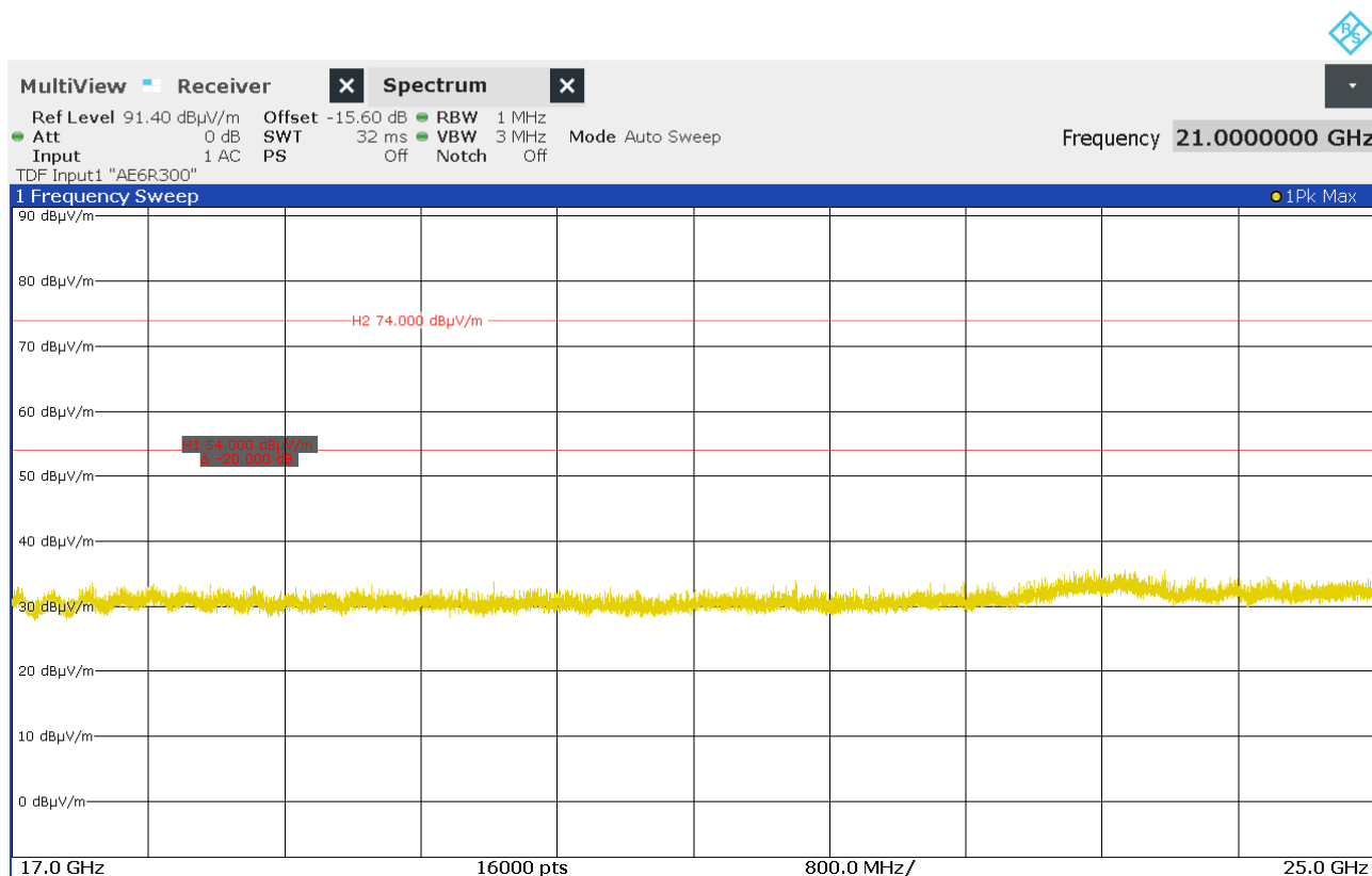
Figure 39: Chart of exploratory emissions measurement from 17 GHz to 25 GHz on middle channel, EUT position X, antenna polarization horizontal and vertical
