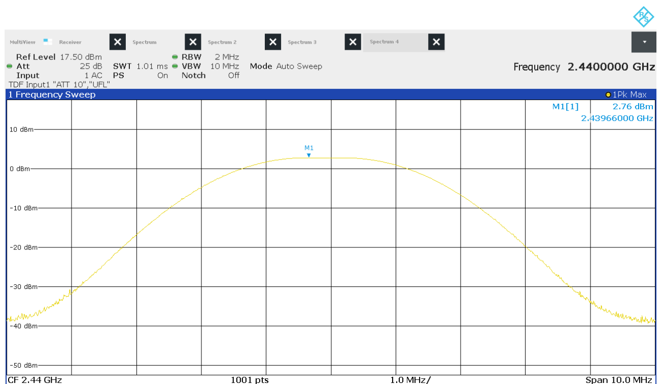
Figure 14: Chart of conducted output power on middle channel
