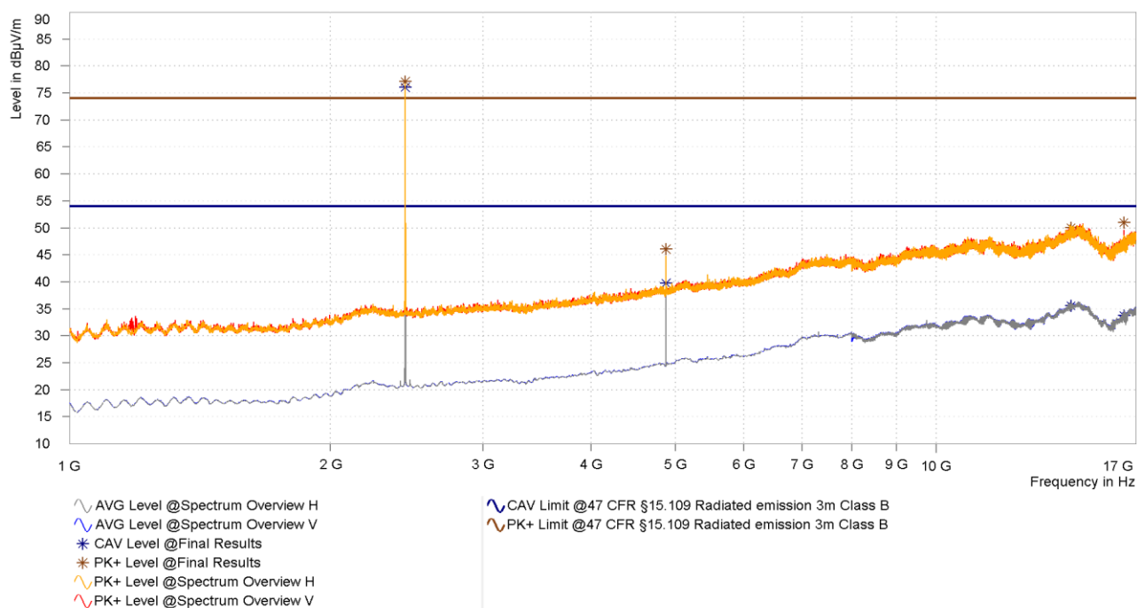
Figure 38: Chart of radiated emissions pre-measurement from 1 GHz to 17 GHz on middle channel, EUT position Y, antenna polarization horizontal and vertical
