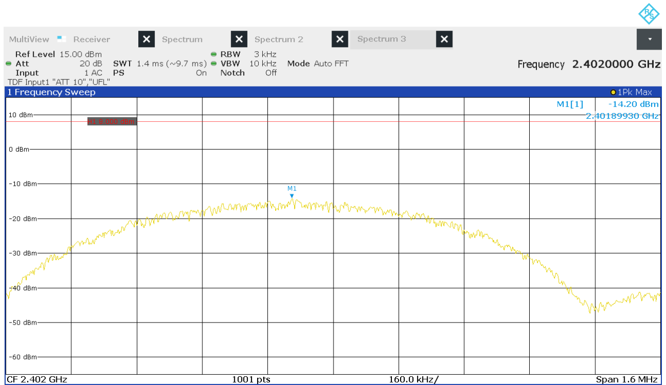
Figure 16: Chart of power spectral density on lowest channel
