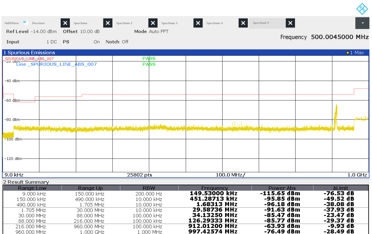
Figure 26: Chart of emissions test from 9 kHz to 1 GHz on middle channel, PK
