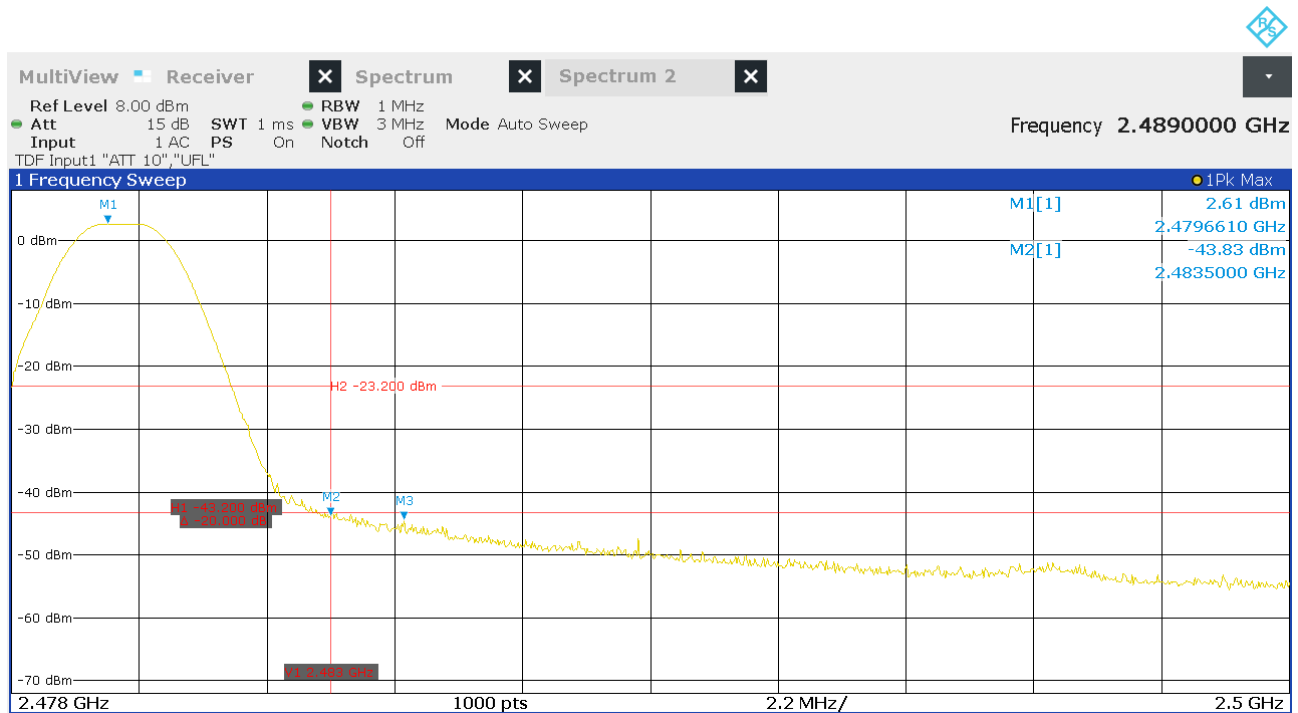
Figure 20: Chart of upper band-edge measurement on highest channel (PK)
