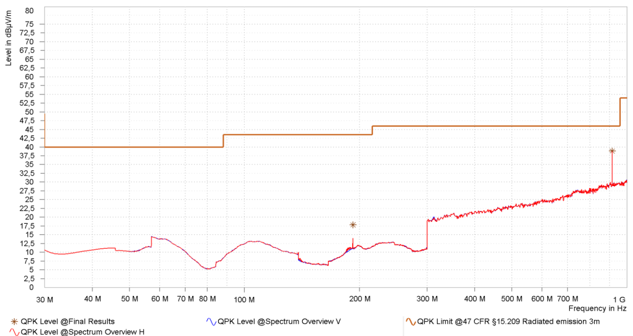
Figure 35: Chart of radiated emissions test from 30 MHz to 1 GHz on middle channel, EUT position Y, antenna polarization horizontal and vertical
