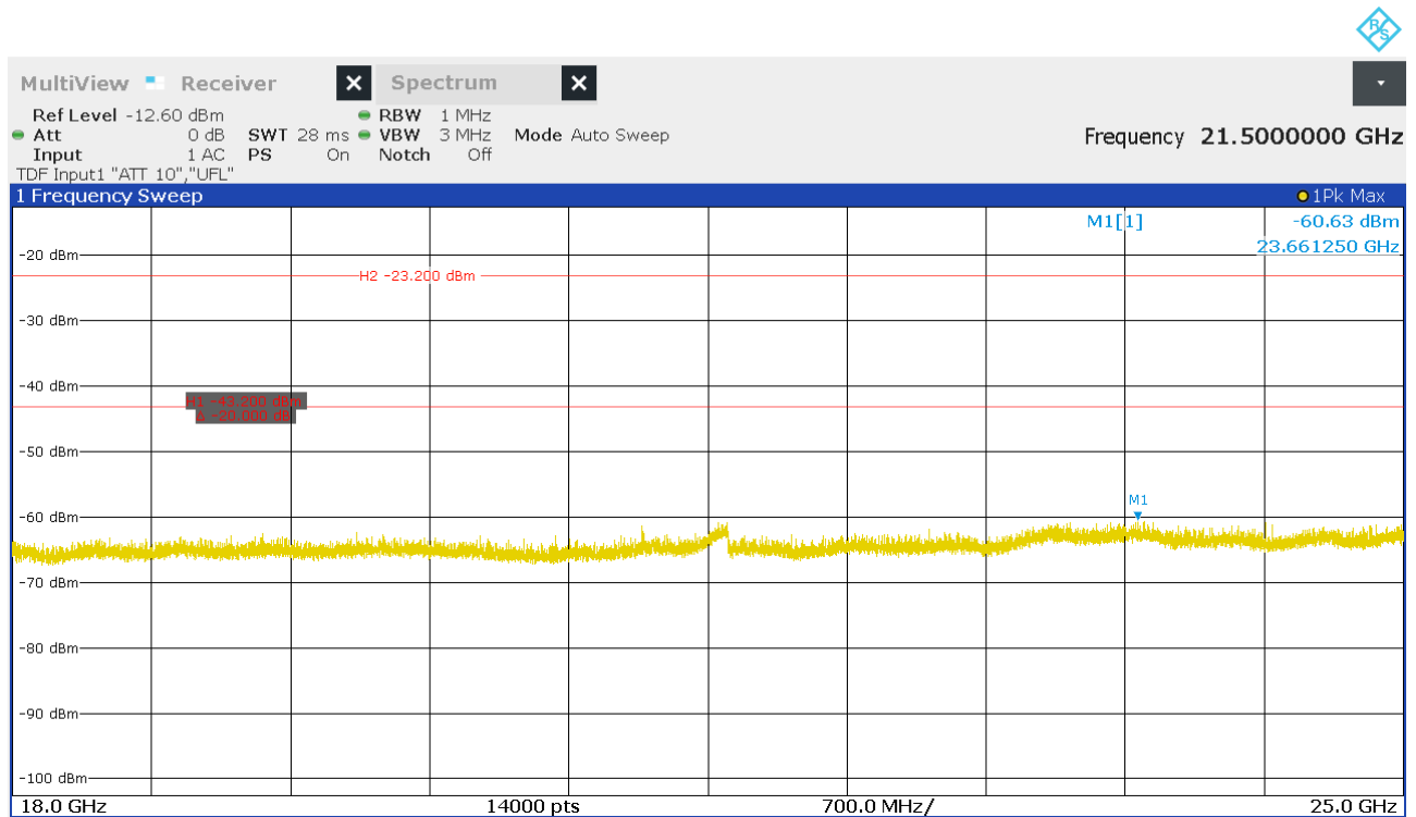
Figure 29: Chart of emissions test from 18 GHz to 25 GHz on middle channel, Pk
