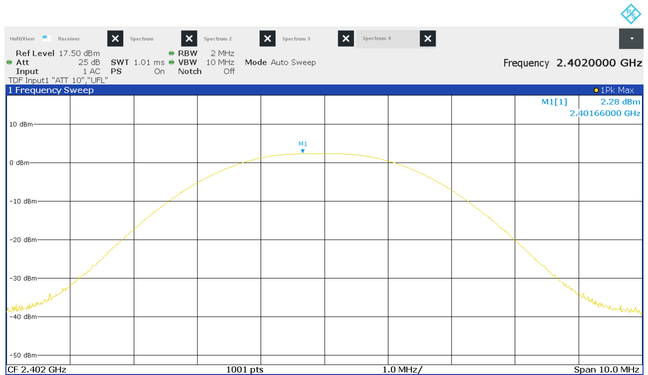
Figure 13: Chart of conducted output power on lowest channel
