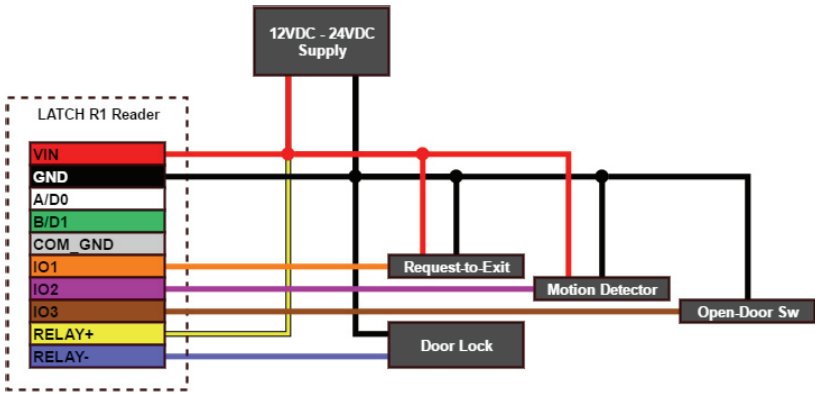
EXAMPLE 1 Stand-Alone Operation – No Panel – Wi-Fi/BLE/Ethern et Credential Sync.
