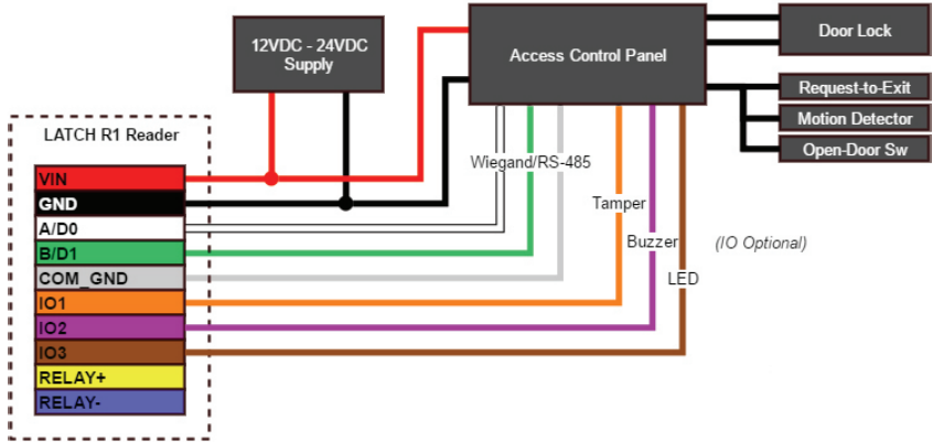
EXAMPLE 2 Reader Function Only – RS-485 or Wiegand Panel Comms – WiFi/BLE/Ethernet Credential Sync.
