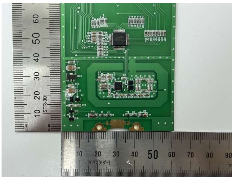
Antenna Bottom View [With Ruler]
