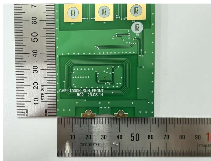
Antenna Top View [With Ruler]
