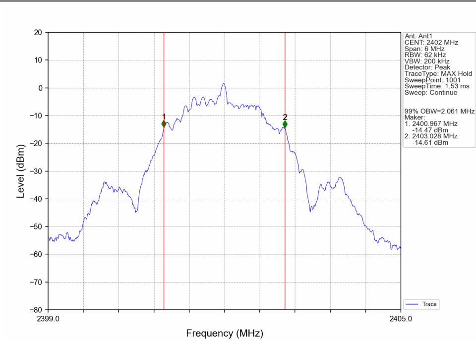
2M_LCH_2402MHz_Ant1_NTNV
