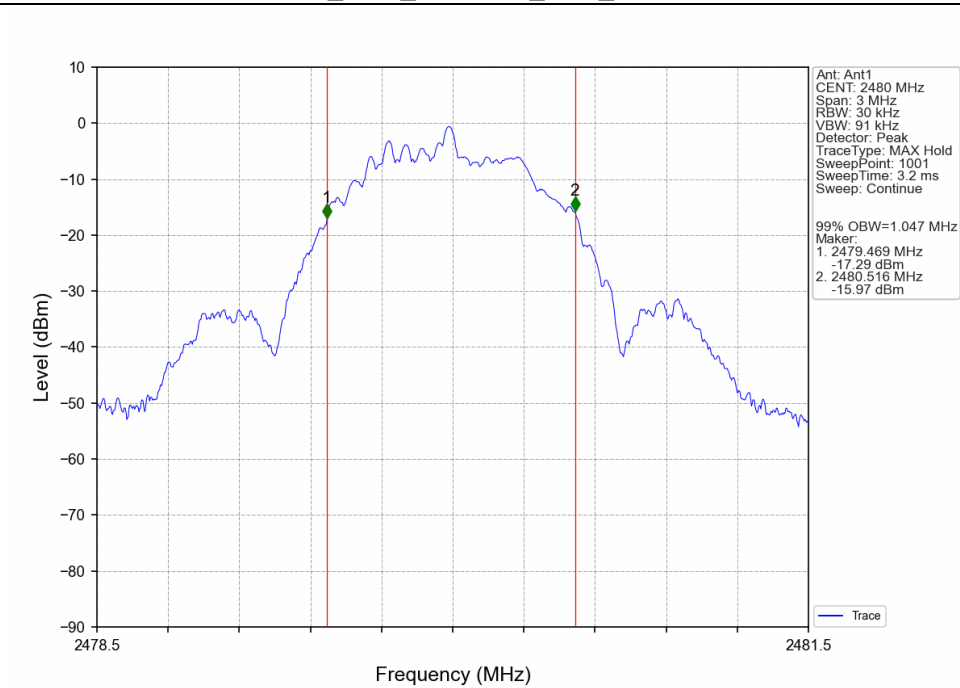
1M_HCH_2480MHz_Ant1_NTNV
