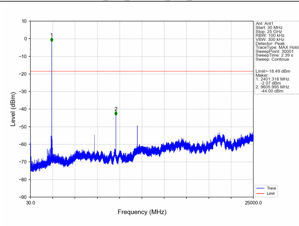
2M_LCH_2402MHz_Ant1_NTNV
