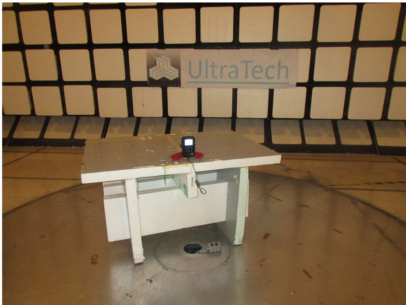
Tx Radiated Emissions at 3 m Orthogonal Position 1
