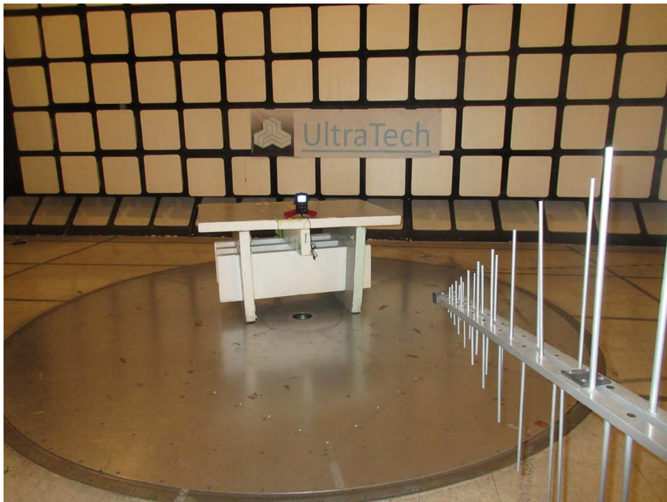
Tx Radiated Emissions at 3 m (30 MHz to 1 GHz) Orthogonal Position 1
