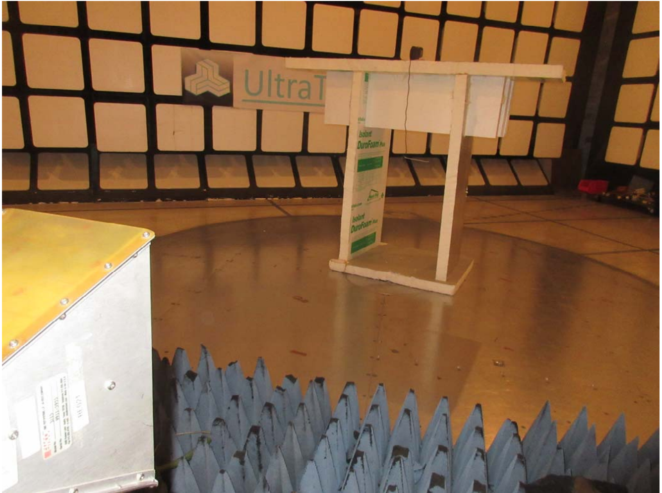
Tx Radiated Emissions at 3 m (Above 1 GHz) Orthogonal Position 3
