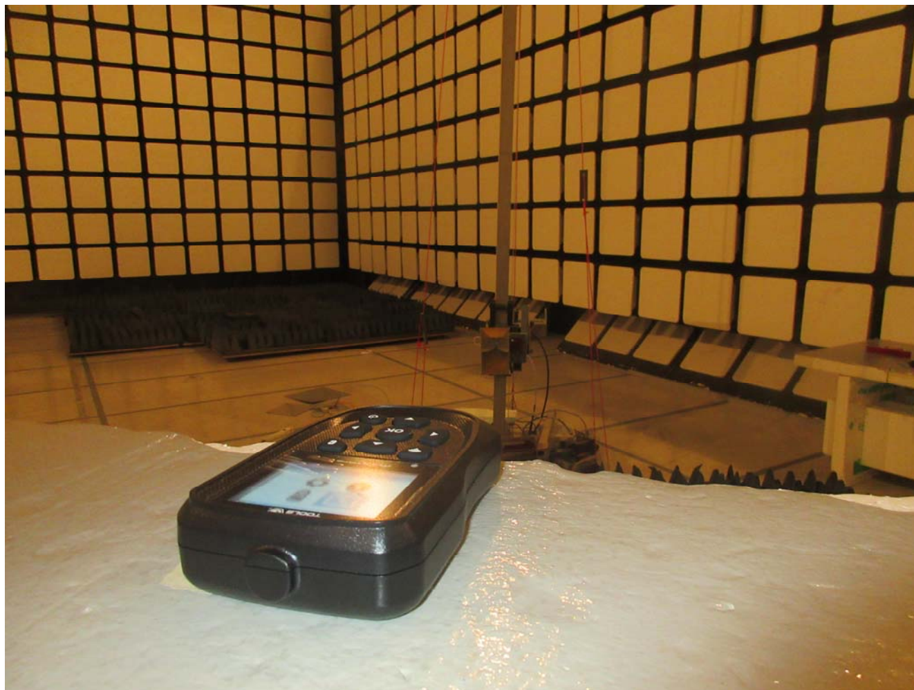
Tx Radiated Emissions at 3 m (Above 1 GHz) Orthogonal Position 2
