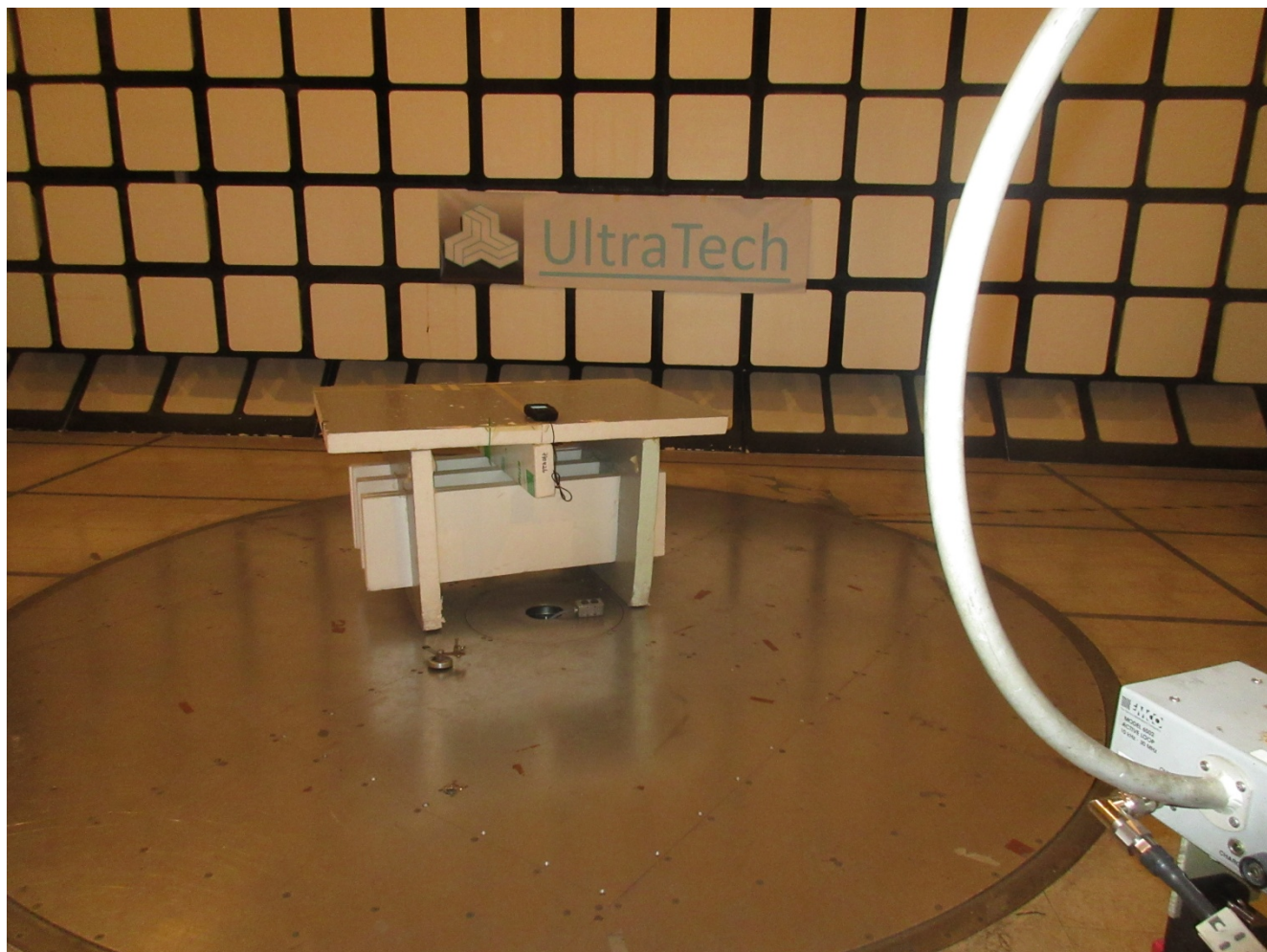
Tx Radiated Emissions at 3 m (Below 30 MHz) Orthogonal Position 2
