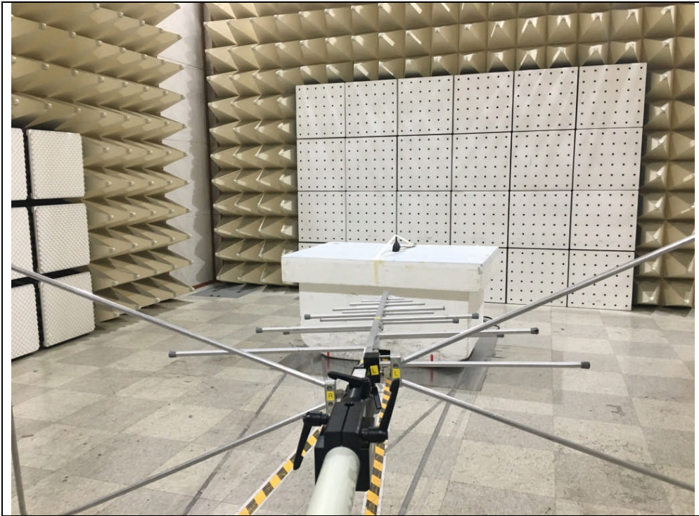
- Photo of Radiated Spurious Emission Test (Below 1 GHz)
