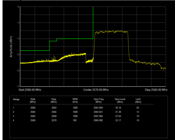
Band38 QPSK BW=5MHz Channel=37775 RB Size=1 Position=#Max Extended
