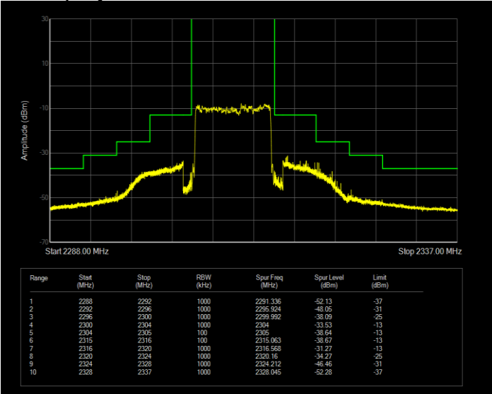
Band40(2305-2315) 16QAM BW=10MHz Channel=38750 RB Size=27 Position=#0 Extended
