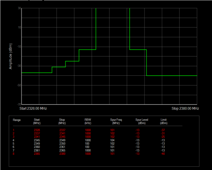
Band40(2350-2360) 16QAM BW=10MHz Channel=39200 RB Size=50 Position=#0 Extended
