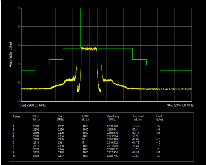
Band40(2305-2315) QPSK BW=5MHz Channel=38775 RB Size=25 Position=#0 Normal
