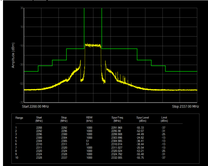
Band40(2305-2315) QPSK BW=10MHz Channel=38750 RB Size=1 Position=#0 Normal
