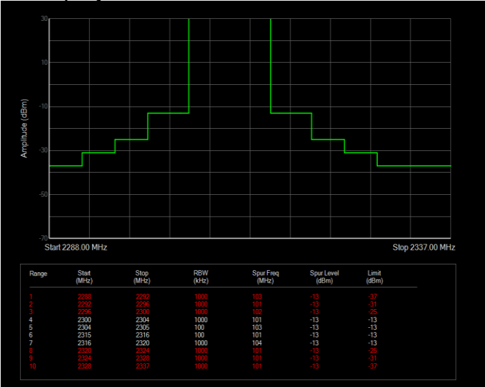
Band40(2305-2315) 16QAM BW=10MHz Channel=38750 RB Size=27 Position=#0 Normal
