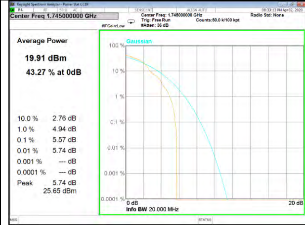
B66_1_QPSK_High
