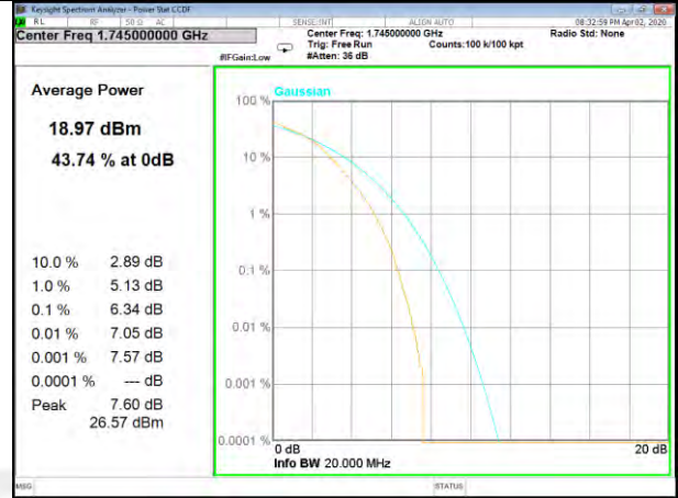
B66_100_QPSK_High
