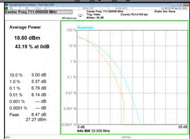
B12_50_Q16_High
