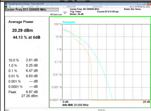
B26_1_QPSK_Middle
