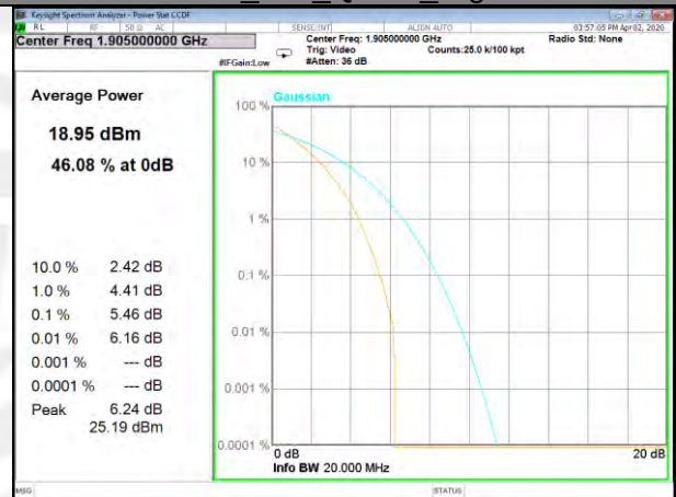
B25_100_Q16_High
