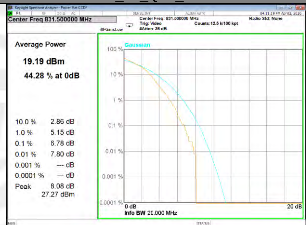
B26_50_QPSK_Middle
