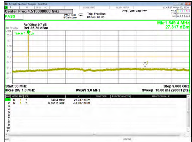
EGPRS_850_Higher_Conducted Spurious
