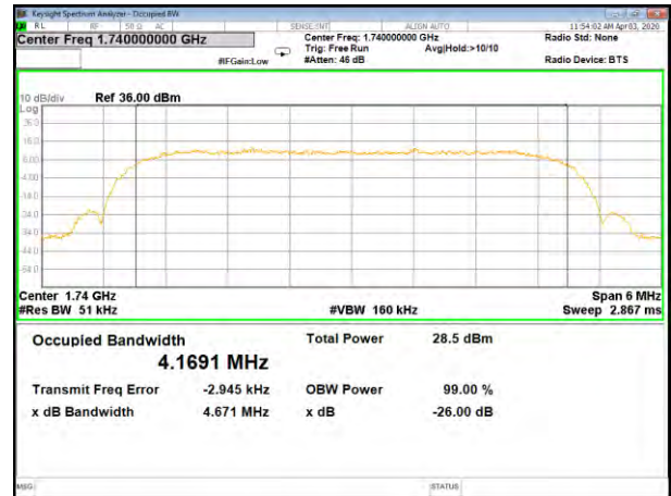
HSUPA B4_26BW and 99%_Middle
