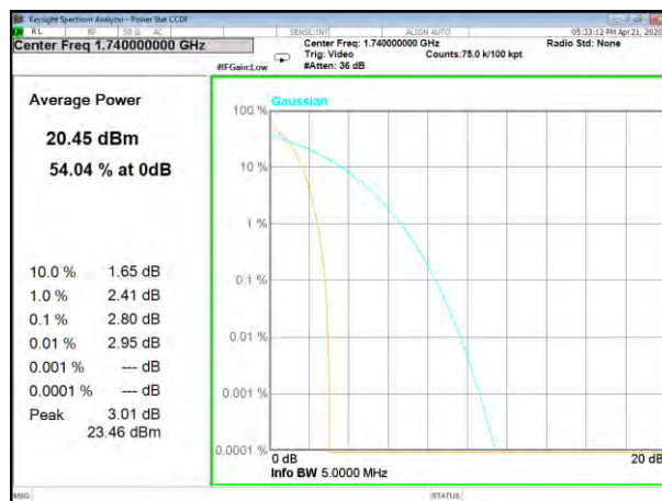
WCDMA B4_Middle
