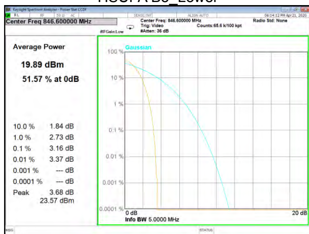
HSPA B5_Higher
