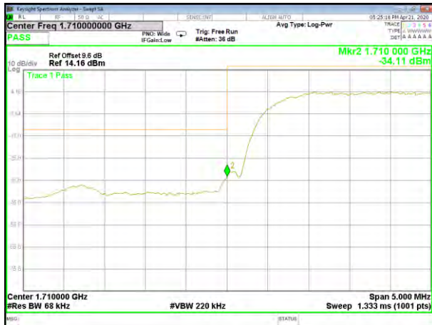
WCDMA B4_Band edge_Low
