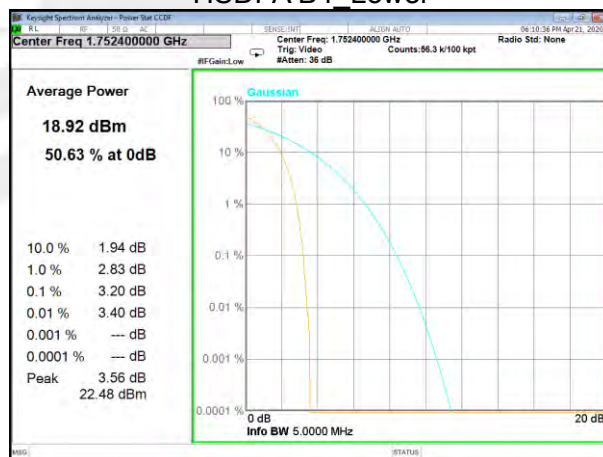
HSDPA B4_Higher
