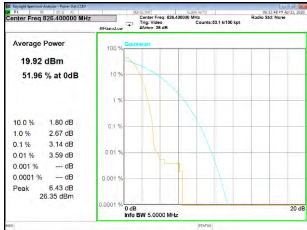
HSPA B5_Lower
