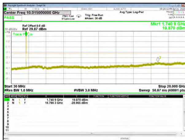
WCDMA B4_Conducted Spurious_Middle
