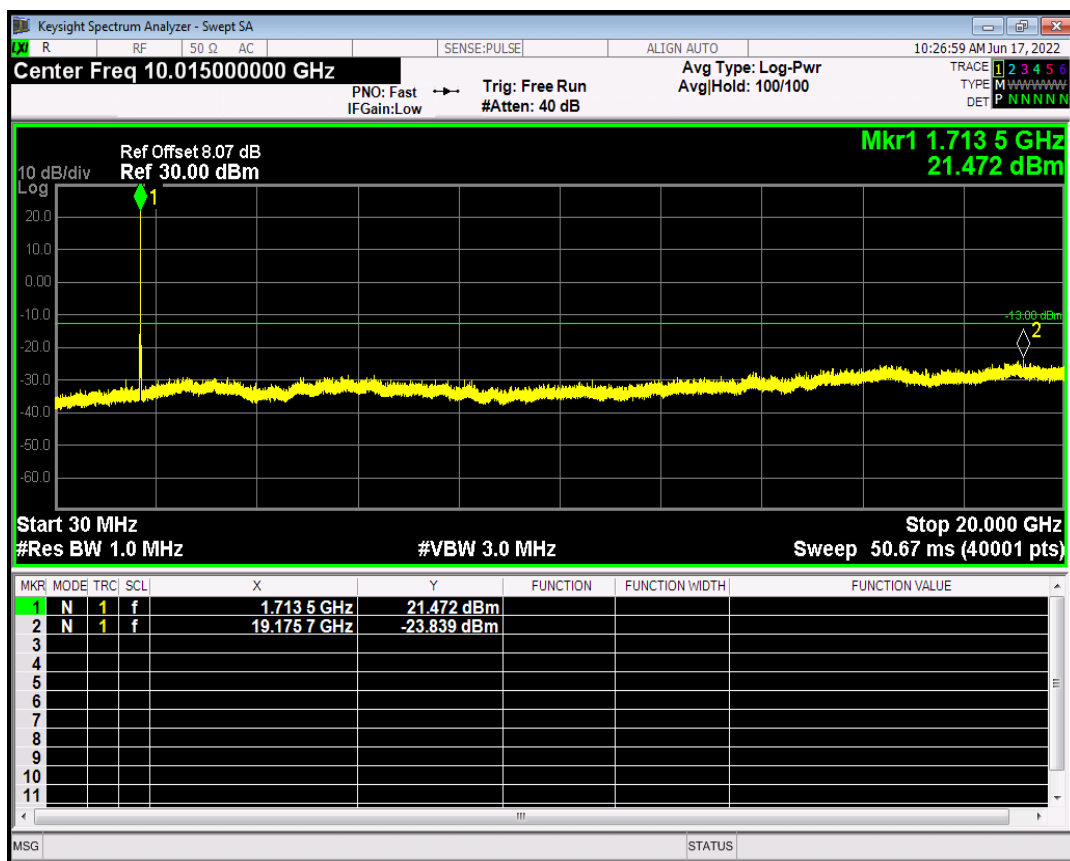
HSUPA Band4 Subtest5 Channel=1450
