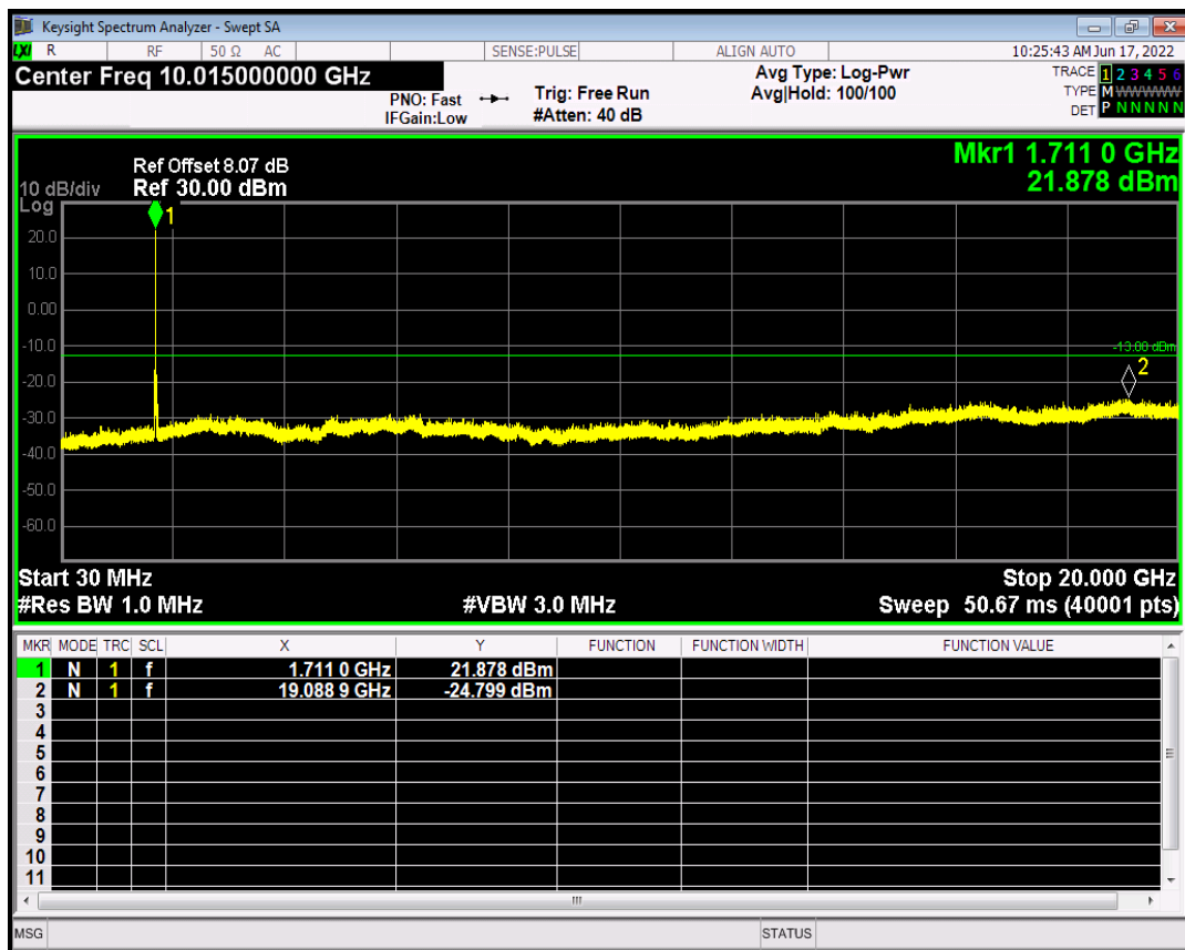
HSUPA Band4 Subtest2 Channel=1450
