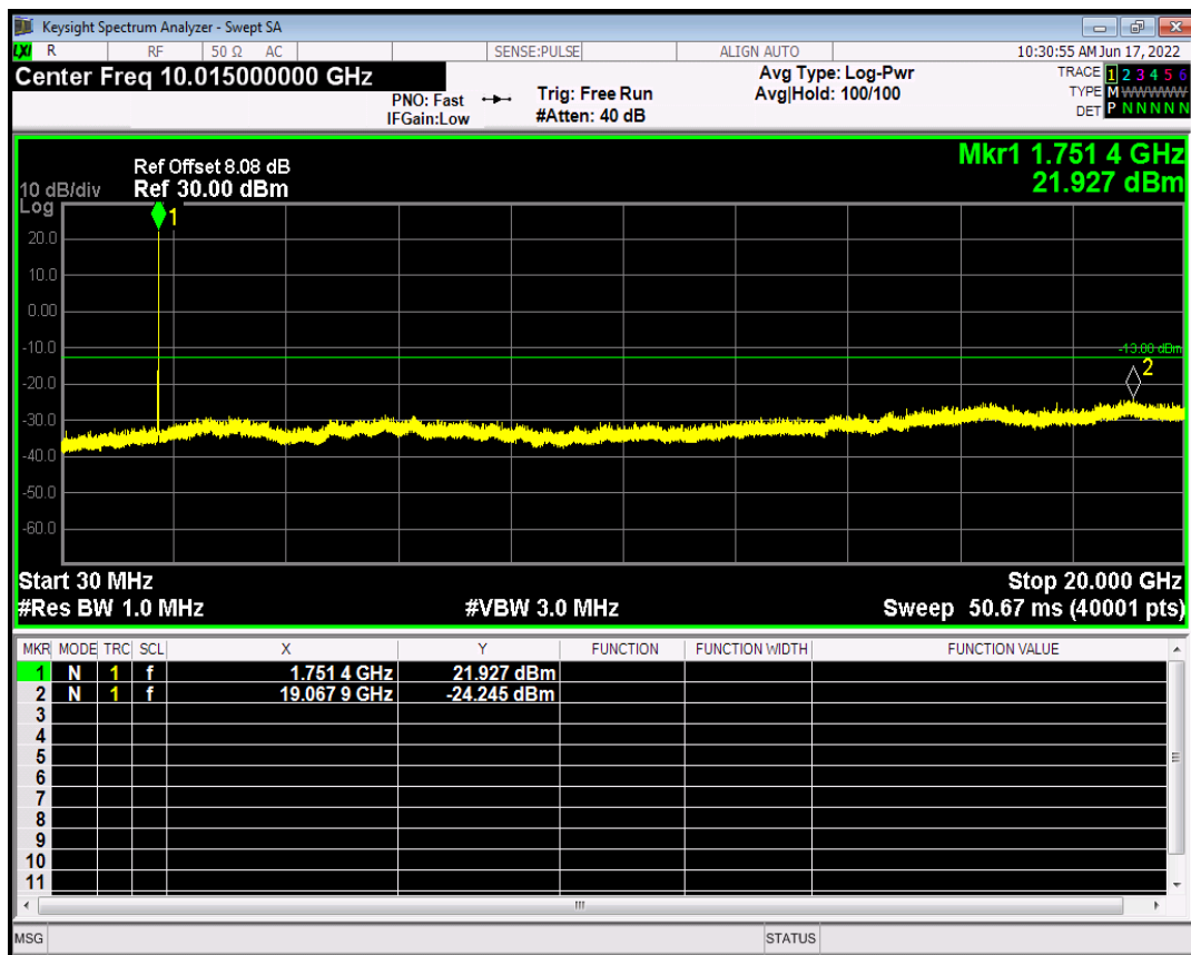
HSUPA Band4 Subtest5 Channel=1312
