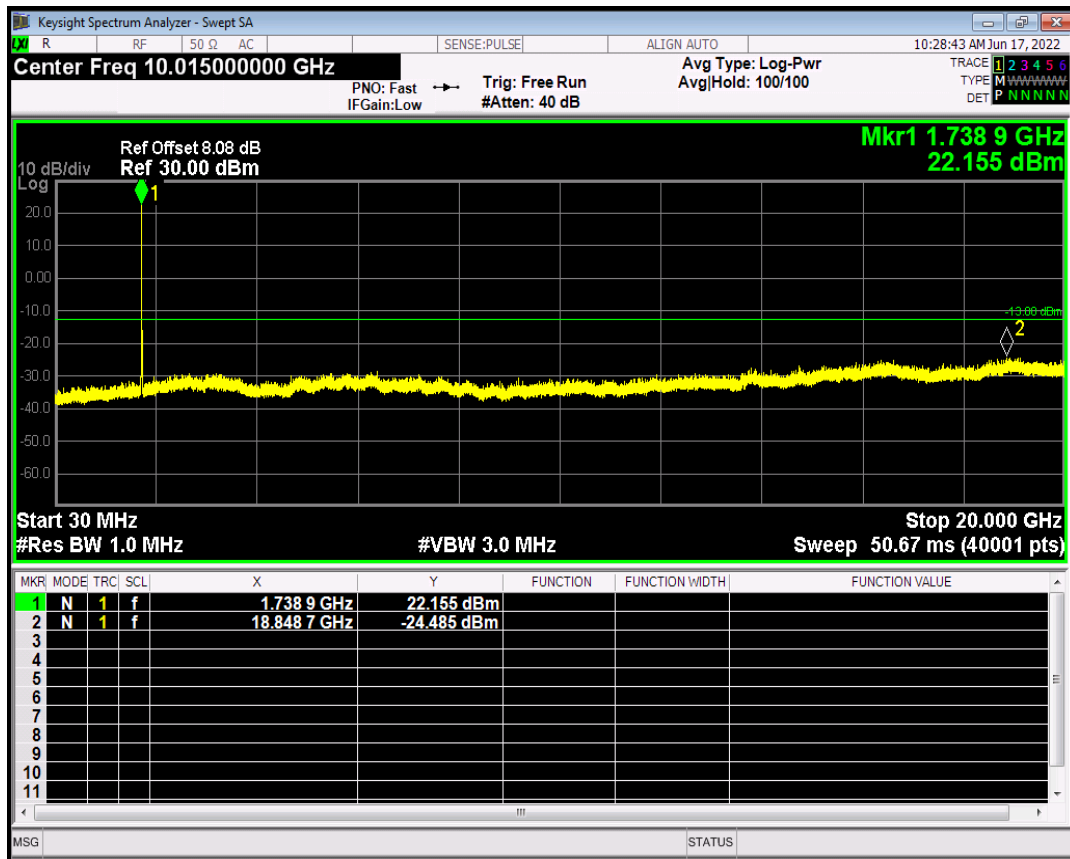
HSUPA Band4 Subtest4 Channel=1513
