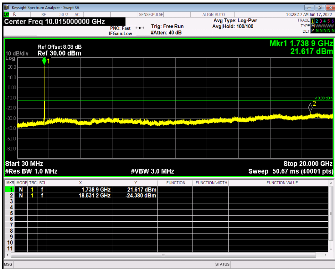
HSUPA Band4 Subtest3 Channel=1513
