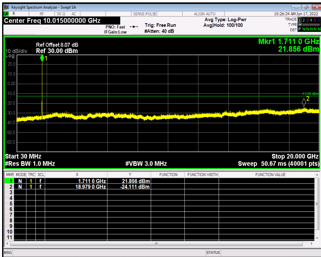
HSUPA Band4 Subtest4 Channel=1450
