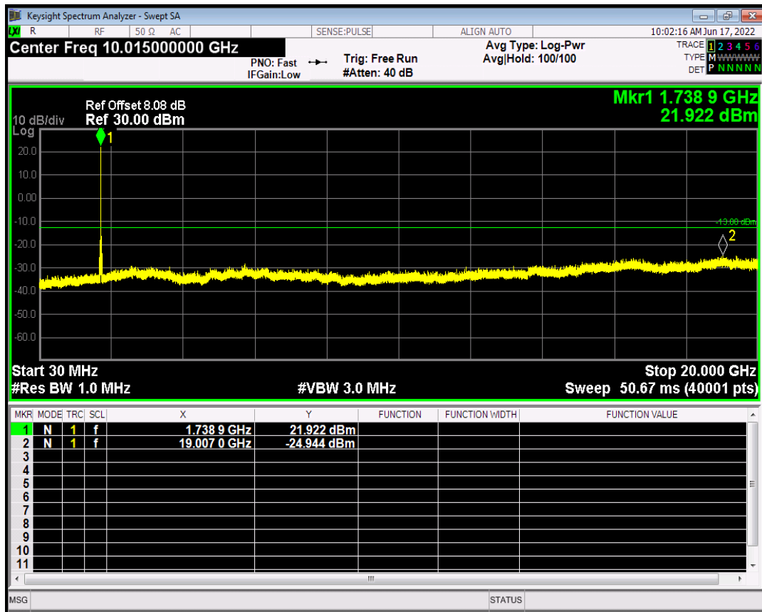
HSDPA Band4 Subtest4 Channel=1513
