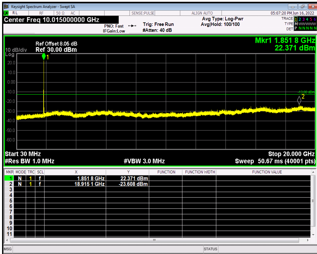
HSUPA Band2 Subtest3 Channel=9400
