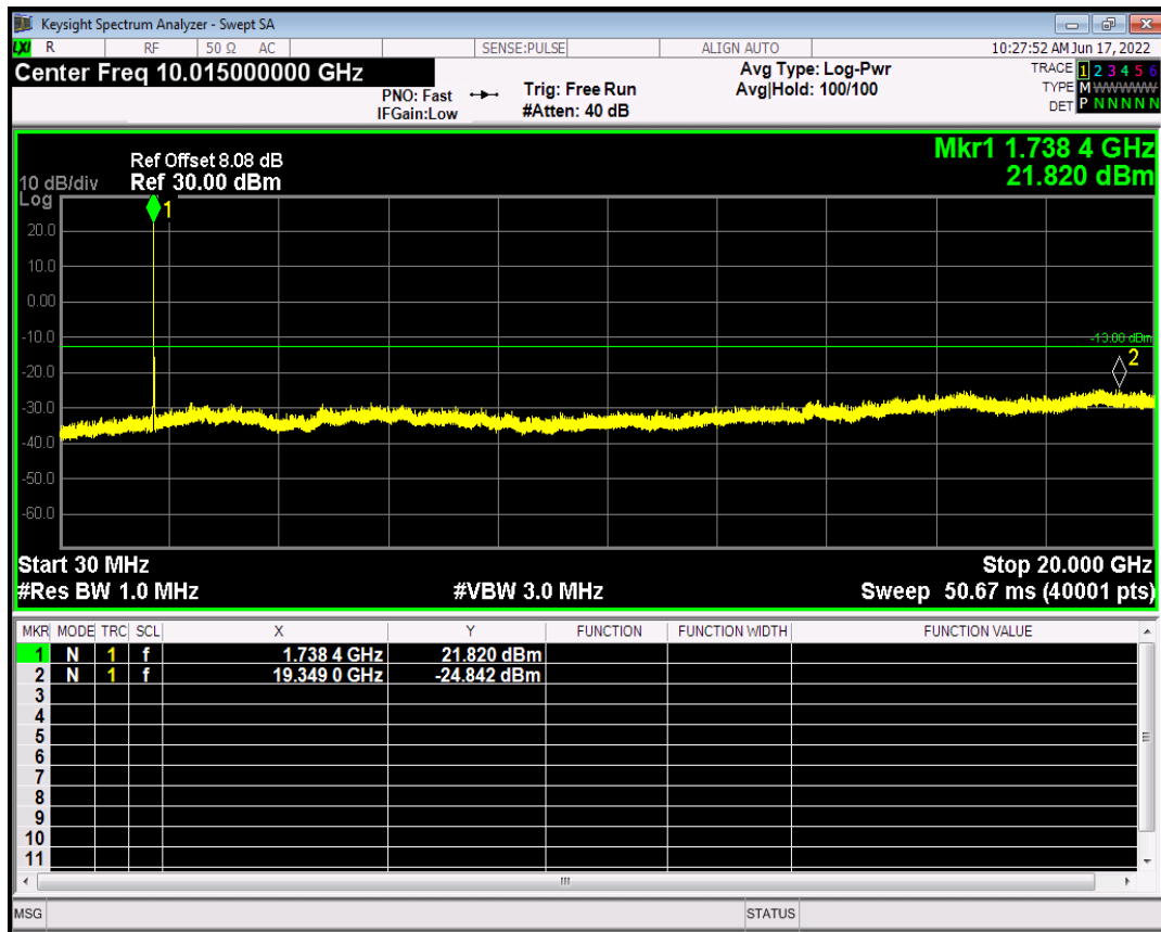
HSUPA Band4 Subtest2 Channel=1513
