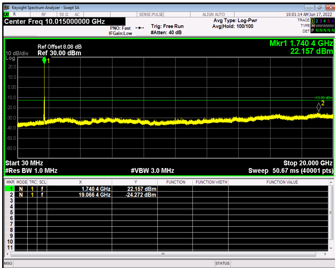
HSDPA Band4 Subtest3 Channel=1513
