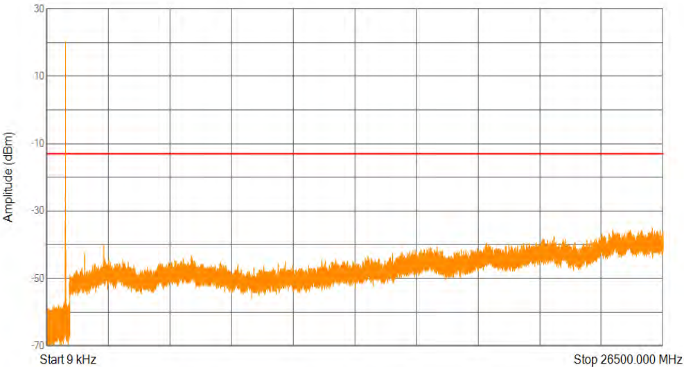
Band26(821-824) QAM16 BW=1.4MHz Channel=26783 RB Size=6 Position=#0
