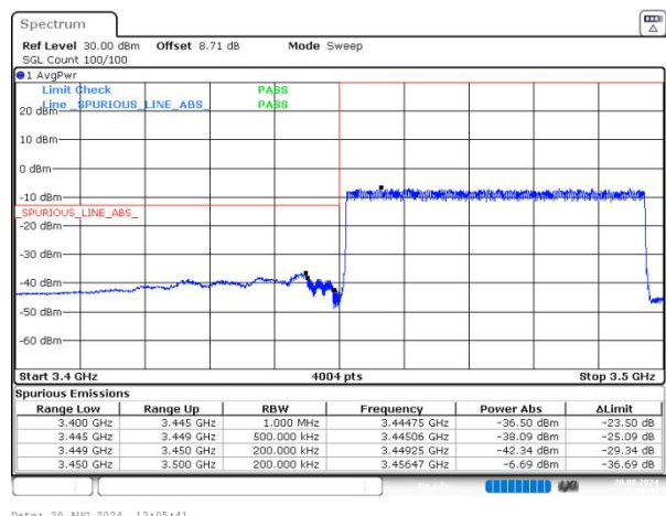
n77(3450-3550) SCS=30kHz DFT_64QAM BW=50MHz LowChannel=631668 RB=128@0 NVNT
