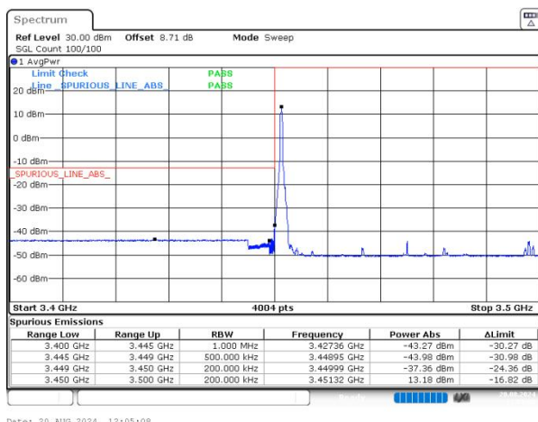
n77(3450-3550) SCS=30kHz DFT_64QAM BW=50MHz LowChannel=631668 RB=1@0 NVNT
