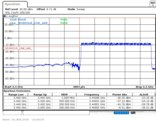
n77(3450-3550) SCS=30kHz DFT_16QAM BW=50MHz LowChannel=631668 RB=128@0 NVNT
