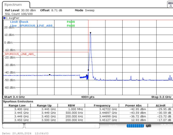
n77(3450-3550) SCS=30kHz DFT_16QAM BW=50MHz LowChannel=631668 RB=1@0 NVNT
