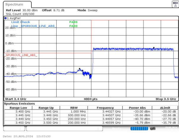
n77(3450-3550) SCS=30kHz DFT_QPSK BW=50MHz LowChannel=631668 RB=128@0 NVNT
