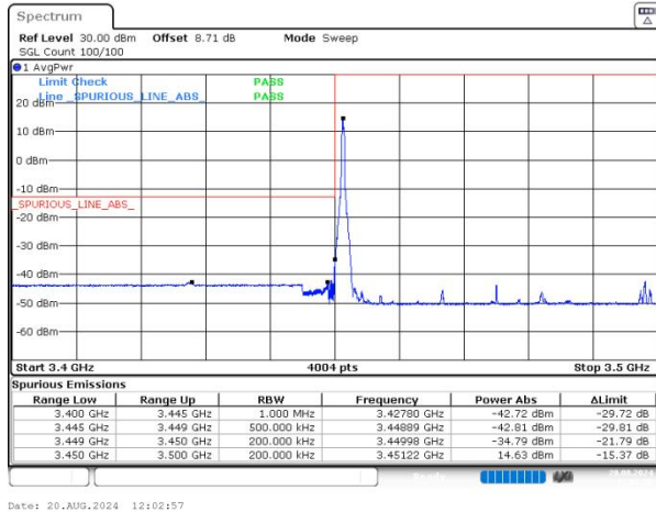
n77(3450-3550) SCS=30kHz DFT_QPSK BW=50MHz LowChannel=631668 RB=1@0 NVNT
