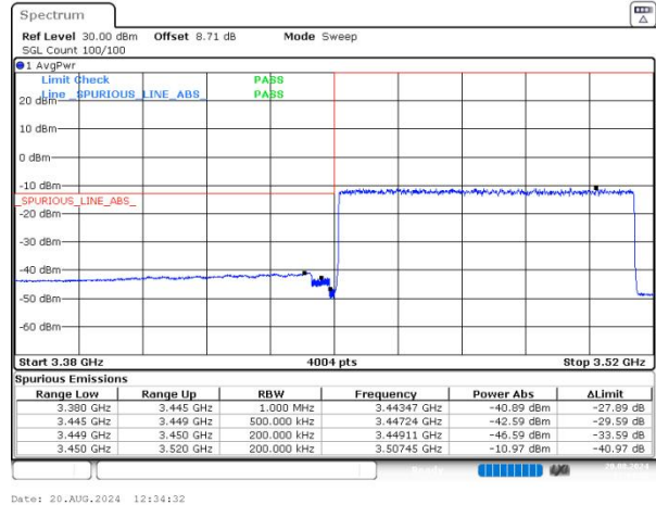
n77(3450-3550) SCS=30kHz DFT_256QAM BW=70MHz LowChannel=632334 RB=180@0 NVNT
