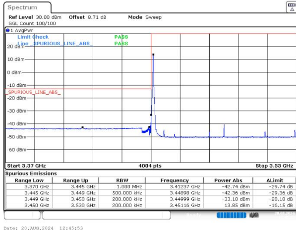
n77(3450-3550) SCS=30kHz DFT_QPSK BW=80MHz LowChannel=632668 RB=1@0 NVNT
