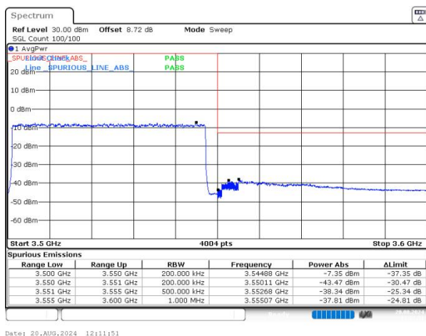
n77(3450-3550) SCS=30kHz DFT_64QAM BW=50MHz HighChannel=635000 RB=128@0 NVNT
