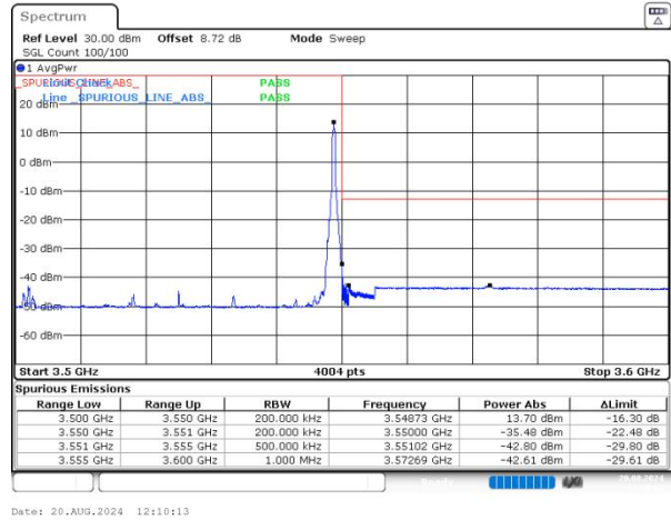
n77(3450-3550) SCS=30kHz DFT_16QAM BW=50MHz HighChannel=635000 RB=1@132 NVNT
