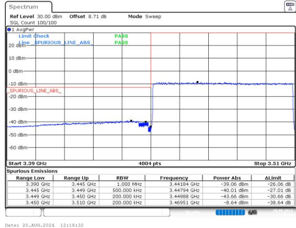
n77(3450-3550) SCS=30kHz DFT_64QAM BW=60MHz LowChannel=632000 RB=162@0 NVNT
