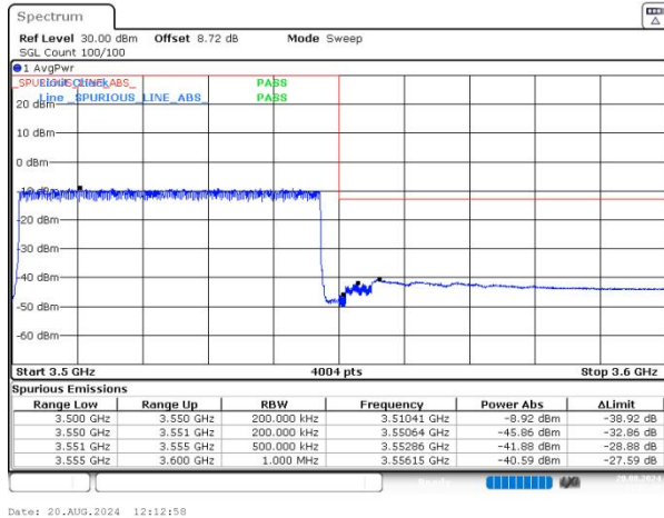
n77(3450-3550) SCS=30kHz DFT_256QAM BW=50MHz HighChannel=635000 RB=128@0 NVNT
