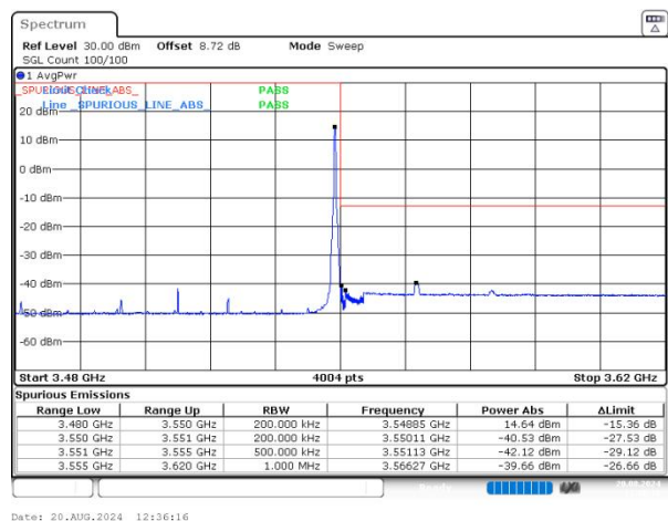
n77(3450-3550) SCS=30kHz DFT_BPSK BW=70MHz HighChannel=634332 RB=1@188 NVNT
