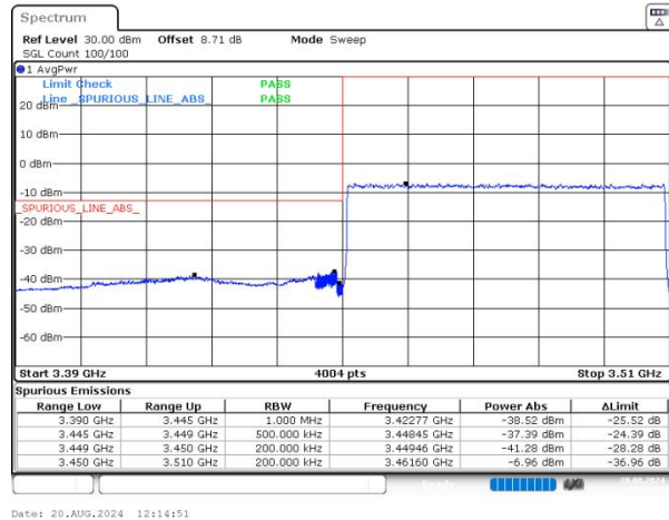
n77(3450-3550) SCS=30kHz DFT_BPSK BW=60MHz LowChannel=632000 RB=162@0 NVNT
