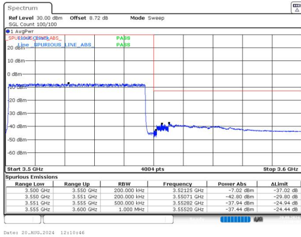
n77(3450-3550) SCS=30kHz DFT_16QAM BW=50MHz HighChannel=635000 RB=128@0 NVNT
