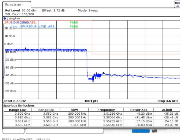
n77(3450-3550) SCS=30kHz DFT_QPSK BW=50MHz HighChannel=635000 RB=128@0 NVNT
