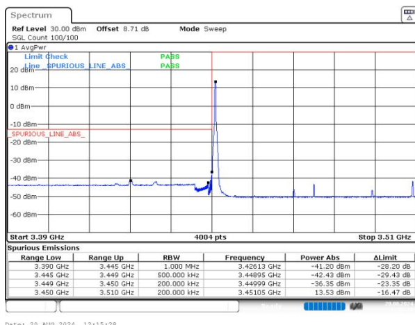
n77(3450-3550) SCS=30kHz DFT_QPSK BW=60MHz LowChannel=632000 RB=1@0 NVNT
