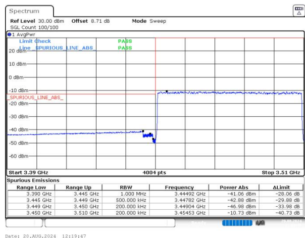
n77(3450-3550) SCS=30kHz DFT_256QAM BW=60MHz LowChannel=632000 RB=162@0 NVNT
