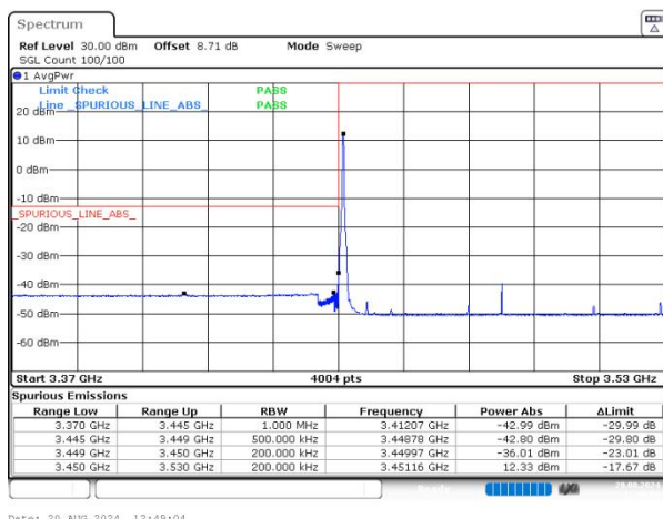
n77(3450-3550) SCS=30kHz DFT_64QAM BW=80MHz LowChannel=632668 RB=1@0 NVNT
