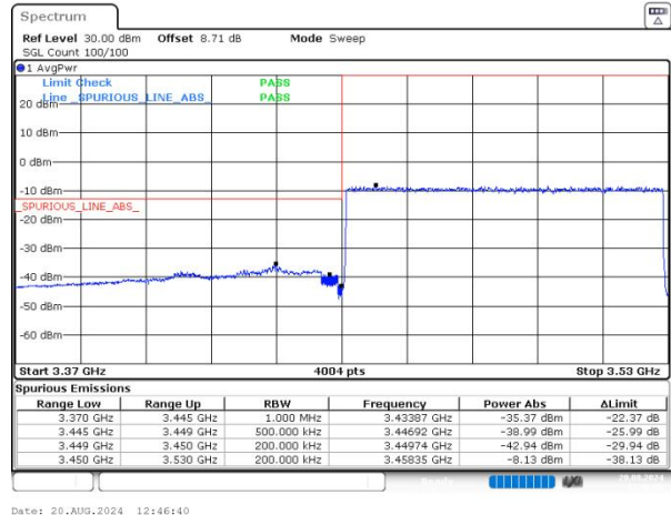
n77(3450-3550) SCS=30kHz DFT_QPSK BW=80MHz LowChannel=632668 RB=216@0 NVNT
