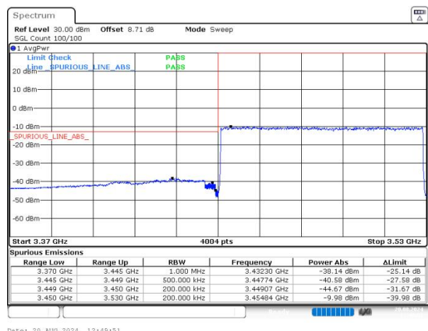
n77(3450-3550) SCS=30kHz DFT_64QAM BW=80MHz LowChannel=632668 RB=216@0 NVNT
