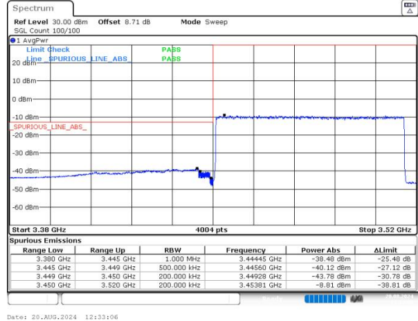
n77(3450-3550) SCS=30kHz DFT_64QAM BW=70MHz LowChannel=632334 RB=180@0 NVNT
