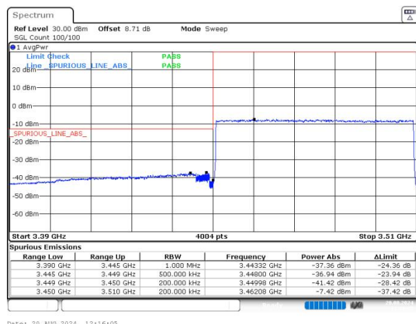
n77(3450-3550) SCS=30kHz DFT_QPSK BW=60MHz LowChannel=632000 RB=162@0 NVNT
