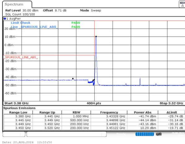
n77(3450-3550) SCS=30kHz DFT_256QAM BW=70MHz LowChannel=632334 RB=1@0 NVNT
