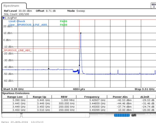
n77(3450-3550) SCS=30kHz DFT_256QAM BW=60MHz LowChannel=632000 RB=1@0 NVNT
