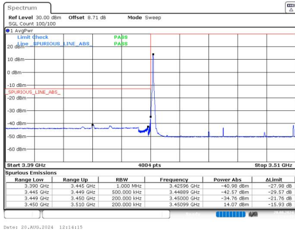
n77(3450-3550) SCS=30kHz DFT_BPSK BW=60MHz LowChannel=632000 RB=1@0 NVNT
