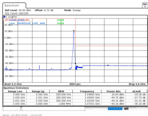
n77(3450-3550) SCS=30kHz DFT_256QAM BW=50MHz HighChannel=635000 RB=1@132 NVNT
