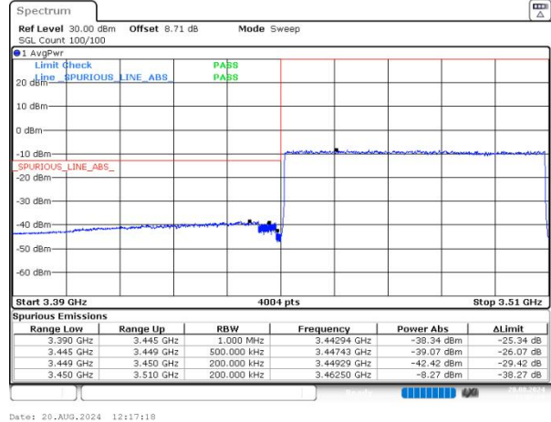
n77(3450-3550) SCS=30kHz DFT_16QAM BW=60MHz LowChannel=632000 RB=162@0 NVNT
