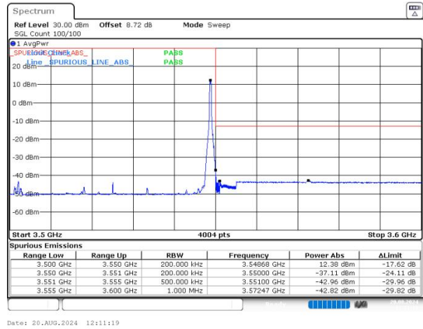
n77(3450-3550) SCS=30kHz DFT_64QAM BW=50MHz HighChannel=635000 RB=1@132 NVNT
