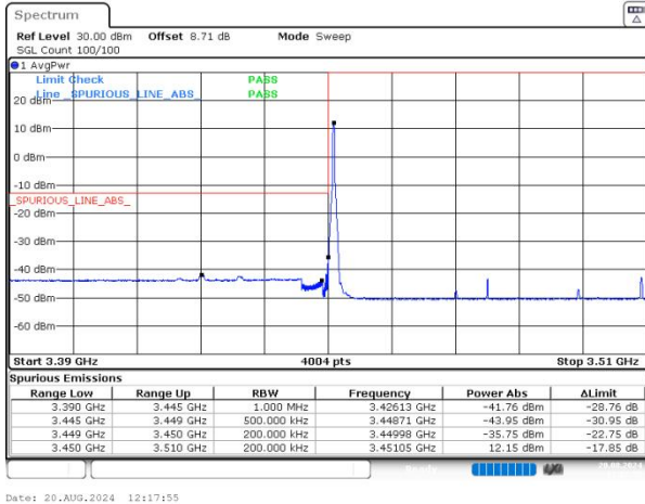
n77(3450-3550) SCS=30kHz DFT_64QAM BW=60MHz LowChannel=632000 RB=1@0 NVNT
