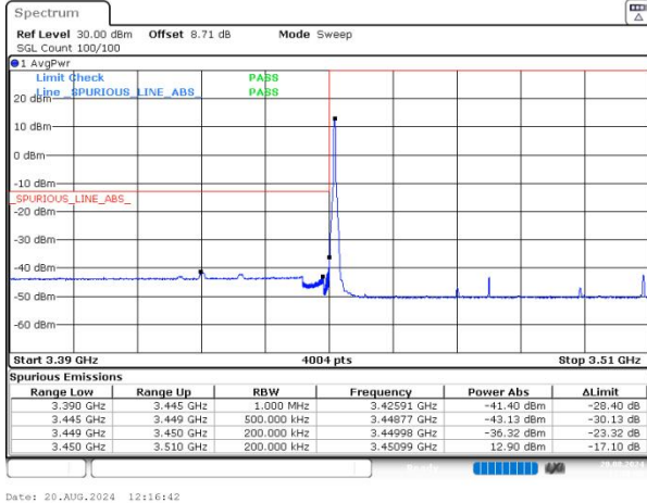
n77(3450-3550) SCS=30kHz DFT_16QAM BW=60MHz LowChannel=632000 RB=1@0 NVNT
