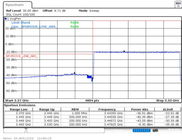
n77(3450-3550) SCS=30kHz DFT_16QAM BW=80MHz LowChannel=632668 RB=216@0 NVNT
