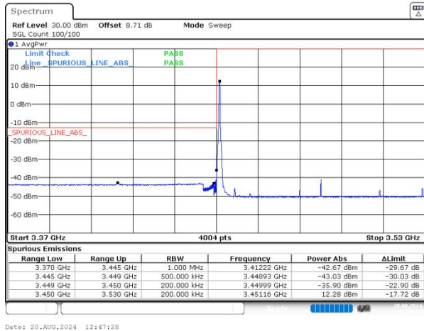
n77(3450-3550) SCS=30kHz DFT_16QAM BW=80MHz LowChannel=632668 RB=1@0 NVNT
