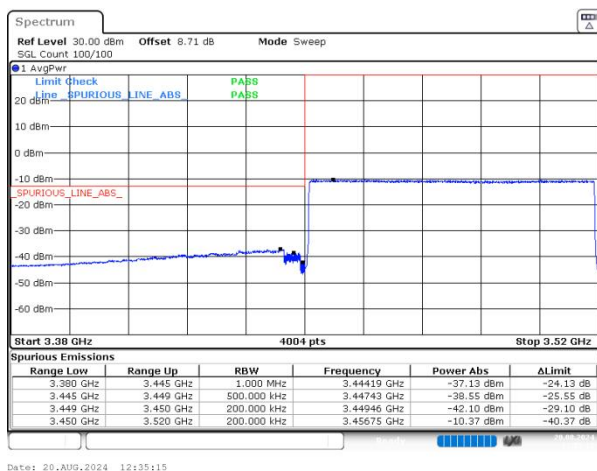
n77(3450-3550) SCS=30kHz CP_QPSK BW=70MHz LowChannel=632334 RB=189@0 NVNT
