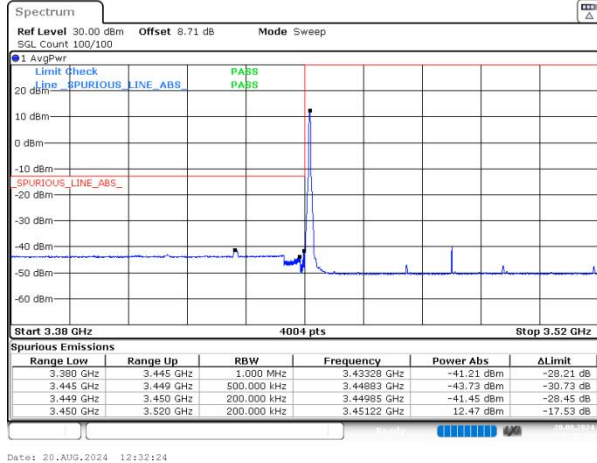
n77(3450-3550) SCS=30kHz DFT_64QAM BW=70MHz LowChannel=632334 RB=1@0 NVNT
