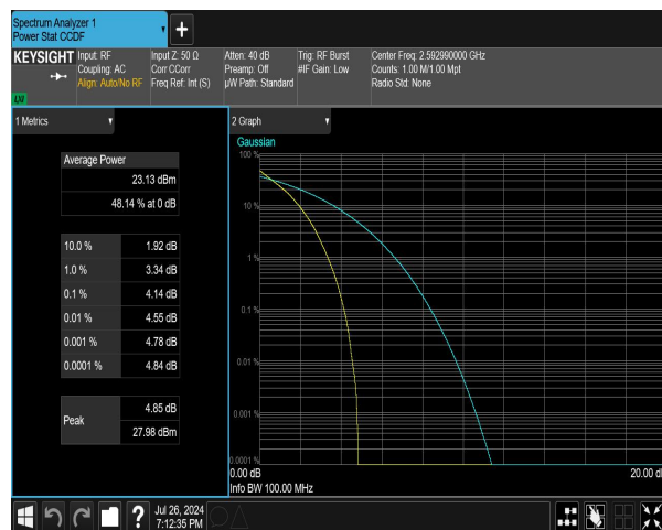
n41 SCS=30kHz DFT_BPSK BW=30MHz Channel=518598 RB=75@0 NVNT
