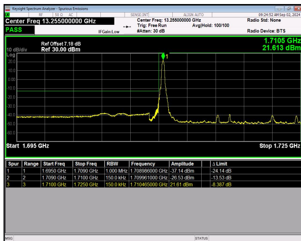
n66 SCS=15kHz DFT_BPSK BW=15MHz LowChannel=343500 RB=1@0 NVNT
