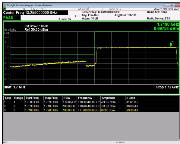
n66 SCS=15kHz CP_QPSK BW=10MHz LowChannel=343000 RB=52@0 NVNT
