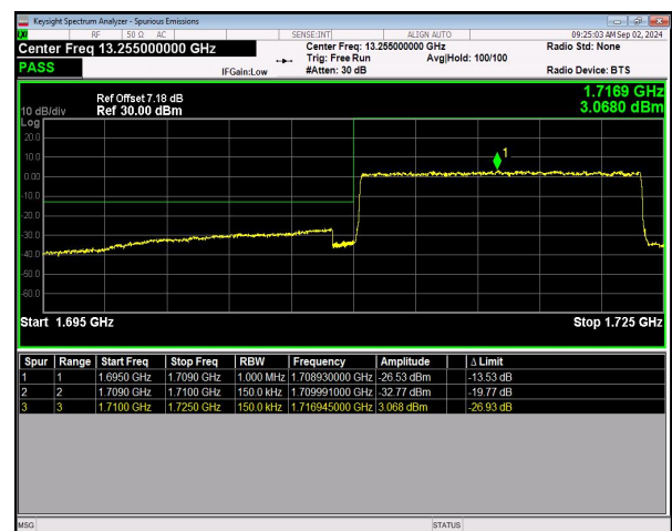
n66 SCS=15kHz DFT_QPSK BW=15MHz LowChannel=343500 RB=75@0 NVNT
