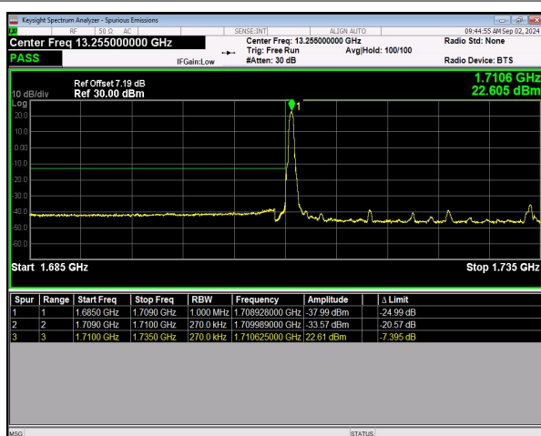
n66 SCS=15kHz DFT_BPSK BW=25MHz LowChannel=344500 RB=1@0 NVNT
