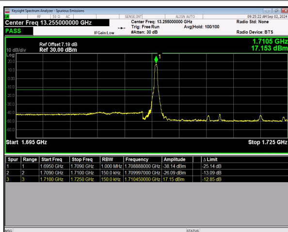
n66 SCS=15kHz DFT_256QAM BW=15MHz LowChannel=343500 RB=1@0 NVNT
