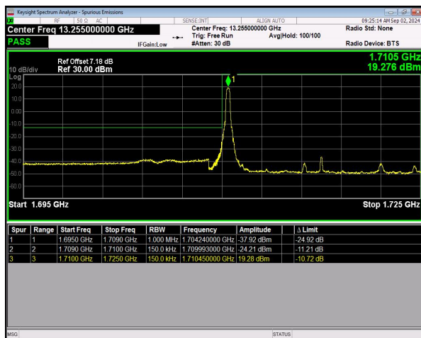
n66 SCS=15kHz DFT_64QAM BW=15MHz LowChannel=343500 RB=1@0 NVNT
