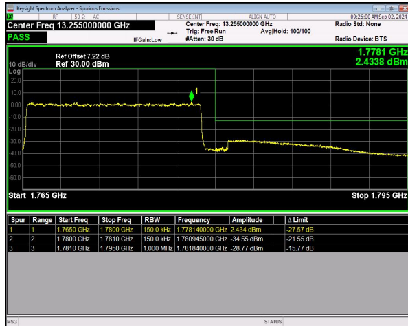
n66 SCS=15kHz DFT_16QAM BW=15MHz HighChannel=354500 RB=75@0 NVNT
