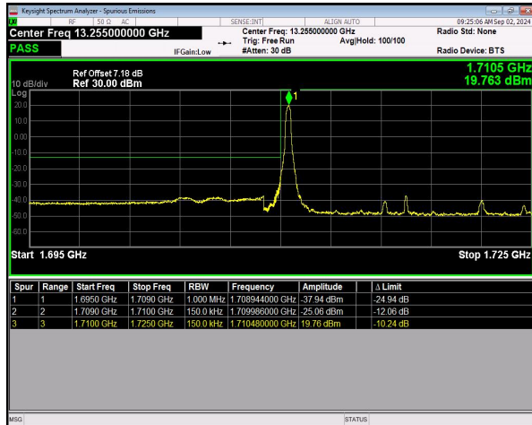
n66 SCS=15kHz DFT_16QAM BW=15MHz LowChannel=343500 RB=1@0 NVNT
