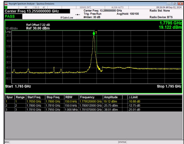
n66 SCS=15kHz DFT_64QAM BW=15MHz HighChannel=354500 RB=1@78 NVNT
