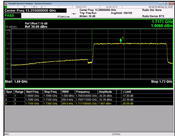
n66 SCS=15kHz DFT_64QAM BW=20MHz LowChannel=344000 RB=100@0 NVNT
