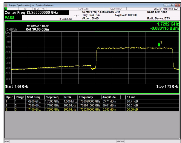
n66 SCS=15kHz DFT_256QAM BW=20MHz LowChannel=344000 RB=100@0 NVNT
