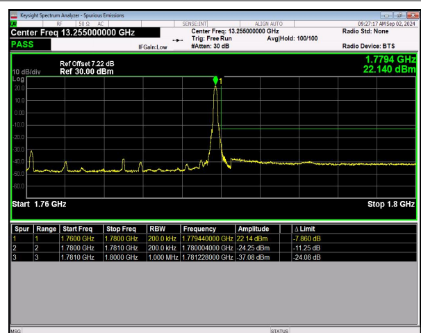
n66 SCS=15kHz DFT_BPSK BW=20MHz HighChannel=354000 RB=1@105 NVNT
