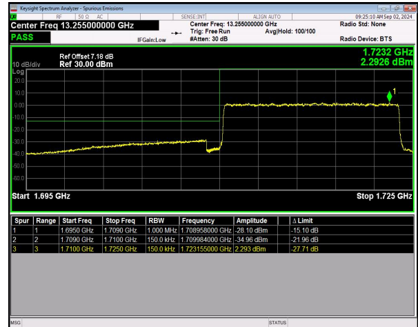
n66 SCS=15kHz DFT_16QAM BW=15MHz LowChannel=343500 RB=75@0 NVNT
