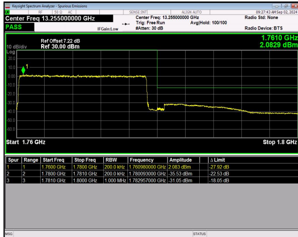
n66 SCS=15kHz DFT_64QAM BW=20MHz HighChannel=354000 RB=100@0 NVNT
