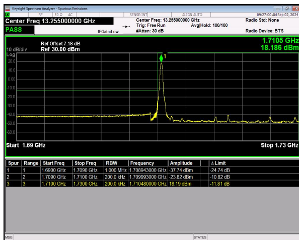
n66 SCS=15kHz DFT_256QAM BW=20MHz LowChannel=344000 RB=1@0 NVNT
