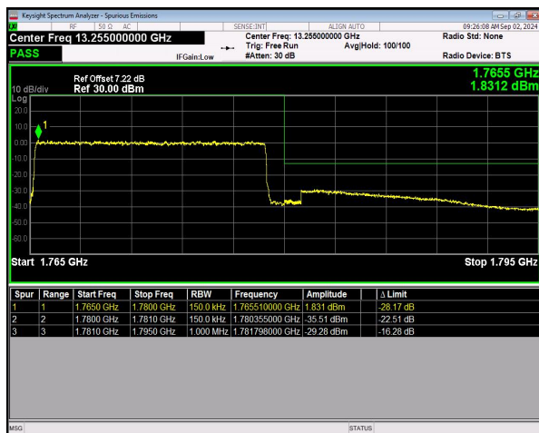
n66 SCS=15kHz DFT_64QAM BW=15MHz HighChannel=354500 RB=75@0 NVNT
