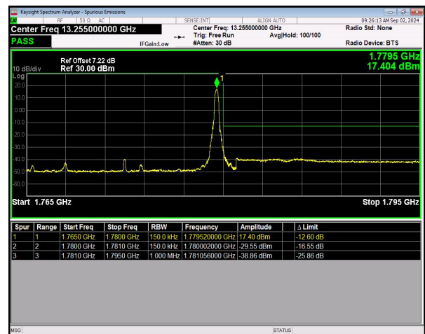
n66 SCS=15kHz DFT_256QAM BW=15MHz HighChannel=354500 RB=1@78 NVNT
