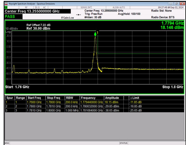
n66 SCS=15kHz DFT_256QAM BW=20MHz HighChannel=354000 RB=1@105 NVNT
