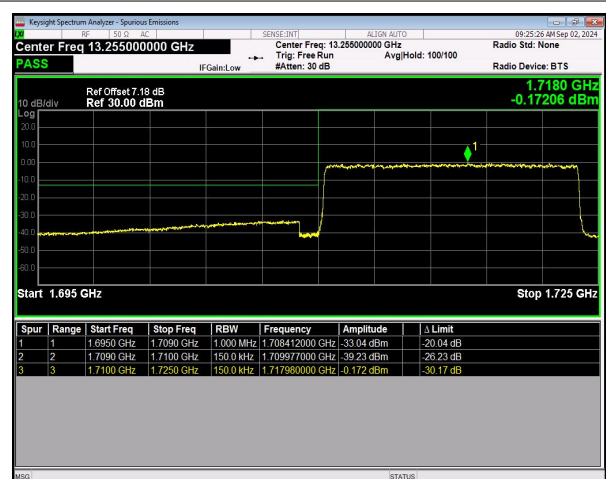
n66 SCS=15kHz DFT_256QAM BW=15MHz LowChannel=343500 RB=75@0 NVNT
