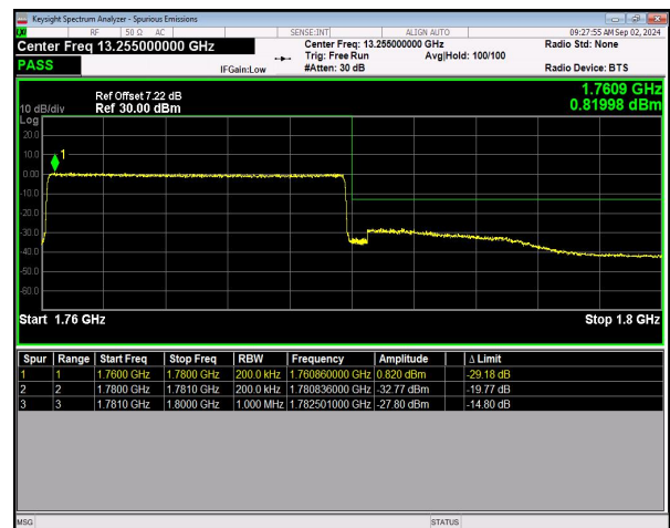
n66 SCS=15kHz CP_QPSK BW=20MHz HighChannel=354000 RB=106@0 NVNT
