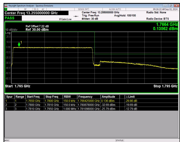
n66 SCS=15kHz CP_QPSK BW=15MHz HighChannel=354500 RB=79@0 NVNT
