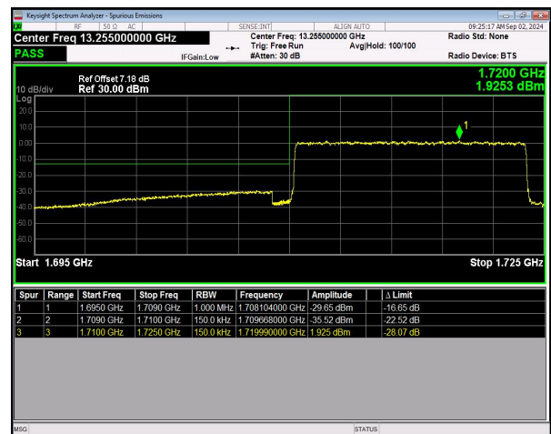
n66 SCS=15kHz DFT_64QAM BW=15MHz LowChannel=343500 RB=75@0 NVNT
