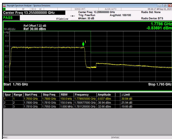
n66 SCS=15kHz DFT_256QAM BW=15MHz HighChannel=354500 RB=75@0 NVNT
