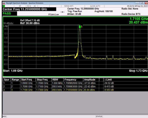
n66 SCS=15kHz DFT_64QAM BW=20MHz LowChannel=344000 RB=1@0 NVNT
