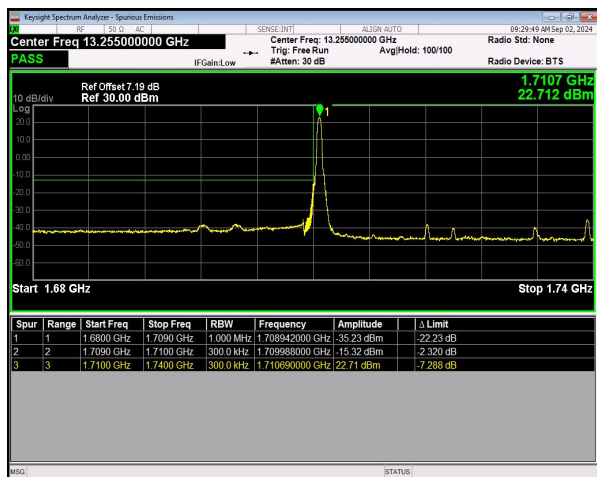
n66 SCS=15kHz DFT_BPSK BW=30MHz LowChannel=345000 RB=1@0 NVNT
