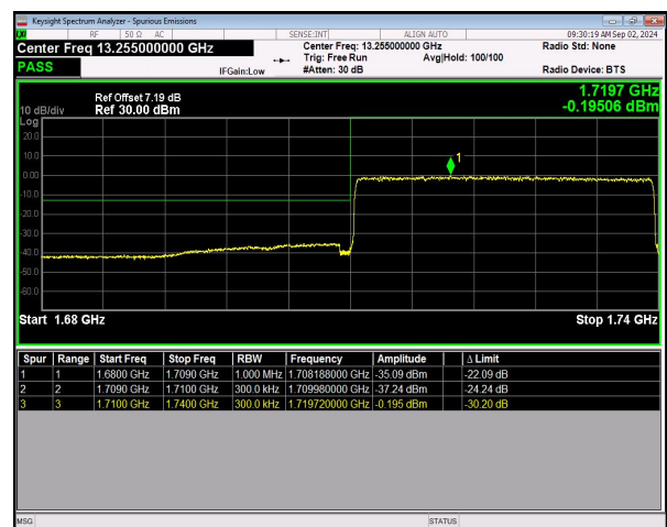
n66 SCS=15kHz DFT_256QAM BW=30MHz LowChannel=345000 RB=160@0 NVNT
