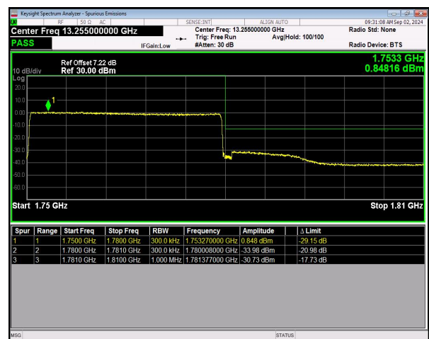
n66 SCS=15kHz CP_QPSK BW=30MHz HighChannel=353000 RB=160@0 NVNT
