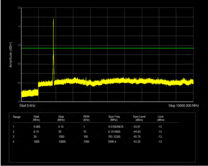
Band25 QAM16 BW=20MHz Channel=26590 RB Size=100 Position=#0
