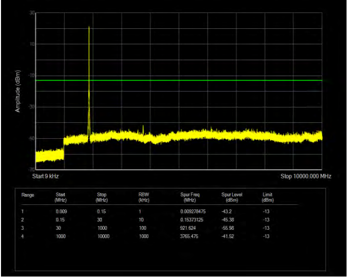
Band25 QAM16 BW=10MHz Channel=26640 RB Size=50 Position=#0
