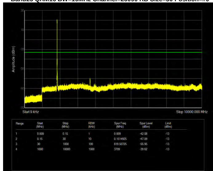
Band25 QAM16 BW=10MHz Channel=26090 RB Size=50 Position=#0
