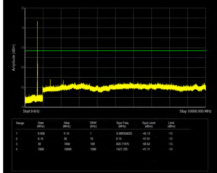
Band25 QAM16 BW=1.4MHz Channel=26047 RB Size=6 Position=#0
