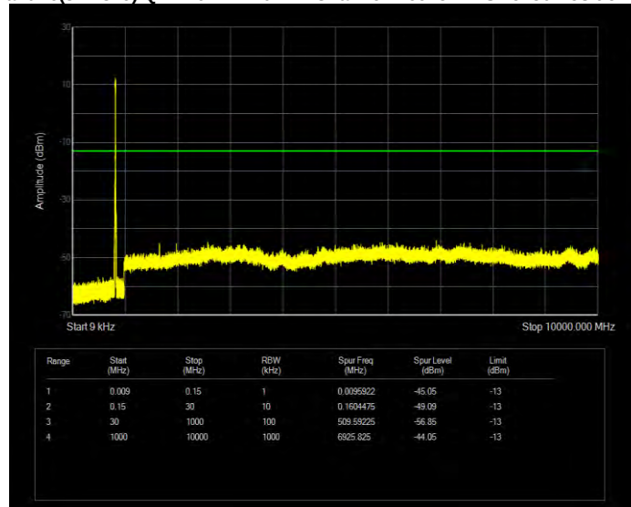
Band26(824-849) QAM16 BW=10MHz Channel=26990 RB Size=50 Position=#0
