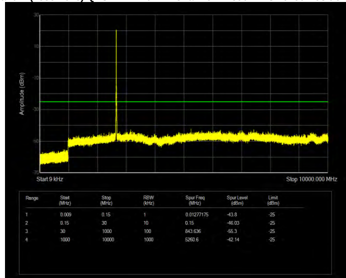
Band41(2535-2675) QPSK BW=15MHz Channel=40115 RB Size=75 Position=#0
