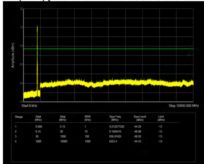
Band26(824-849) QAM16 BW=15MHz Channel=26965 RB Size=75 Position=#0
