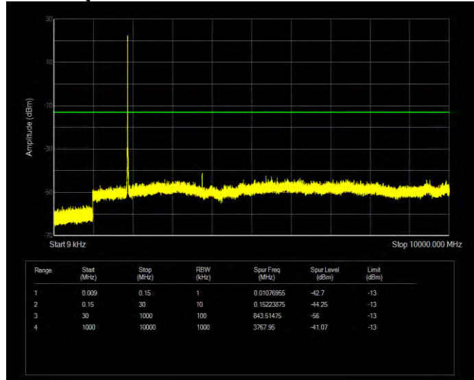
Band25 QAM16 BW=5MHz Channel=26665 RB Size=25 Position=#0
