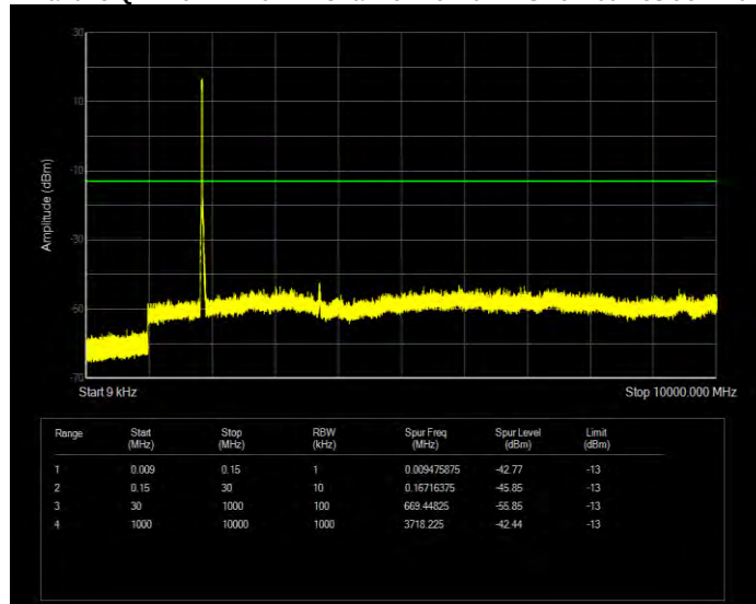
Band25 QAM16 BW=20MHz Channel=26140 RB Size=100 Position=#0
