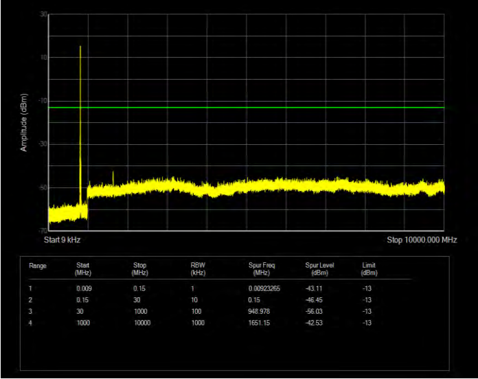
Band26(824-849) QAM16 BW=5MHz Channel=26815 RB Size=25 Position=#0
