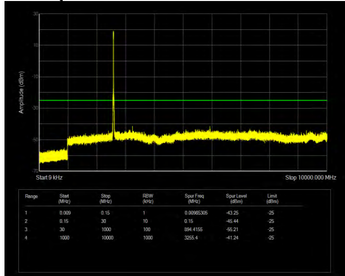
Band38 QAM16 BW=15MHz Channel=38175 RB Size=75 Position=#0
