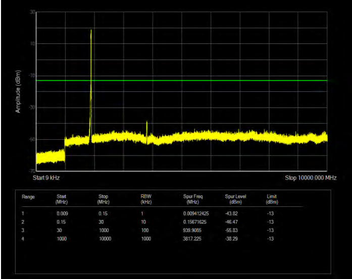
Band25 QAM16 BW=3MHz Channel=26055 RB Size=15 Position=#0
