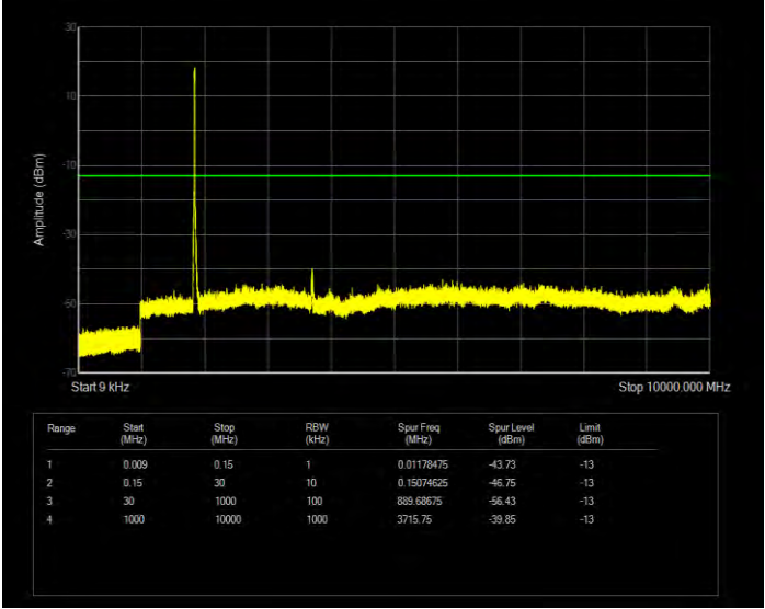
Band25 QAM16 BW=15MHz Channel=26115 RB Size=75 Position=#0
