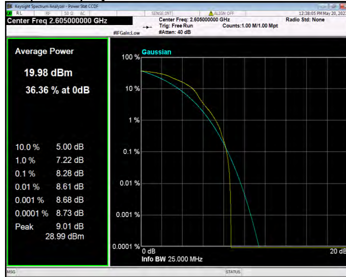
Band41(2535-2675) 16QAM BW=15MHz Channel=40740 RB Size=1 Position=#0
