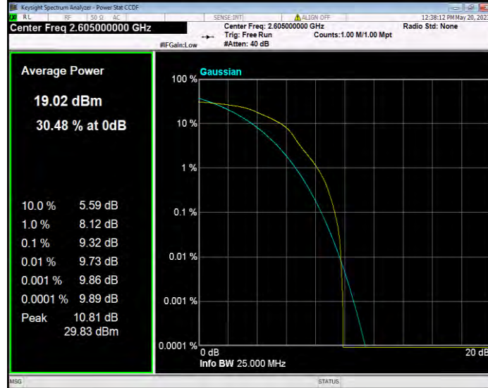
Band41(2535-2675) 16QAM BW=20MHz Channel=40740 RB Size=1 Position=#0
