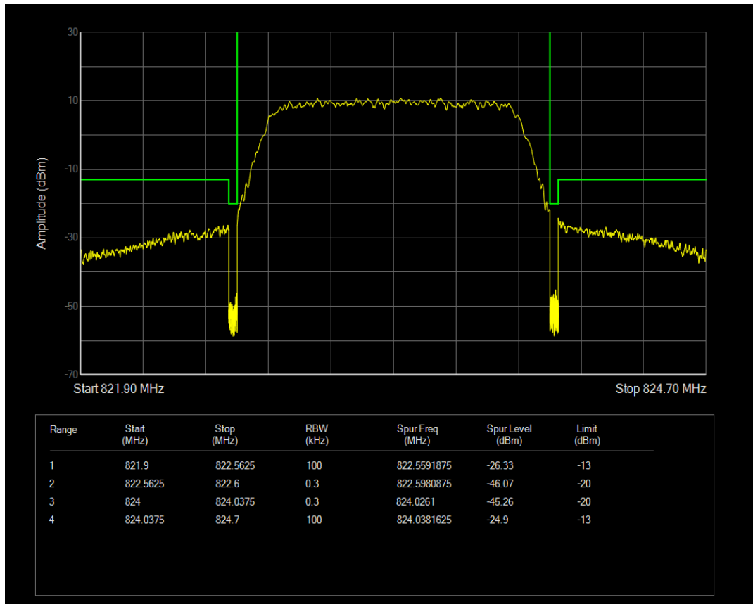
Band26(820-824) QPSK BW=3MHz Channel=26765 RB Size=15 Position=#0
