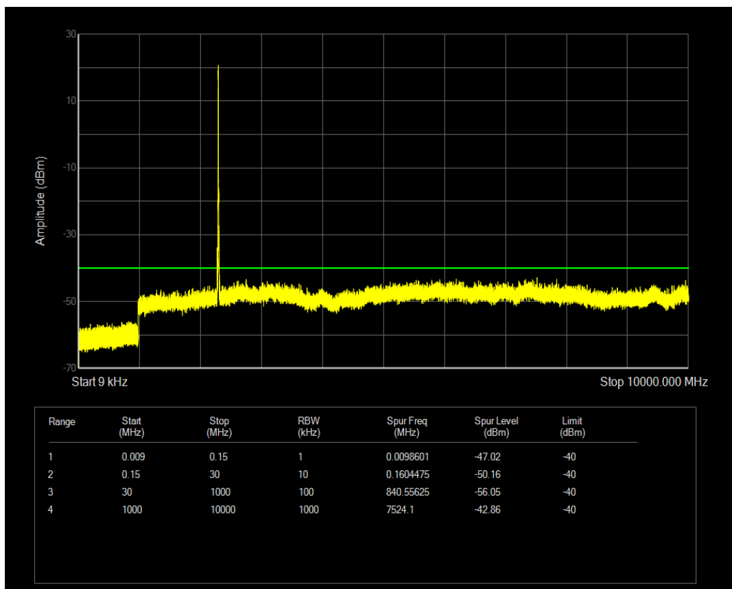
Band40(2305-2315) QPSK BW=5MHz Channel=38775 RB Size=25 Position=#0
