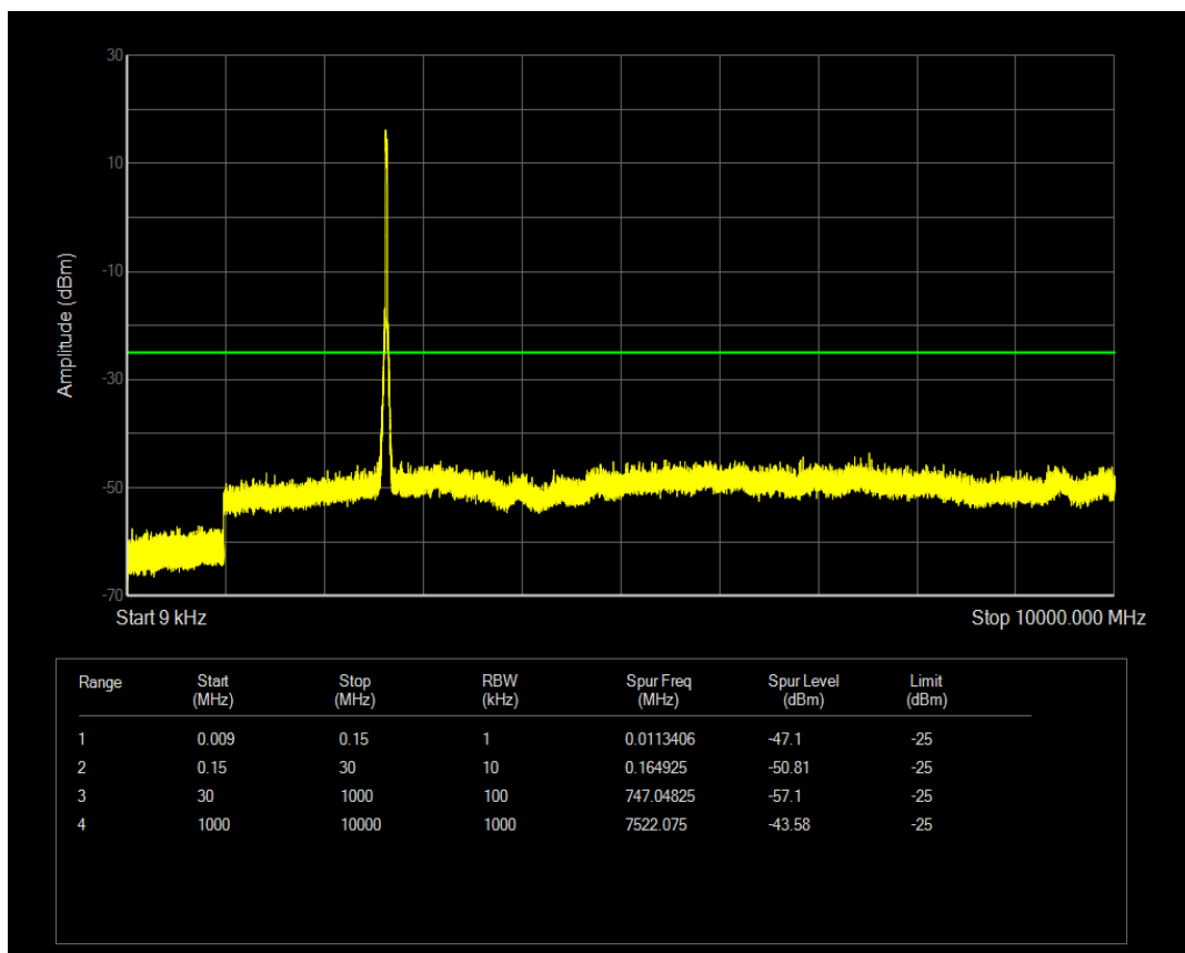
Band41(2555-2655) 16QAM BW=5MHz Channel=40265 RB Size=25 Position=#0
