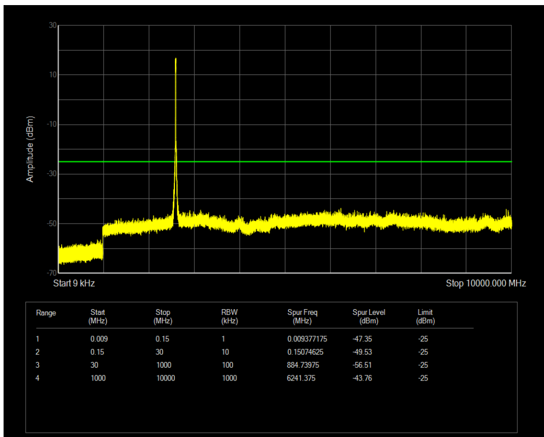
Band41(2555-2655) 16QAM BW=15MHz Channel=41165 RB Size=75 Position=#0
