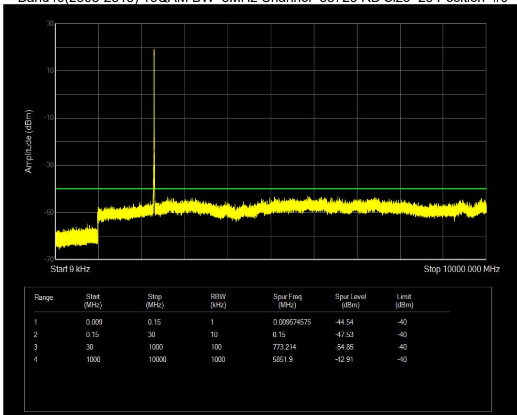
Band40(2305-2315) 16QAM BW=5MHz Channel=38750 RB Size=25 Position=#0
