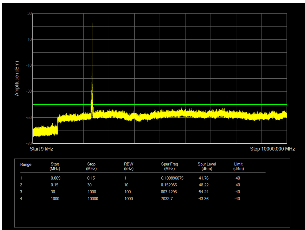
Band40(2350-2360) QPSK BW=5MHz Channel=39200 RB Size=25 Position=#0
