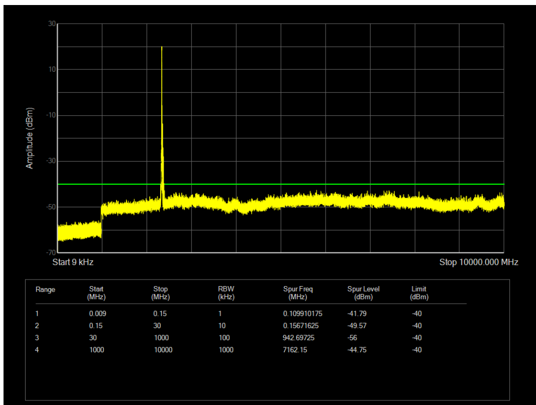
Band40(2350-2360) 16QAM BW=5MHz Channel=39200 RB Size=25 Position=#0
