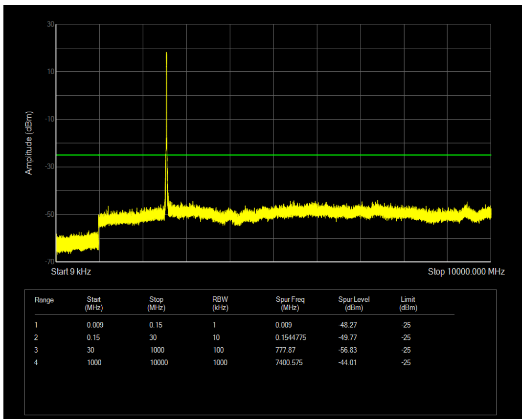
Band41(2555-2655) 16QAM BW=10MHz Channel=40740 RB Size=50 Position=#0
