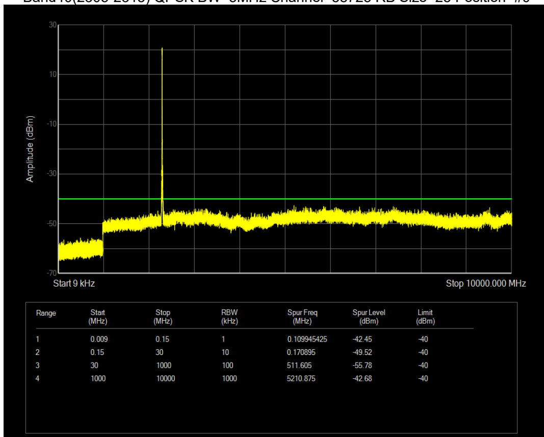
Band40(2305-2315) QPSK BW=5MHz Channel=38750 RB Size=25 Position=#0
