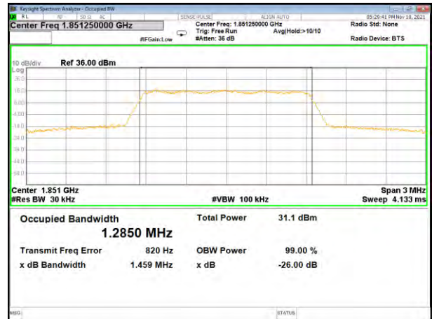
EVDO CDMA Lower6BW and 99%
