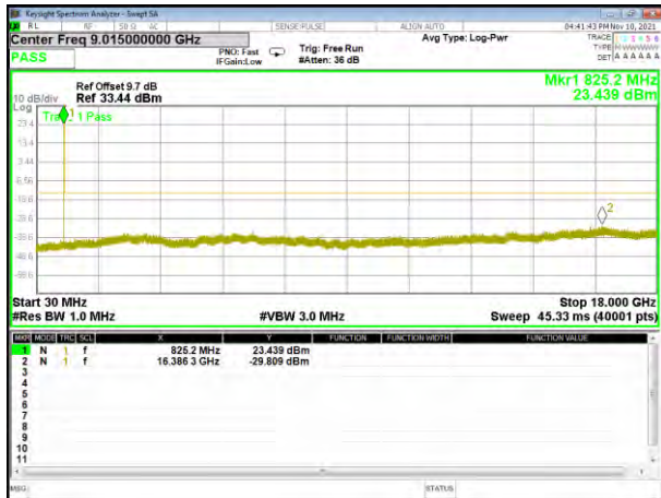
CDMA BC0 Low Conducted Spurious
