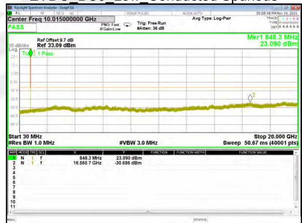
EVDO BC0 High Conducted Spurious
