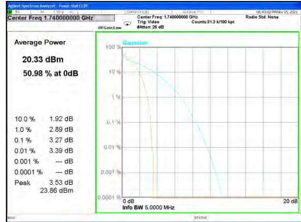
HSUPA Band 4_Middle
