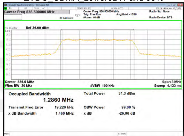
EVDO CDMA Middle6BW and 99%
