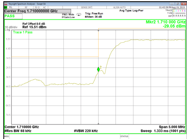
B4 HSDPA Lower Band edge
