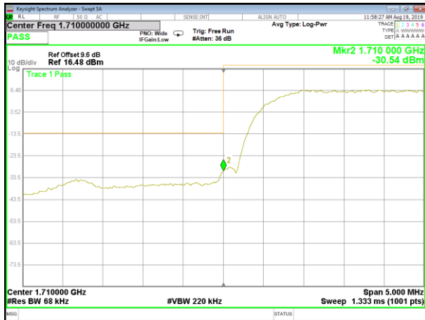
B4 WCDMA Lower Band edge
