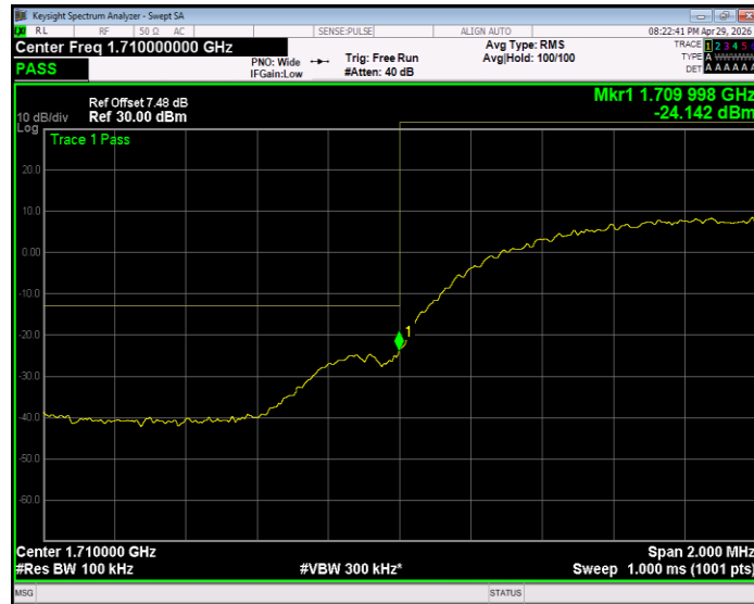
WCDMA Band4 Channel=1513
