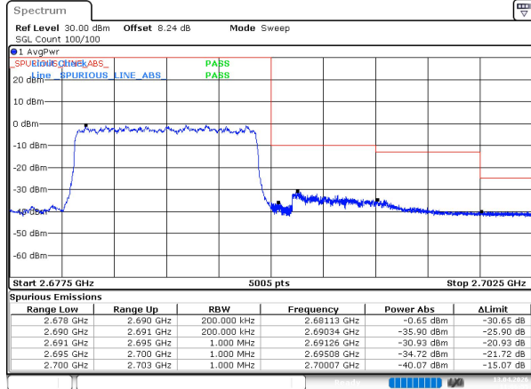
n41 SCS=30kHz DFT_64QAM BW=10MHz HighChannel=537000 RB=24@0
