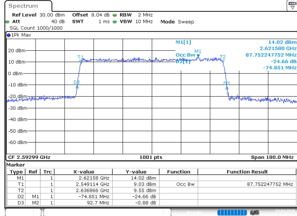
n41 SCS=30kHz CP_64QAM BW=90MHz Channel=518598 RB=245@0
