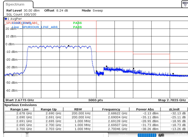
n41 SCS=30kHz DFT_256QAM BW=10MHz HighChannel=537000 RB=1@23
