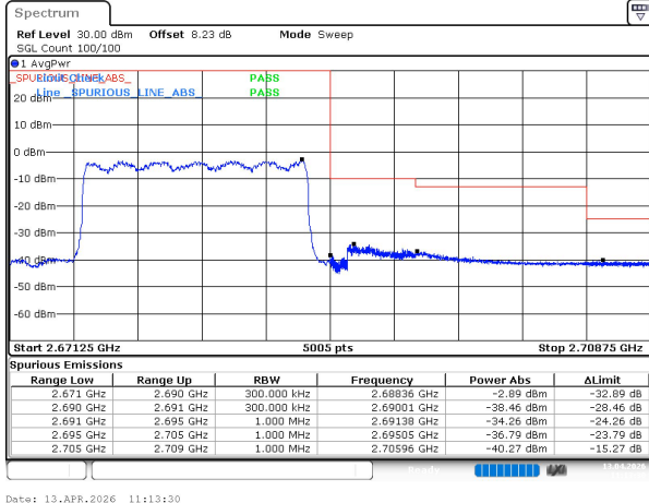
n41 SCS=30kHz DFT_256QAM BW=15MHz HighChannel=536496 RB=36@0
