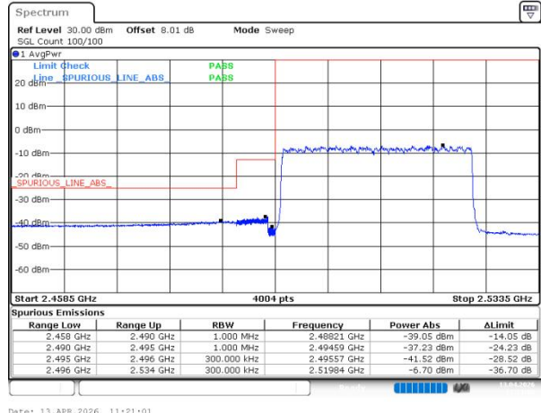
n41 SCS=30kHz DFT_256QAM BW=30MHz LowChannel=502200 RB=75@0
