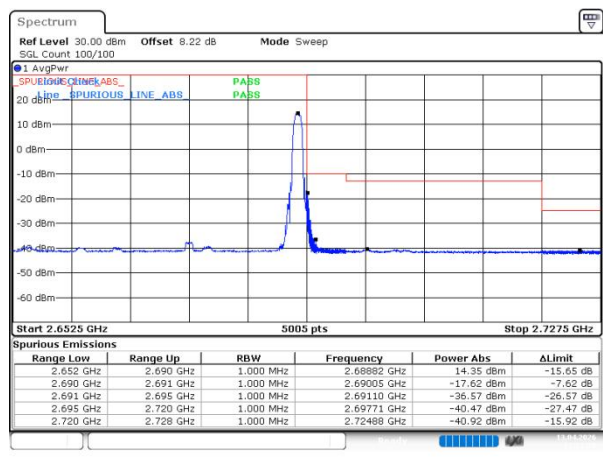
n41 SCS=30kHz DFT_BPSK BW=30MHz HighChannel=534996 RB=1@77
