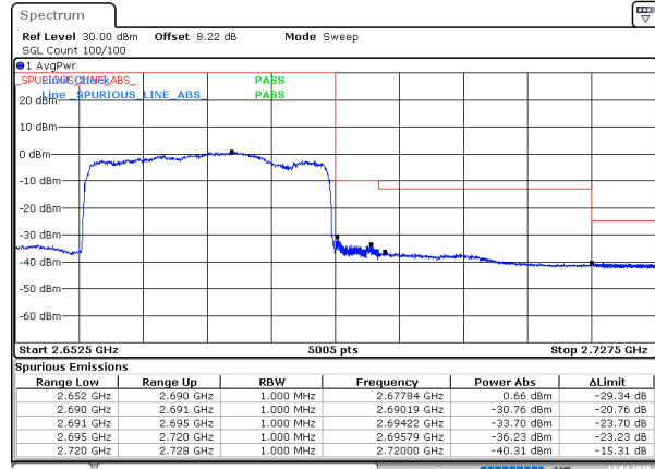
n41 SCS=30kHz DFT_256QAM BW=30MHz HighChannel=534996 RB=1@77
