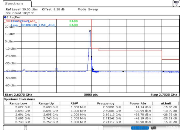
n41 SCS=30kHz DFT_64QAM BW=50MHz HighChannel=532998 RB=1@132
