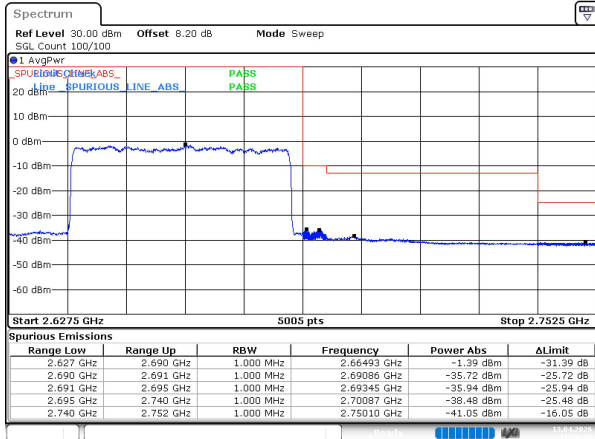
n41 SCS=30kHz DFT_16QAM BW=50MHz HighChannel=532998 RB=128@0
