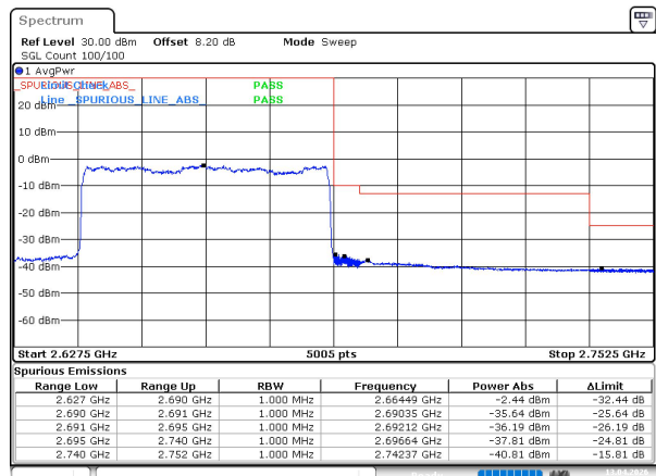
n41 SCS=30kHz DFT_256QAM BW=50MHz HighChannel=532998 RB=1@132
