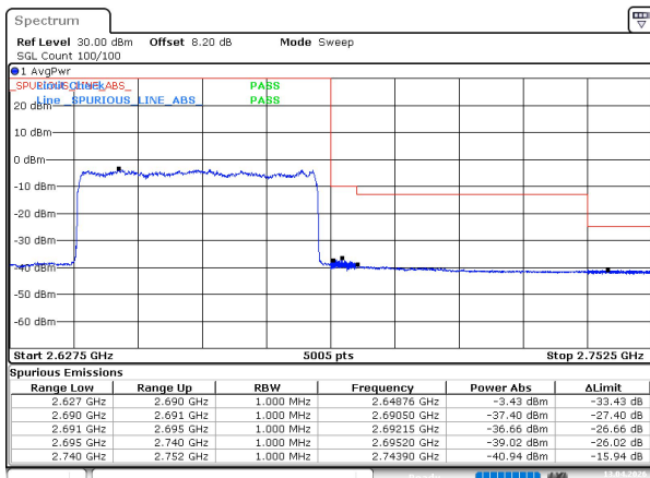
n41 SCS=30kHz DFT_64QAM BW=50MHz HighChannel=532998 RB=128@0
