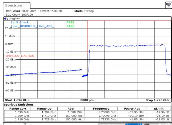
n66 SCS=15kHz DFT_64QAM BW=15MHz LowChannel=343500 RB=75@0
