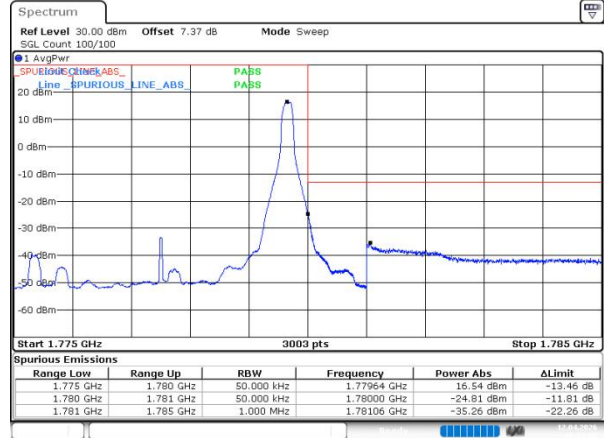
n66 SCS=15kHz DFT_QPSK BW=5MHz HighChannel=355500 RB=1@24
