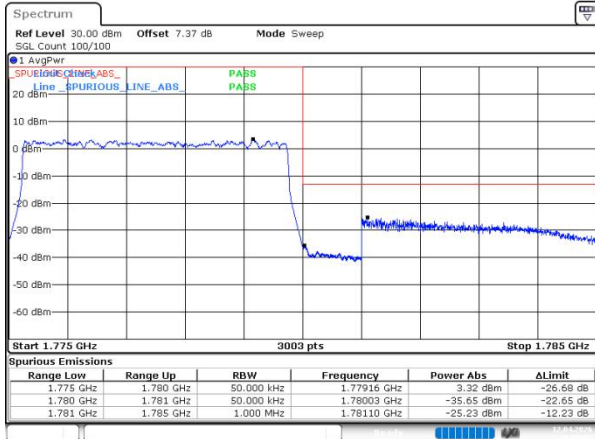
n66 SCS=15kHz DFT_BPSK BW=5MHz HighChannel=355500 RB=25@0
