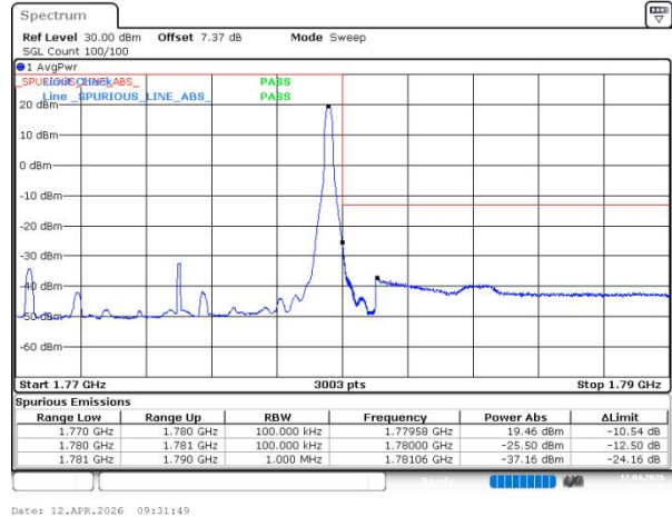
n66 SCS=15kHz DFT_BPSK BW=10MHz HighChannel=355000 RB=1@51
