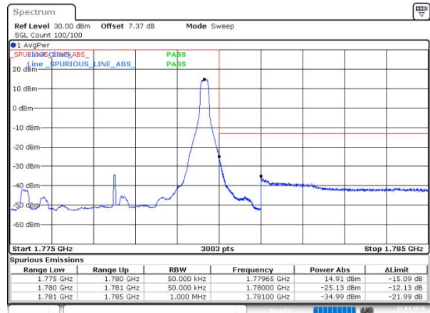
n66 SCS=15kHz DFT_16QAM BW=5MHz HighChannel=355500 RB=1@24
